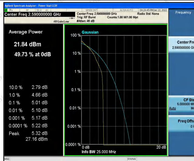
Band41-15MHz-QPSK-40590-75RB#0
