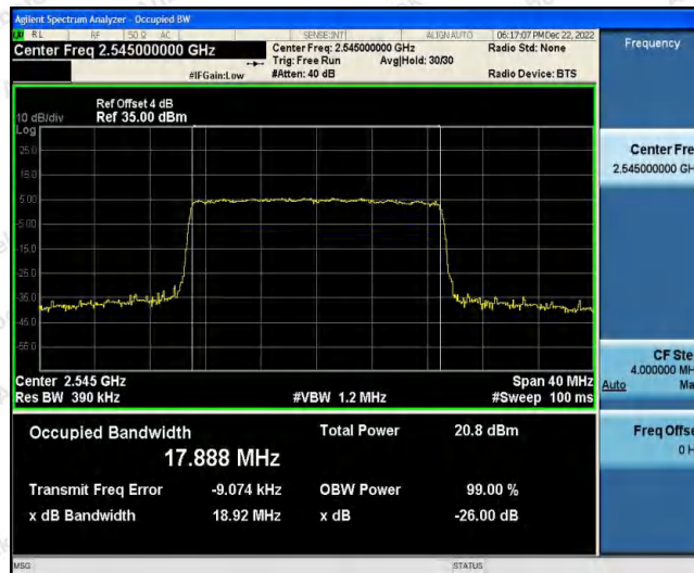
Band41-20MHz-16QAM-40590-100RB#0
