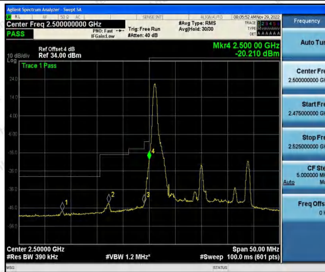
Band7-20MHz-QPSK-20850-1RB#99
