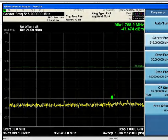
Band2-1.4MHz-QPSK-18900-1RB#0-Range1:30~1000MHz
