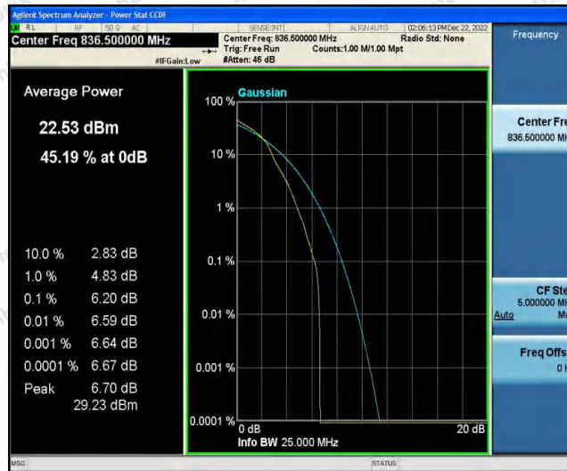
Band26-1.4MHz-16QAM-26915-6RB#0
