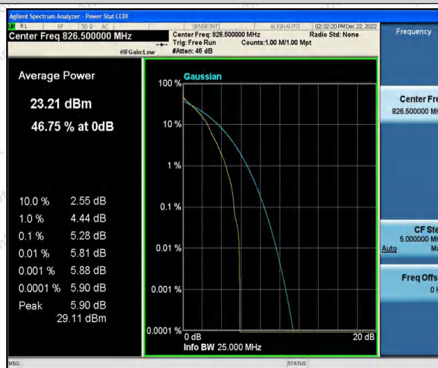
Band26-5MHz-QPSK-26815-25RB#0
