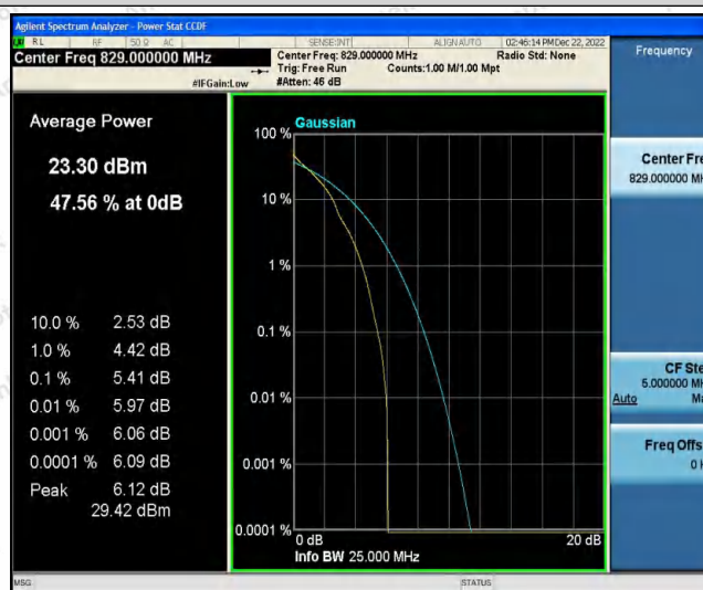
Band26-10MHz-QPSK-26840-50RB#0
