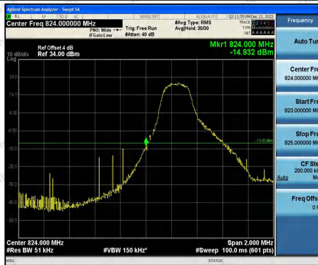
Band26-3MHz-QPSK-26805-1RB#14
