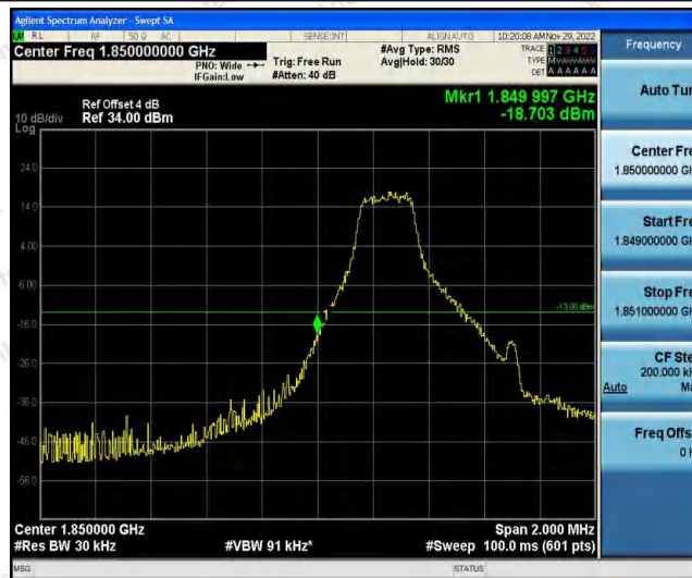
Band25-1.4MHz-16QAM-26047-1RB#5
