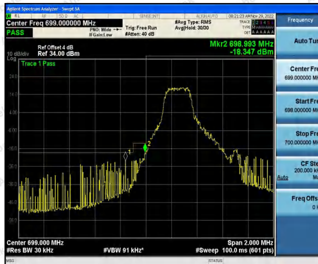
Band12-1.4MHz-16QAM-23017-1RB#5
