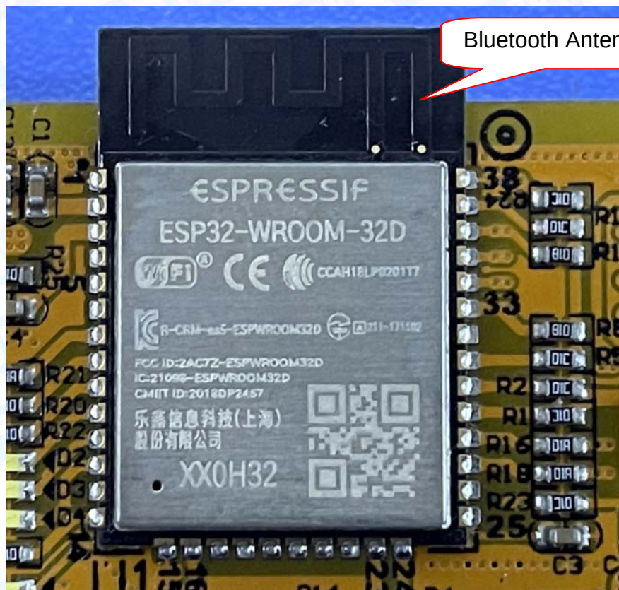
Photo 12 Appearance of PCB
