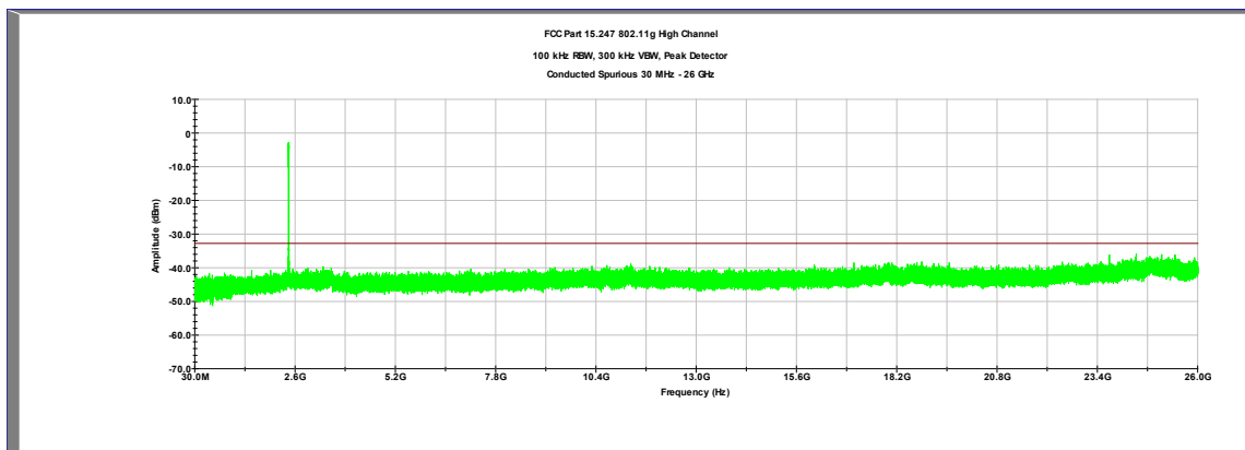
Plot 4.6 Tx @ 2462MHz 802.11g
