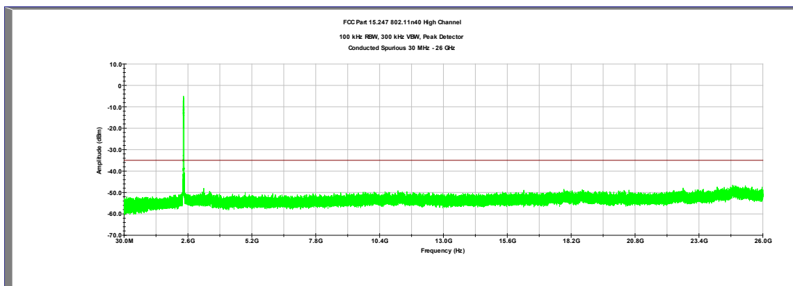
Plot 4.12 Tx @ 2452MHz 802.11n 40MHz
