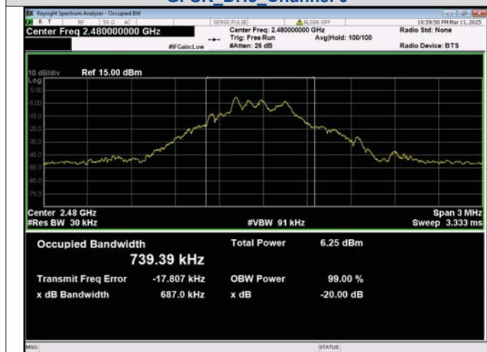
GFSK_DH5_Channel 78
