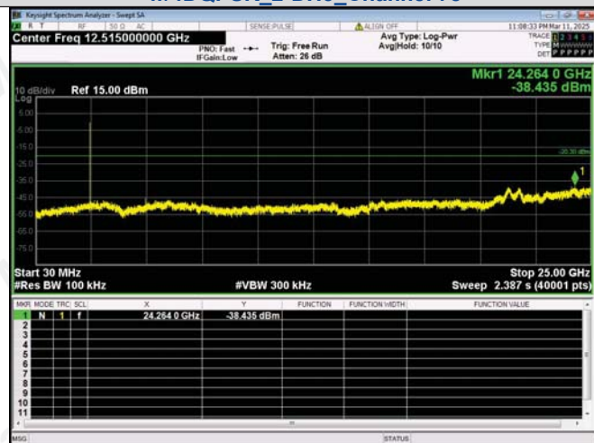
30.0 MHz - 25000.0 MHz \pi/4 DQPSK_2-DH5_Channel 78
