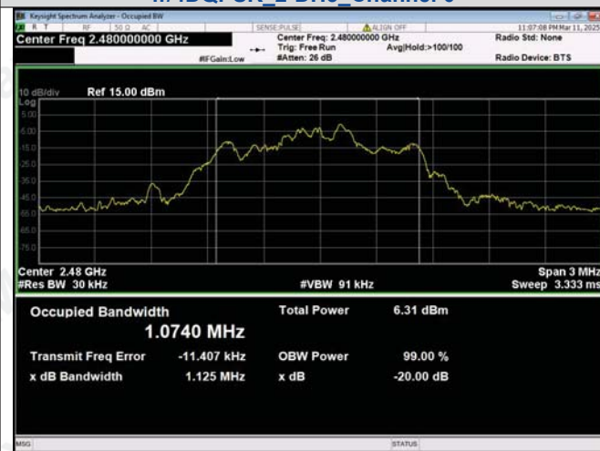
\pi/4 DQPSK_2-DH5_Channel 78
