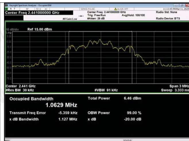
8DPSK_3-DH5_Channel 39
