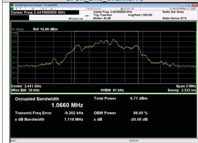
\pi/4 DQPSK_2-DH5_Channel 39
