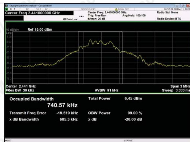
GFSK_DH5_Channel 39
