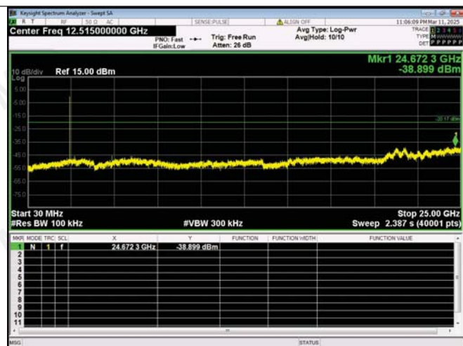
30.0 MHz - 25000.0 MHz \pi/4 DQPSK_2-DH5_Channel 39
