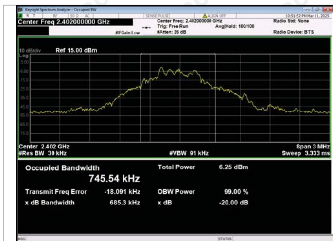
GFSK_DH5_Channel 0
