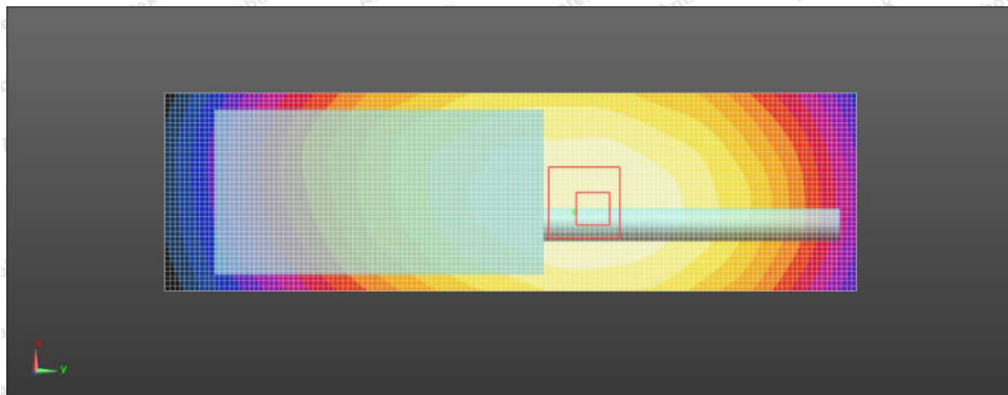
Figure 1: PMR_FM12.5KHz_Face held_25mm
