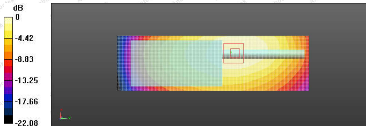
Figure 2: PMR_FM12.5KHz_Body Worn_0mm
