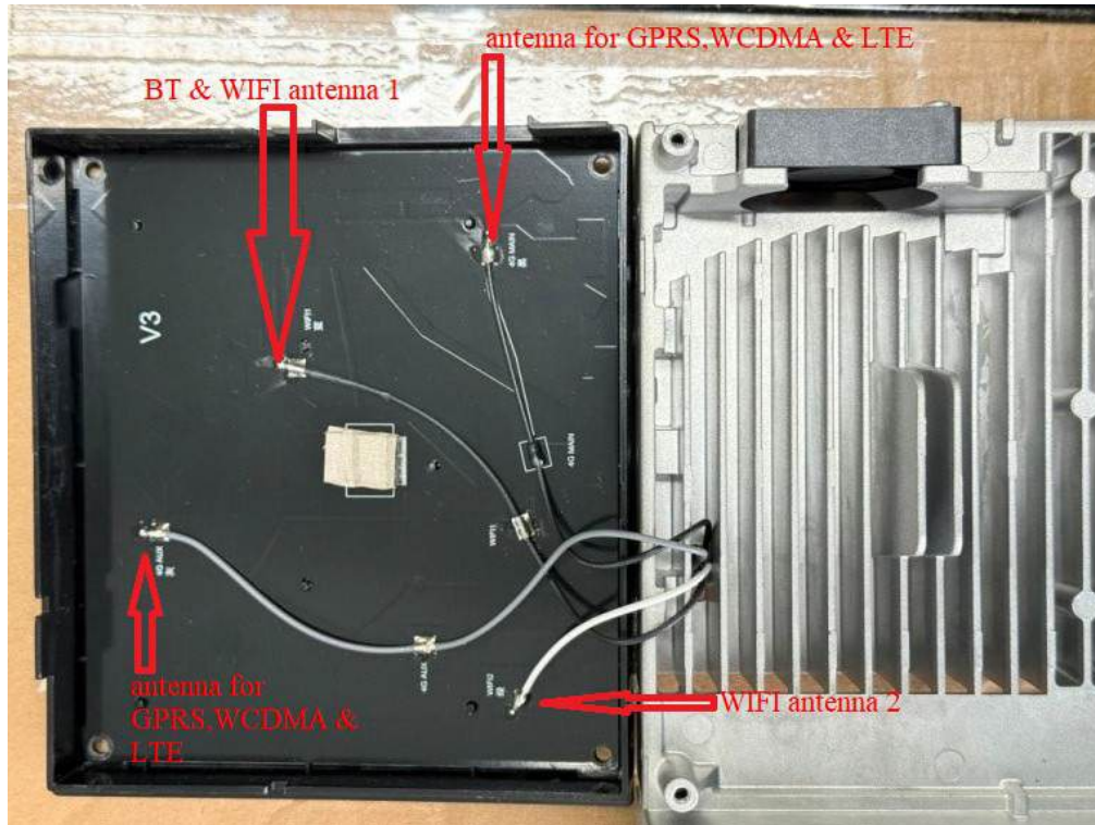
Photo 19: Internal View for Antenna
