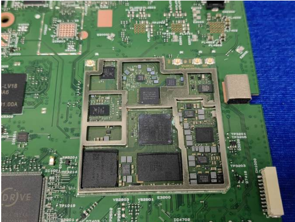
Photo 19: Internal View for PCB
