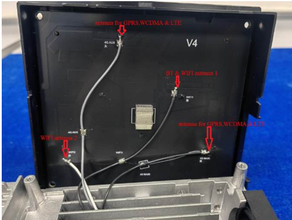
Photo 31: Internal View for Antenna
