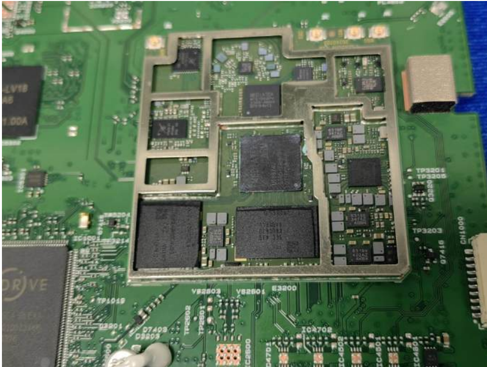
Photo 21: Internal View for PCB
