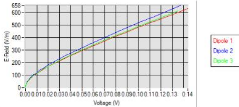
Calibration curves
