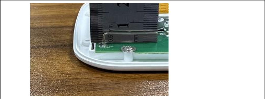
Antenna Bottom View [With Ruler]
