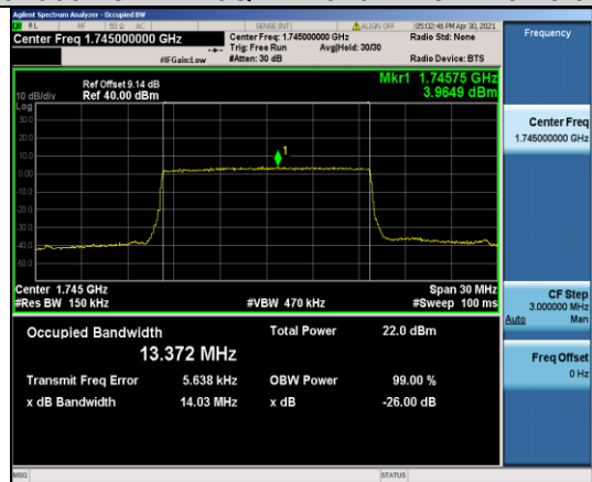
Band66-15MHz-16QAM-132322-75RB#0-13.372
