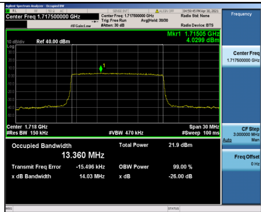
Band66-15MHz-16QAM-132047-75RB#0-13.360
