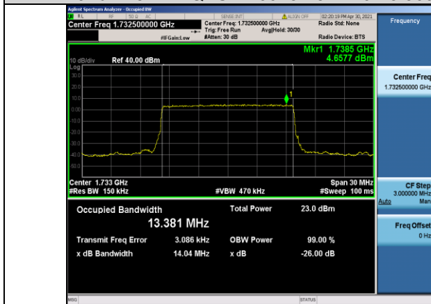
Band4-15MHz-QPSK-20175-75RB#0-13.381
