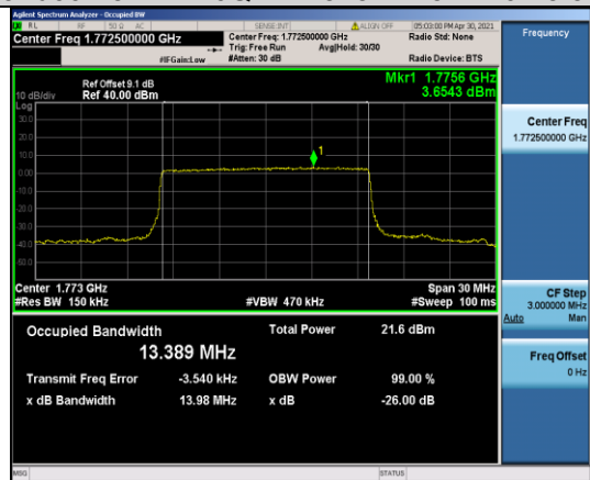
Band66-15MHz-16QAM-132597-75RB#0-13.389
