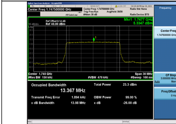
Band4-15MHz-QPSK-20325-75RB#0-13.367
