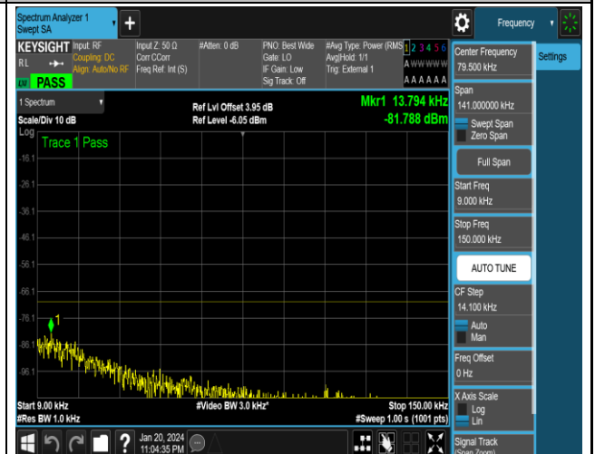
NTNV_N48_PC3_30_40_H_TID18_NS_01_0.009_0.15_#1
