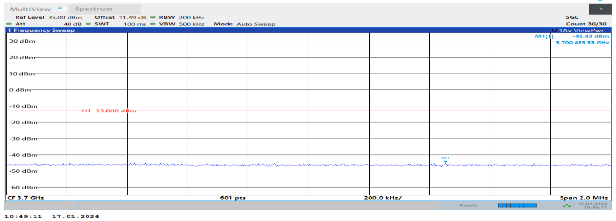
Band48-10MHz-16QAM-56690-1RB#49
