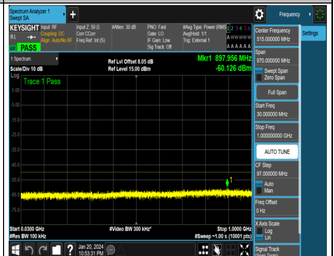
NTNV_N48_PC3_30_40_H_TID16_NS_01_30_1000_#1
