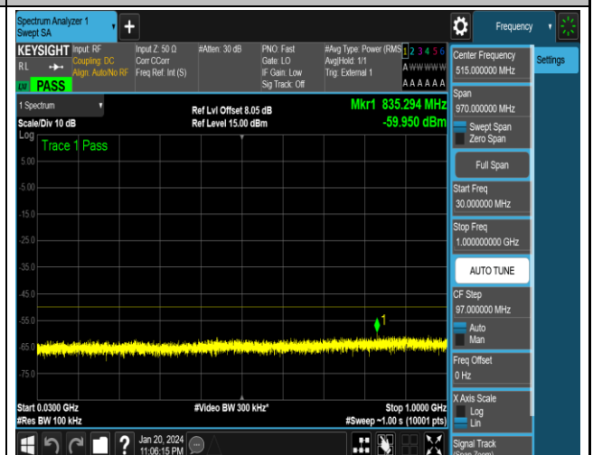
NTNV_N48_PC3_30_40_H_TID18_NS_01_30_1000_#1
