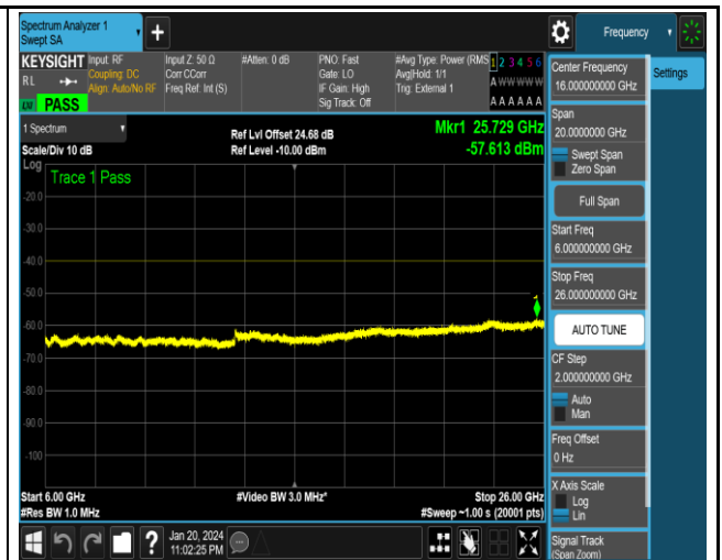
NTNV_N48_PC3_30_40_H_TID17_NS_01_6000_26000_#1
