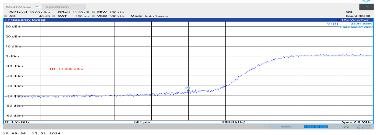
Band48-10MHz-16QAM-56690-1RB#0
