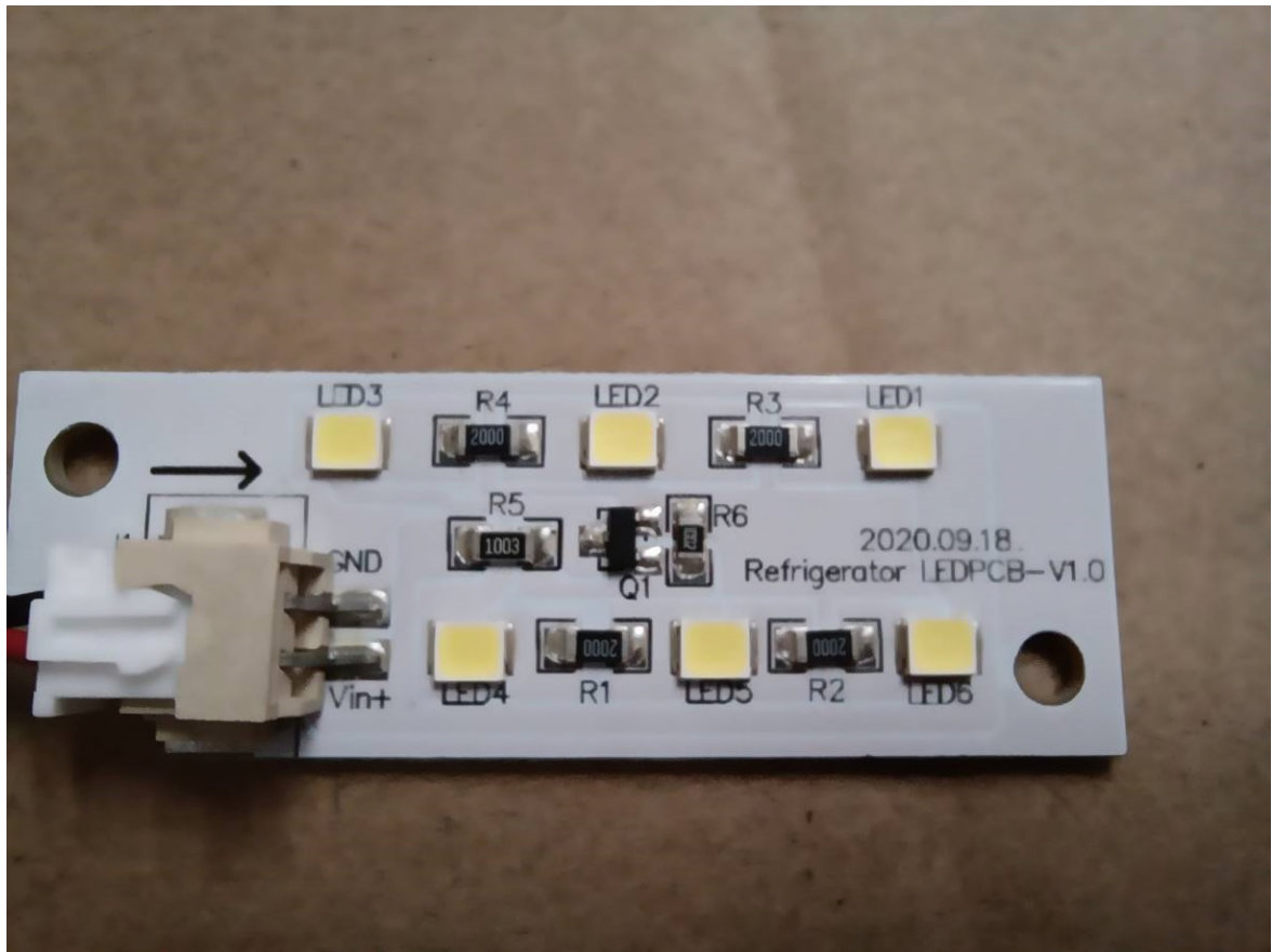
Picture 7 LED board
