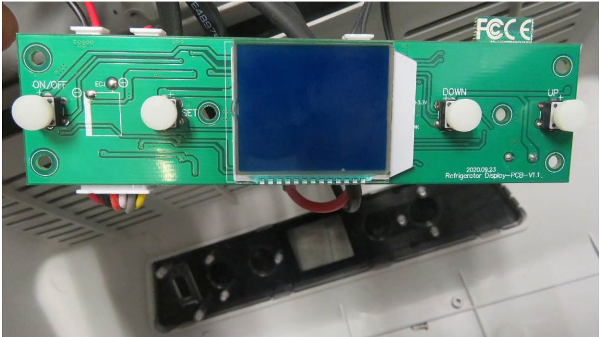
Picture 13 Control display board
