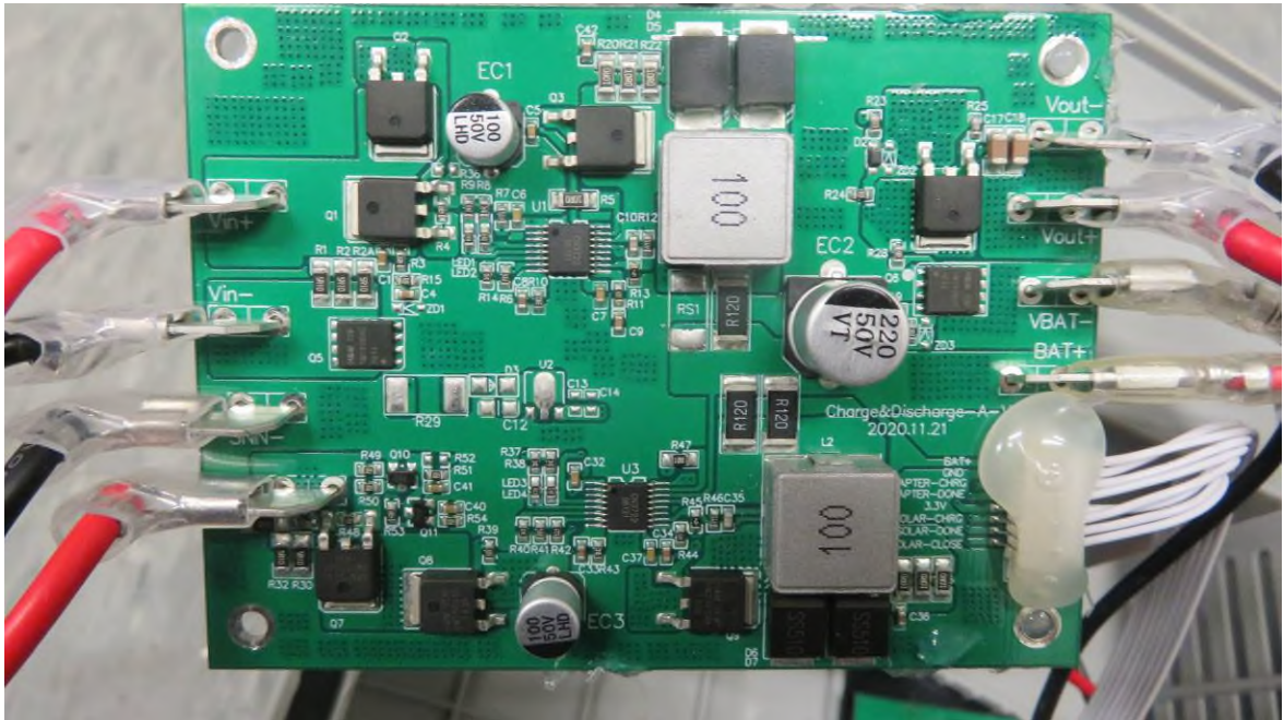
Picture 11 Charge board (for FCR-15, FCR-30, FCR-40 and FCR-50)
