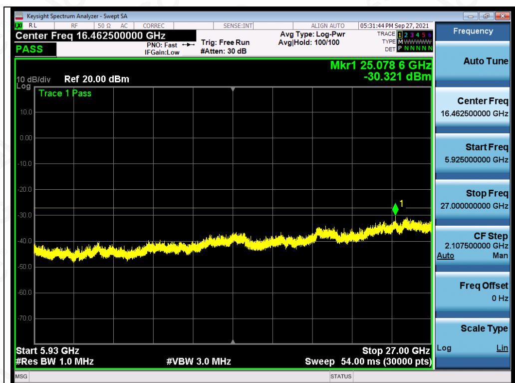
Test Graph 802.11a ANT1 5825 6Mbps Frequency Band4
