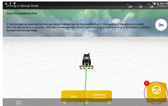
Figure 3.2.36 Starting auto steering driving after turning around
