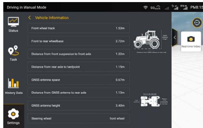
Figure 3.2.20 Vehicle information
