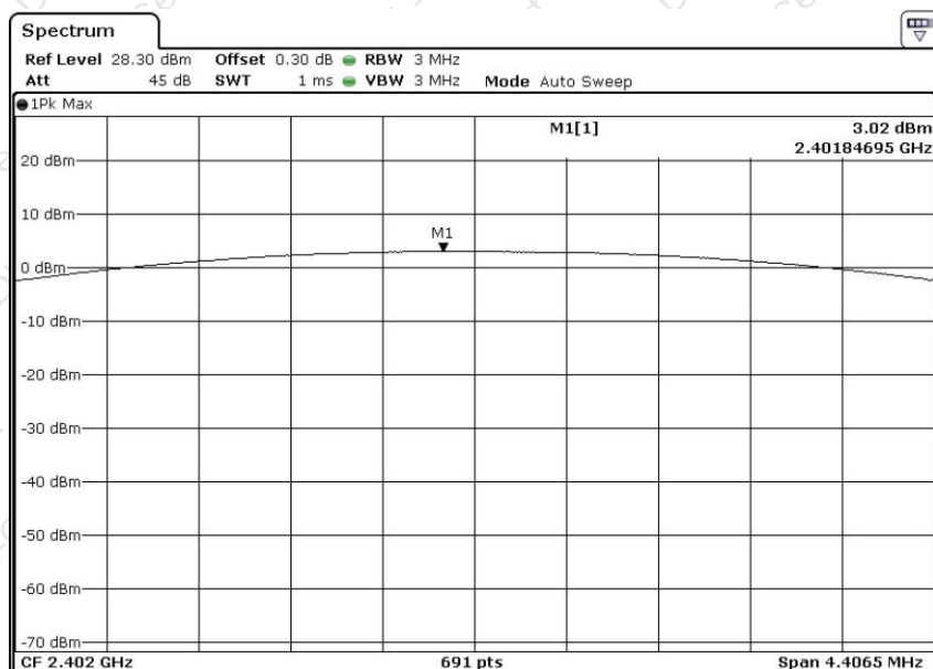
GFSK - 1-DH1 Test plots Low Channel
