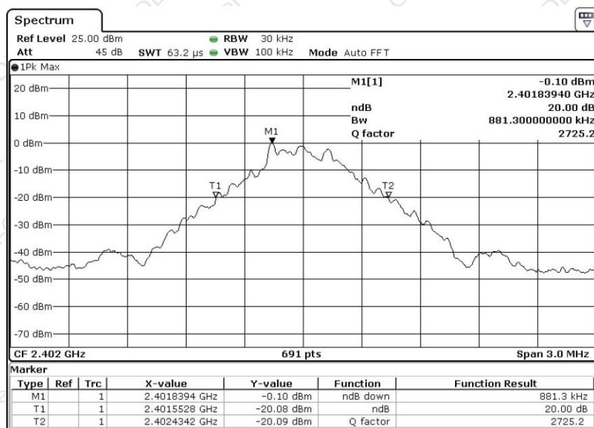
GFSK - 1-DH1 Test plots
