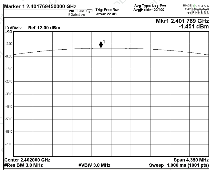
GFSK - 1-DH1 Test plots Low Channel
