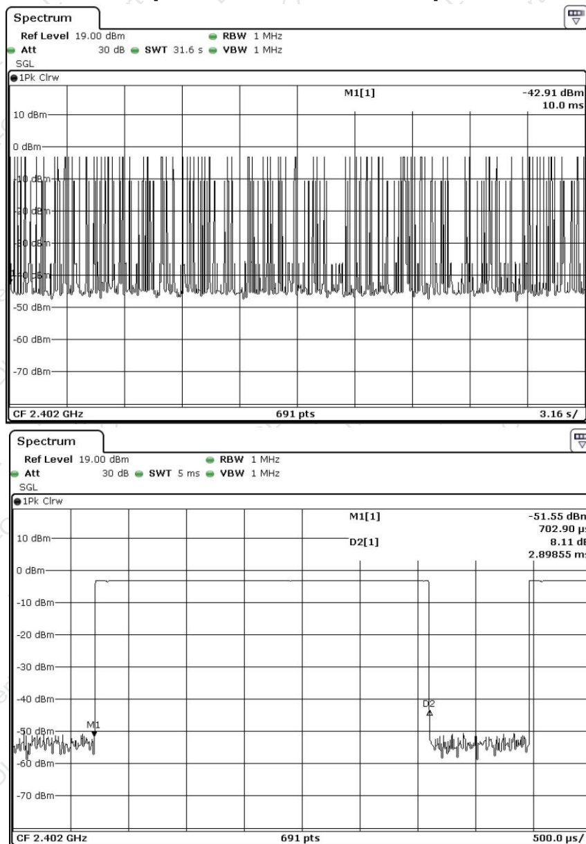
DH5 Measurement Data: Fig. A [Pulse duration of Lowest Channel]
