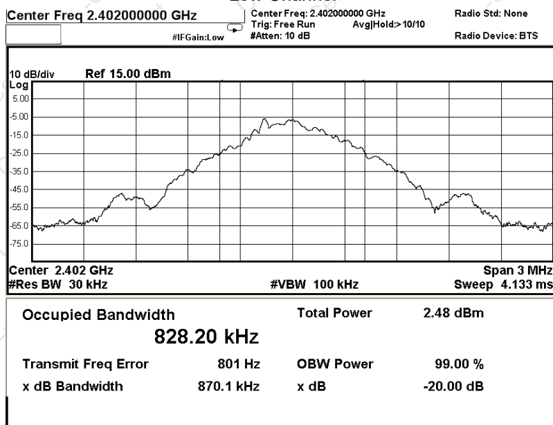
GFSK - 1-DH1 Test plots
