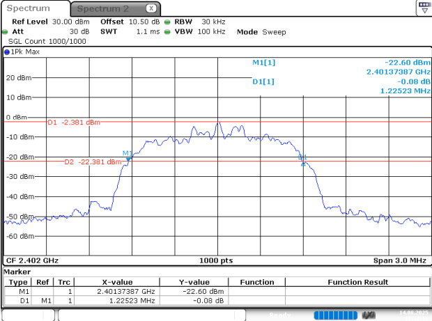
2EDR_DH1_Low
