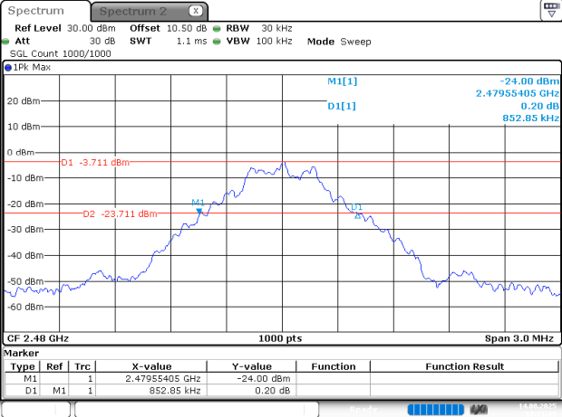
BDR_DH1_High
