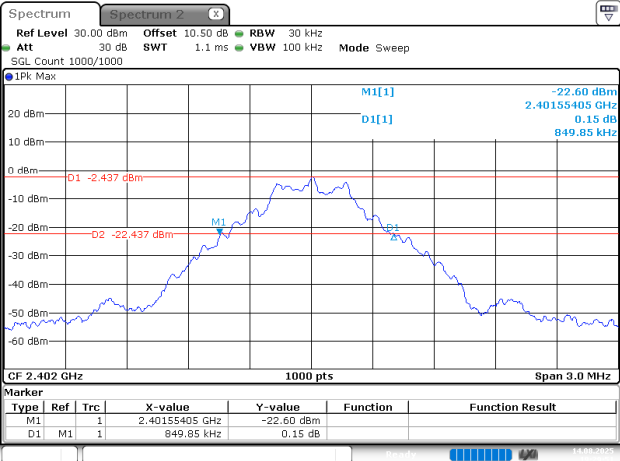
BDR_DH1_Low
