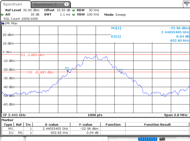
BDR_DH1_Middle
