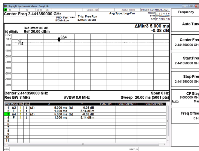
Duty Cycle_2441.35MHz
