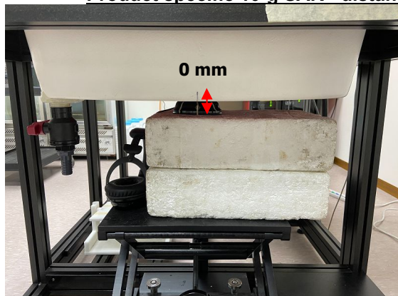
Photograph 3. Product specific 10-g SAR, Front Surface, 0mm
