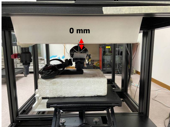
Photograph 9. Product specific 10-g SAR, Right Edge, 0mm
