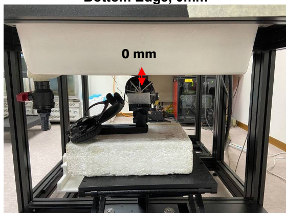
Photograph 7. Product specific 10-g SAR, Right Up Edge, 0mm
