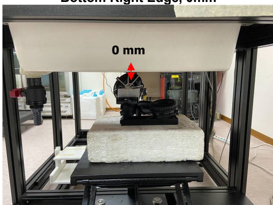
Photograph 13. Product specific 10-g SAR, Left Up Edge, 0mm
