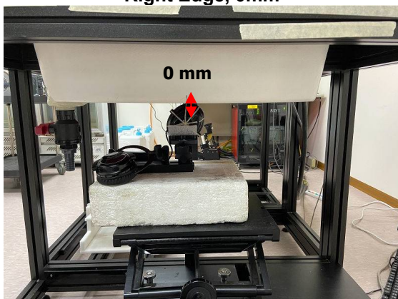
Photograph 11. Product specific 10-g SAR, Bottom Right Edge, 0mm
