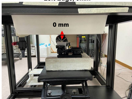
Photograph 17. Product specific 10-g SAR, Bottom Left Edge, 0mm
