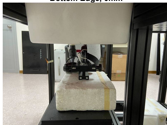
Photograph 8. Product specific 10-g SAR, Right Up Edge, 0mm
