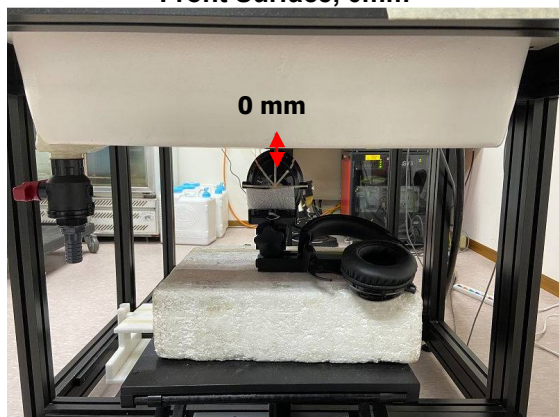
Photograph 5. Product specific 10-g SAR, Bottom Edge, 0mm
