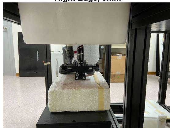
Photograph 12. Product specific 10-g SAR, Bottom Right Edge, 0mm
