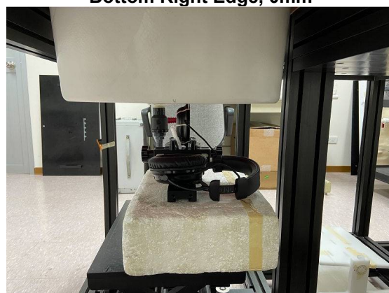
Photograph 14. Product specific 10-g SAR, Left Up Edge, 0mm
