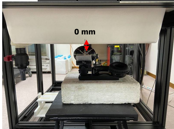
Photograph 15. Product specific 10-g SAR, Left Edge, 0mm
