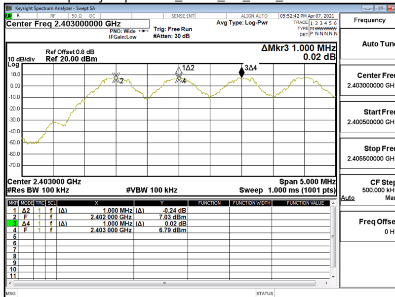
Frequency Separation _8DPSK_3M_DH5_CH0CH1CH2
