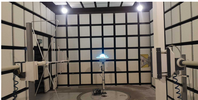
Photo 6: EUT at the anechoic chamber
