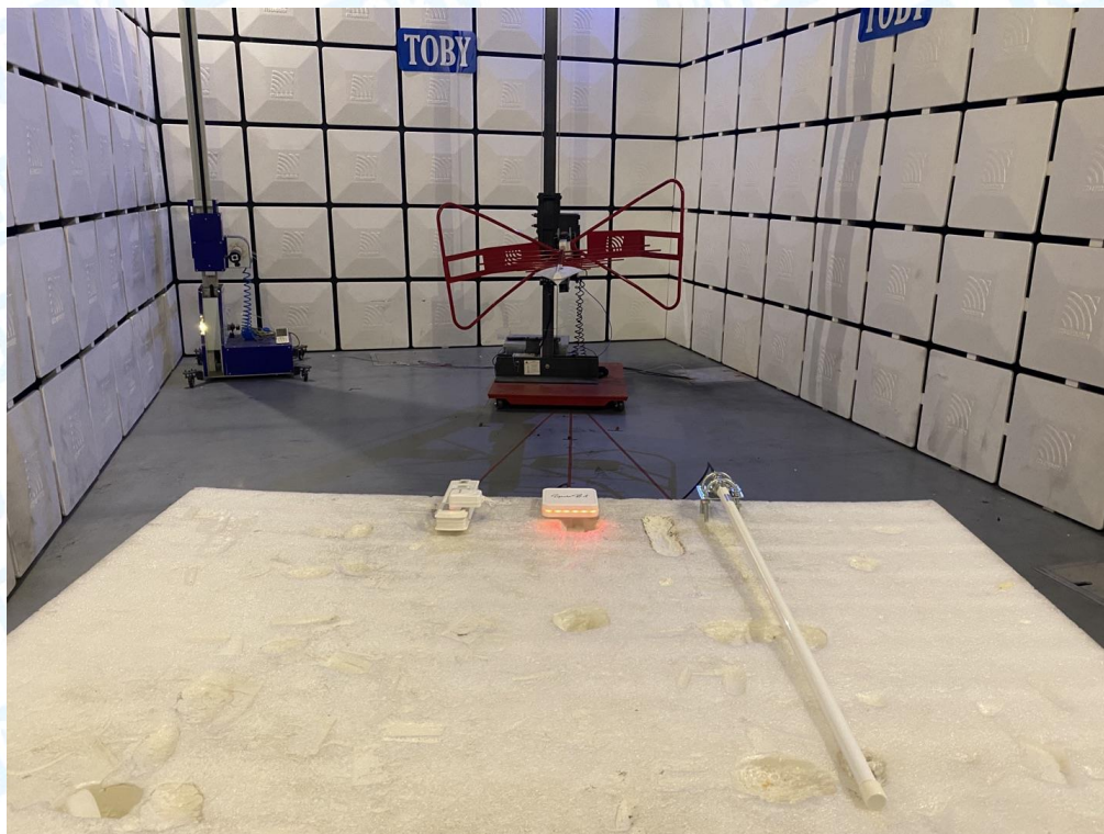
Photo of Setup for Radiated Emission (Below 1 GHz) for Ant 2
