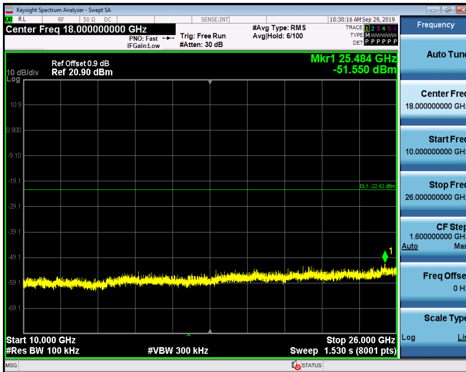
RF Conducted Spurious Emissions_11N20ISO_2462_Ant1
