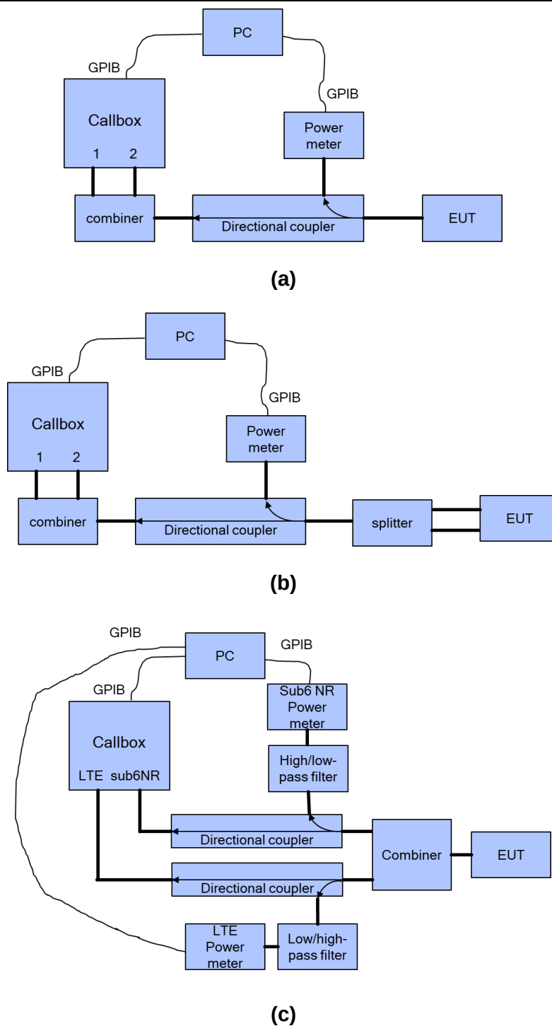
Figure 5-2 Conducted power measurement setup
