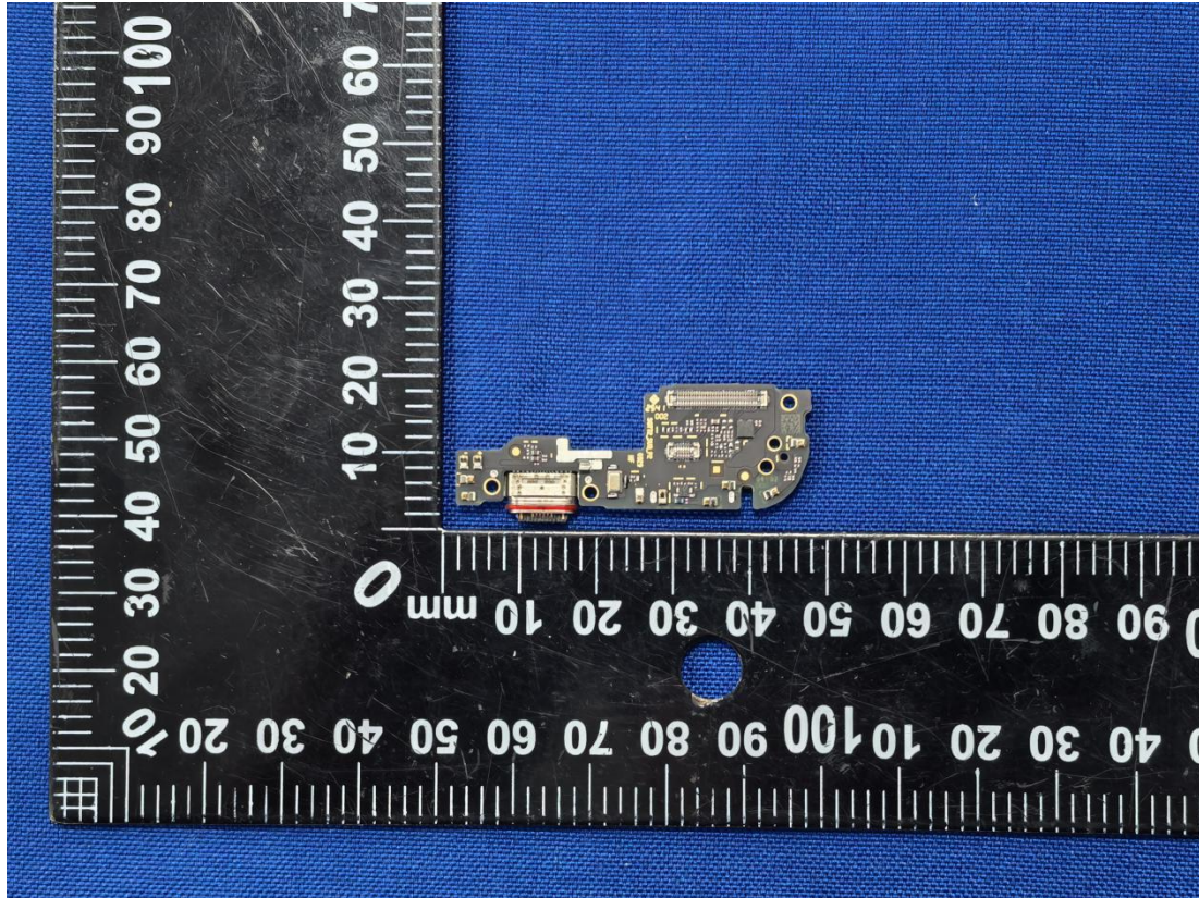
SECONDARY BOARD 1 TOP VIEW
