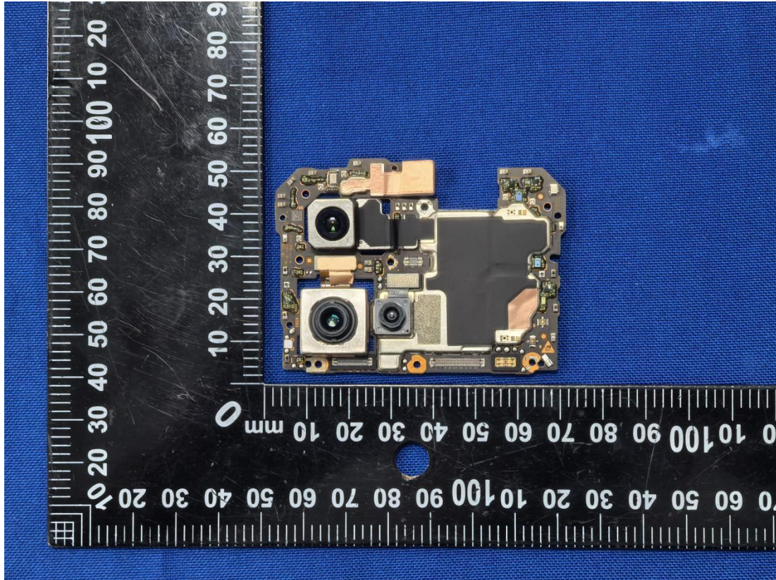
MAIN BOARD REAR VIEW (WITH SHIELDING)
