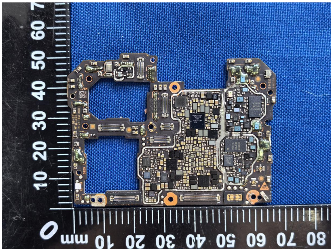
MAIN BOARD REAR VIEW (WITHOUT SHIELDING)
