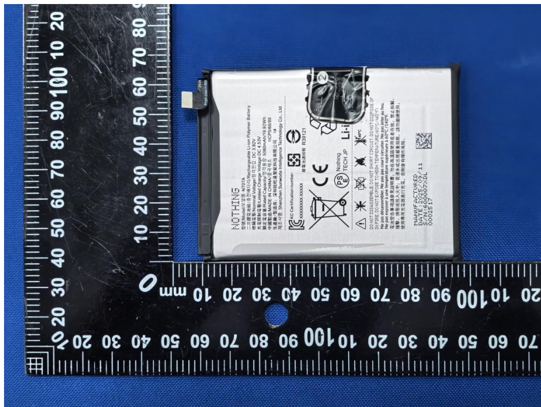
BATTERY 1 TOP VIEW
