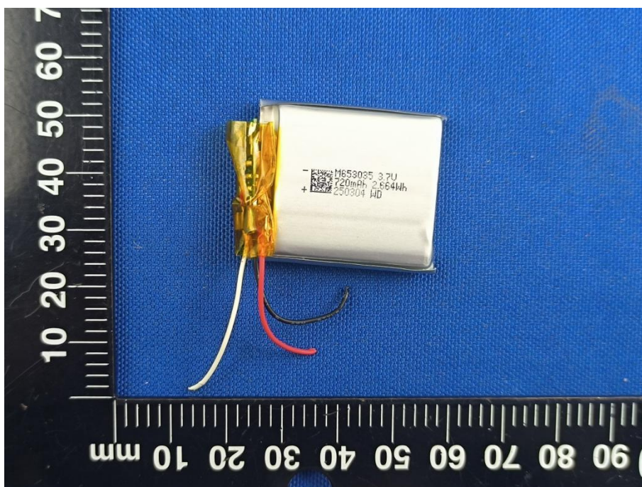
BATTERY 1 (FRONT)
