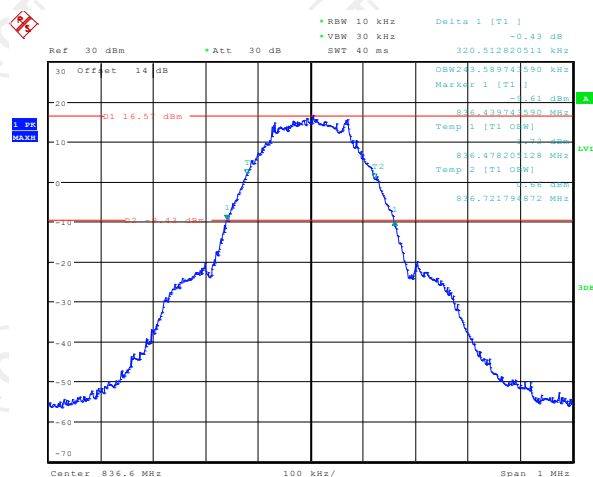
26dB&99% Occupied Bandwidth Plot on Channel 190
