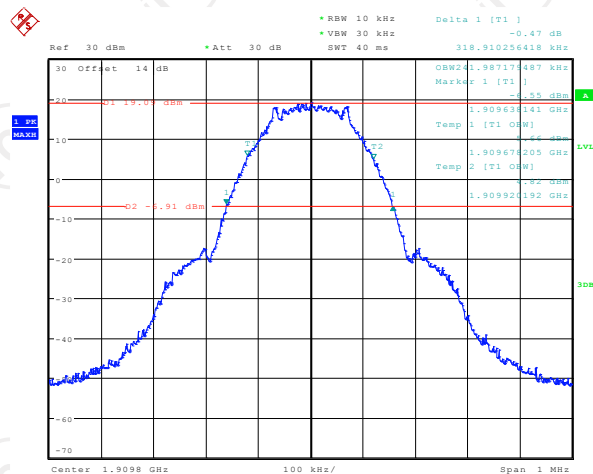
26dB&99% Occupied Bandwidth Plot on Channel 810
