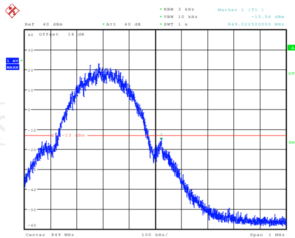
Higher Band Edge Plot on Channel 251
