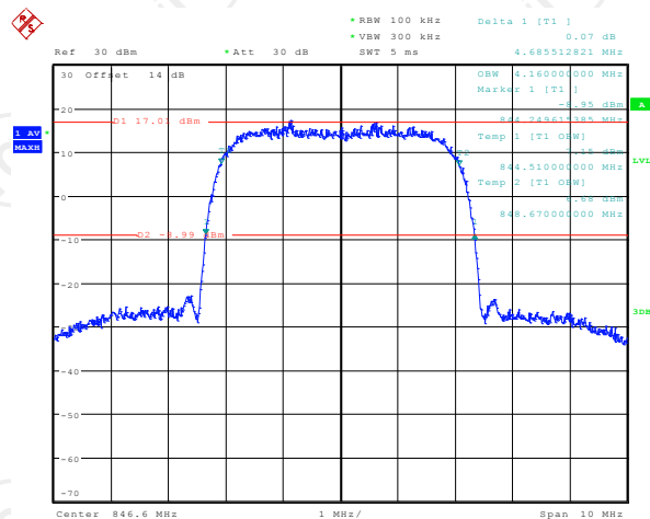
26dB&99% Occupied Bandwidth Plot on Channel 4233
