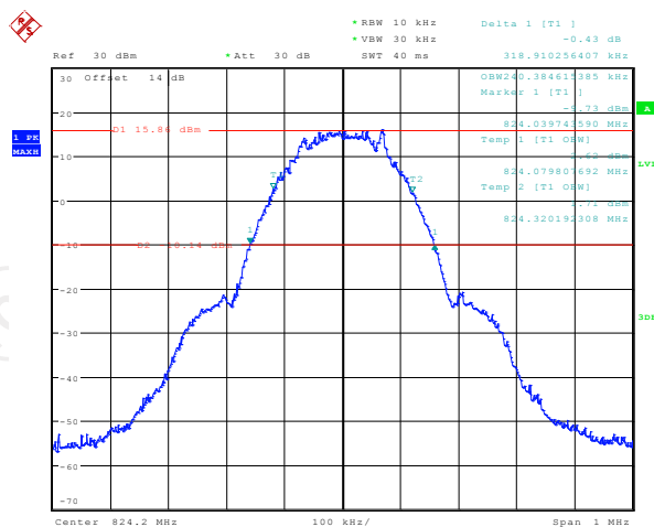
26dB&99% Occupied Bandwidth Plot on Channel 128
