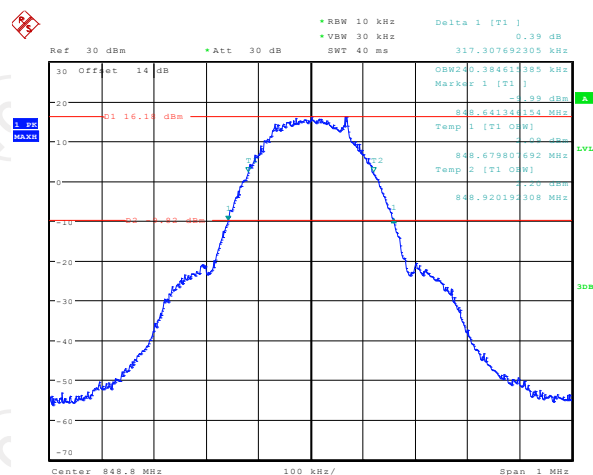
26dB&99% Occupied Bandwidth Plot on Channel 251
