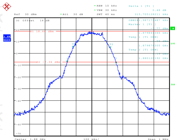
26dB&99% Occupied Bandwidth Plot on Channel 661
