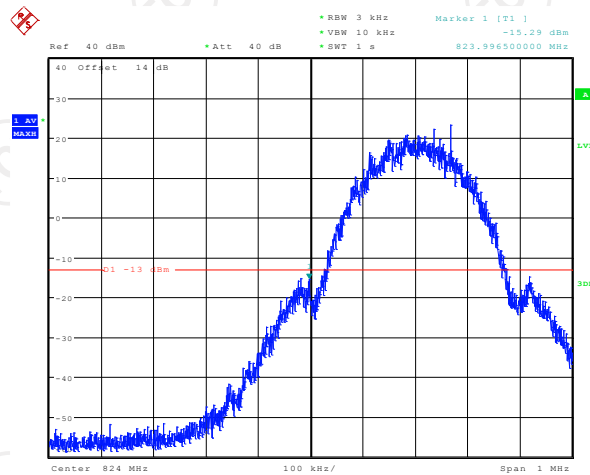
Lower Band Edge Plot on Channel 128
