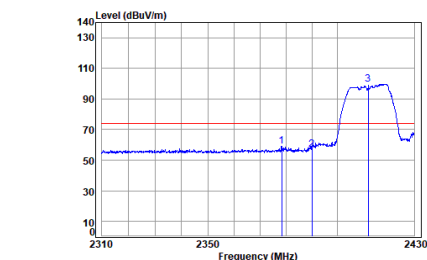
Antenna 2 11g_TX_CH_01_Horizontal-Peak
