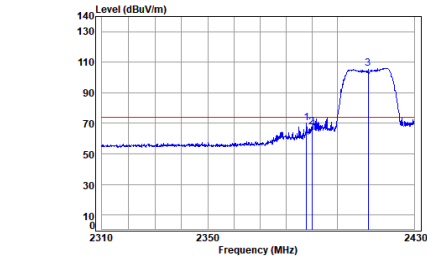
Antenna 2 11n_HT(20M)_TX_CH_01_Vertical-Peak
