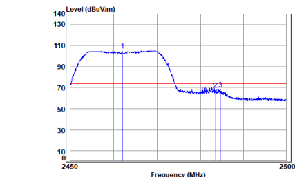
Antenna 1 11n_HT(20M)_TX_CH_11_Vertical-Peak
