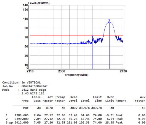
Antenna 1 11b_TX_CH_01_Vertical-Peak
