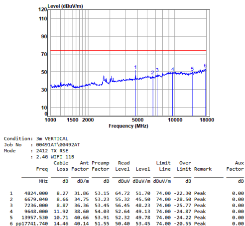
Antenna 1 11b_TX_CH_01_Vertical-Peak
