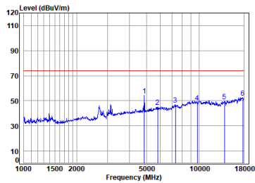
Antenna 1 11b_TX_CH_06_Vertical-Peak
