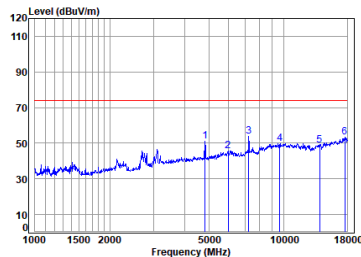
Antenna 2 11b_TX_CH_01_Vertical-Peak
