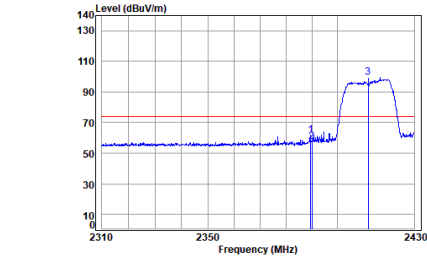
Antenna 2 11n_HT(20M)_TX_CH_01_Horizontal-Peak
