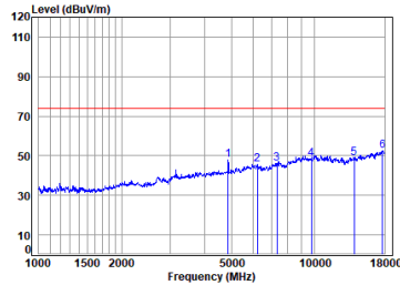
Antenna 2 11n_HT(20M)_TX_CH_06_Horizontal-Peak
