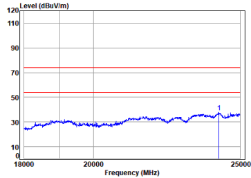
Antenna 1 11b_TX_CH_06_Horizontal-Peak
