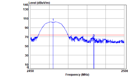
Antenna 1 11b_TX_CH_11_Vertical-Peak
