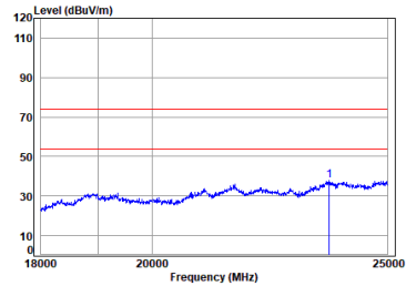
Antenna 2 11b_TX_CH_06_Vertical-Peak
