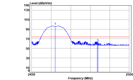
Antenna 2 11b_TX_CH_11_Horizontal-Peak
