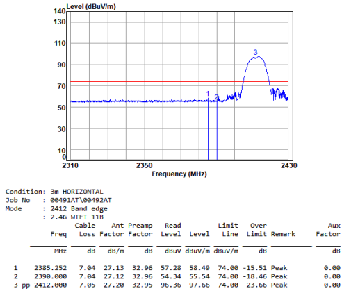
Antenna 1 11b_TX_CH_01_Horizontal-Peak
