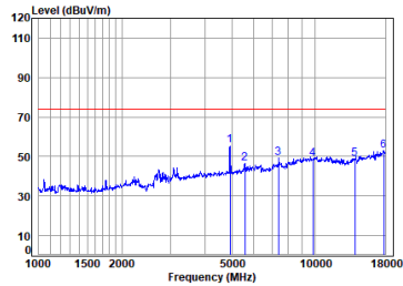
Antenna 2 11b_TX_CH_11_Vertical-Peak
