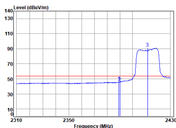
Antenna 2 11g_TX_CH_01_Horizontal-Avg
