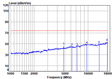
Antenna 2 11n_HT(20M)_TX_CH_01_Horizontal-Peak
