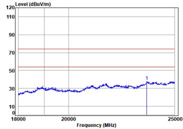
Antenna 1 11b_TX_CH_06_Vertical-Peak
