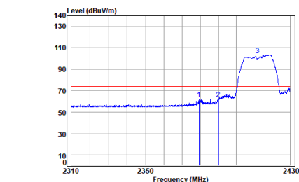
Antenna 1 11g_TX_CH_01_Horizontal-Peak
