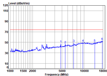
Antenna 2 11n_HT(20M)_TX_CH_01_Vertical-Peak
