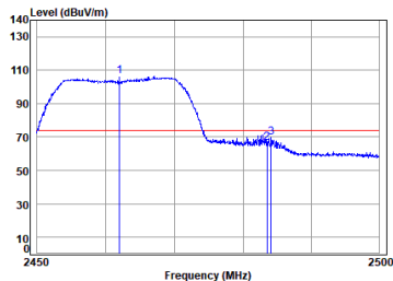
Antenna 2 11n_HT(20M)_TX_CH_11_Vertical-Peak
