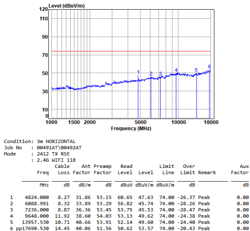
Antenna 1 11b_TX_CH_01_Horizontal-Peak
