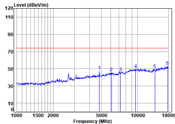
Antenna 2 11b_TX_CH_01_Horizontal-Peak
