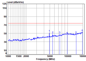
Antenna 2 11n_HT(20M)_TX_CH_11_Vertical-Peak
