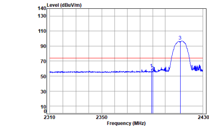
Antenna 2 11b_TX_CH_01_Horizontal-Peak
