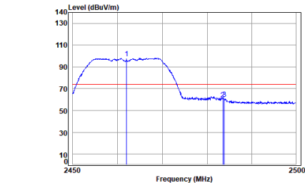
Antenna 2 11g_TX_CH_11_Horizontal-Peak
