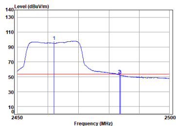
Antenna 2 11g_TX_CH_11_Vertical-Avg
