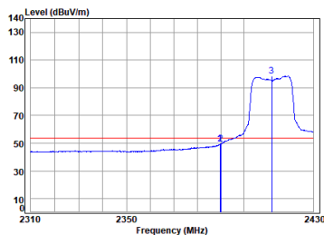
Antenna 2 11g_TX_CH_01_Vertical-Avg
