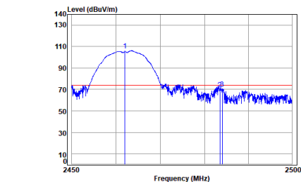
Antenna 2 11b_TX_CH_11_Vertical-Peak
