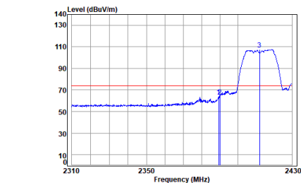
Antenna 2 11g_TX_CH_01_Vertical-Peak
