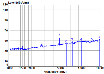
Antenna 1 11n_HT(20M)_TX_CH_11_Vertical-Peak
