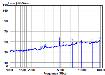
Antenna 2 11b_TX_CH_06_Vertical-Peak
