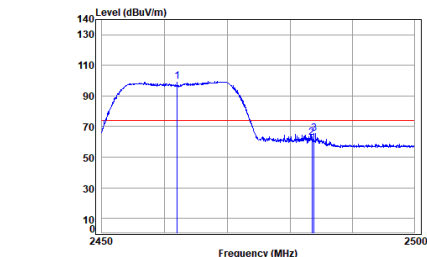
Antenna 1 11n_HT(20M)_TX_CH_11_Horizontal-Peak
