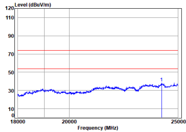
Antenna 2 11b_TX_CH_06_Horizontal-Peak
