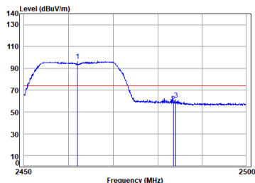
Antenna 2 11n_HT(20M)_TX_CH_11_Horizontal-Peak
