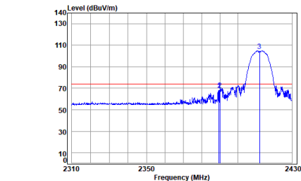
Antenna 2 11b_TX_CH_01_Vertical-Peak
