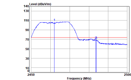
Antenna 2 11g_TX_CH_11_Vertical-Peak
