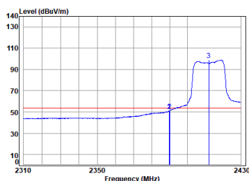
Antenna 1 11g_TX_CH_01_Vertical-Avg
