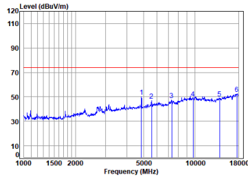
Antenna 2 11n_HT(20M)_TX_CH_06_Vertical-Peak
