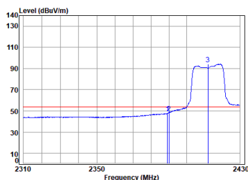
Antenna 1 11g_TX_CH_01_Horizontal-Avg
