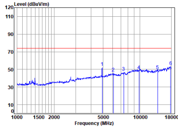
Antenna 1 11n_HT(20M)_TX_CH_11_Horizontal-Peak
