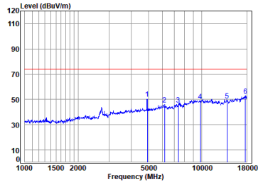
Antenna 2 11b_TX_CH_11_Horizontal-Peak
