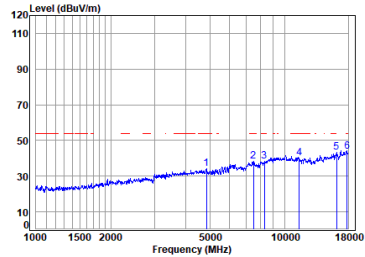
Antenna 1 11a_TX_CH_149_Horizontal-Avg
