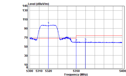
Antenna 2 11ac_VHT(20M)_TX_CH_64_Vertical-Peak
