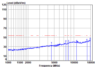
Antenna 2 11a_TX_CH_100_Vertical-Avg
