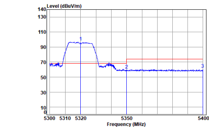
Antenna 1 11a_TX_CH_64_Horizontal-Peak
