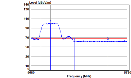
Antenna 1 11a_TX_CH_140_Horizontal-Peak
