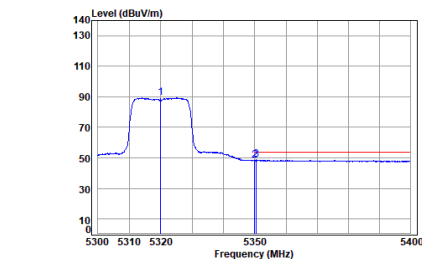
Antenna 2 11ac_VHT(20M)_TX_CH_64_Vertical-Avg
