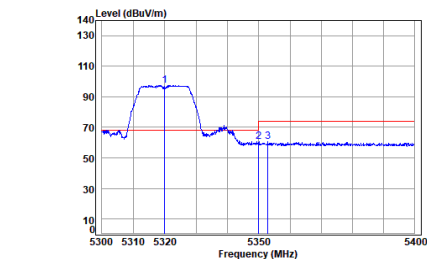
Antenna 2 11a_TX_CH_64_Vertical-Peak
