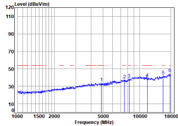
Antenna 2 11a_TX_CH_157_Horizontal-Avg
