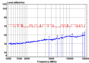
Antenna 1 11a_TX_CH_100_Horizontal-Peak
