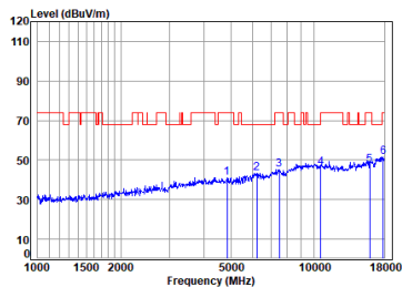
Antenna 2 11a_TX_CH_60_Horizontal-Peak
