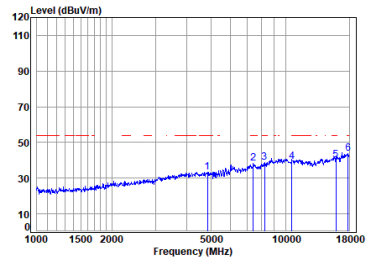
Antenna 1 11a_TX_CH_60_Horizontal-Avg
