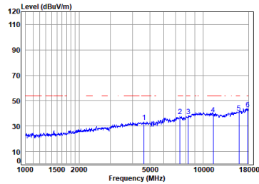
Antenna 2 11a_TX_CH_140_Vertical-Avg
