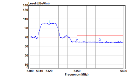
Antenna 1 11a_TX_CH_64_Vertical-Peak
