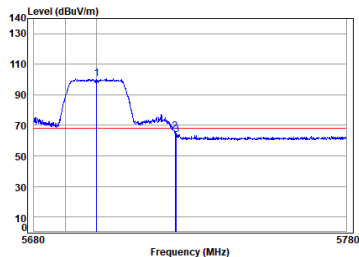
Antenna 2 11ac_VHT(20M)_TX_CH_140_Horizontal-Peak
