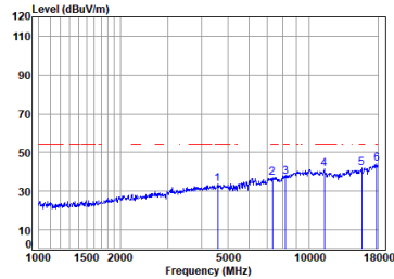
Antenna 2 11a_TX_CH_140_Horizontal-Avg
