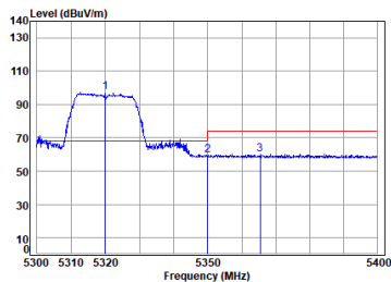
Antenna 1 11ac_VHT(20M)_TX_CH_64_Horizontal-Peak
