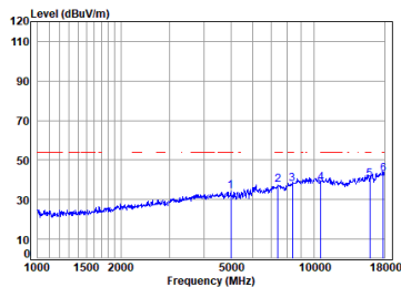
Antenna 2 11a_TX_CH_60_Horizontal-Avg
