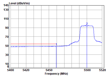
Antenna 2 11a_TX_CH_100_Vertical-Avg
