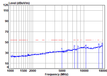
Antenna 1 11a_TX_CH_64_Horizontal-Avg
