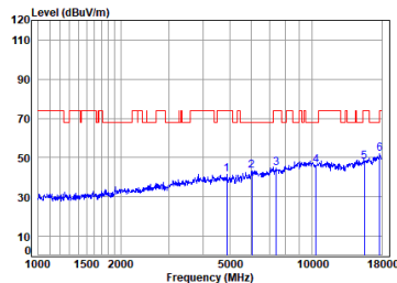
Antenna 2 11a_TX_CH_36_Vertical-Peak
