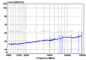
Antenna 2 11a_TX_CH_48_Vertical-Avg
