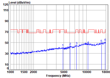
Antenna 1 11a_TX_CH_52_Horizontal-Peak
