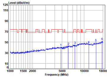
Antenna 2 11a_TX_CH_157_Vertical-Peak
