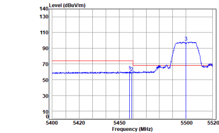
Antenna 2 11a_TX_CH_100_Horizontal-Peak
