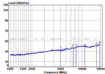
Antenna 1 11a_TX_CH_100_Horizontal-Avg
