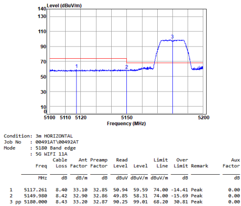
Antenna 1 11a_TX_CH_36_Horizontal-Peak
