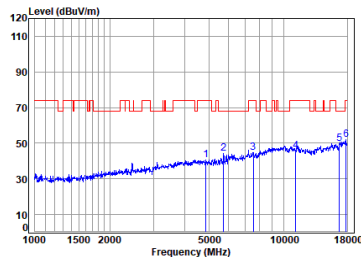
Antenna 2 11a_TX_CH_116_Vertical-Peak
