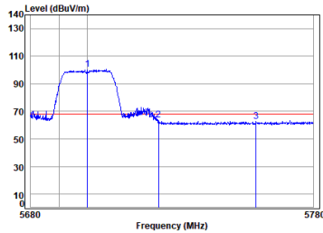
Antenna 1 11ac_VHT(20M)_TX_CH_140_Horizontal-Peak
