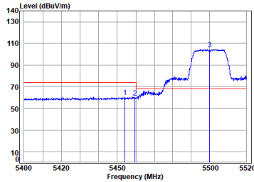
Antenna 1 11ac_VHT(20M)_TX_CH_100_Vertical-Peak
