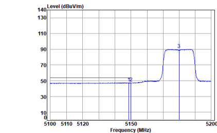
Antenna 1 11ac_VHT(20M)_TX_CH_36_Horizontal-Avg
