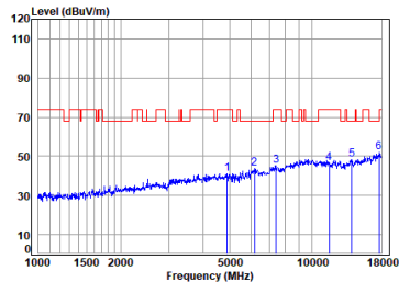
Antenna 1 11a_TX_CH_157_Horizontal-Peak
