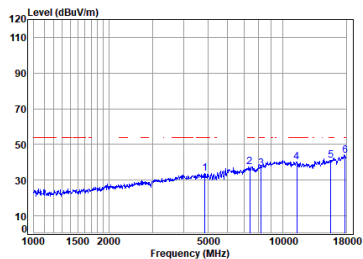
Antenna 2 11a_TX_CH_44_Horizontal-Avg
