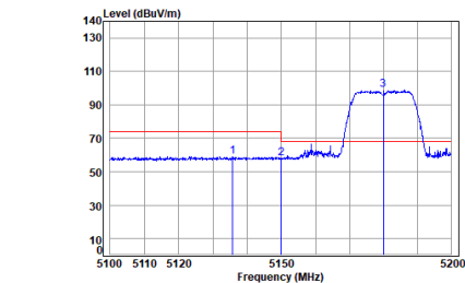
Antenna 1 11ac_VHT(20M)_TX_CH_36_Horizontal-Peak
