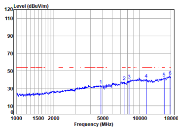
Antenna 1 11a_TX_CH_140_Horizontal-Avg
