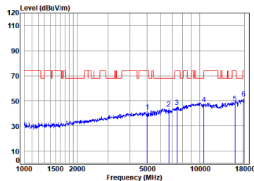
Antenna 1 11a_TX_CH_60_Vertical-Peak
