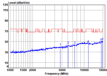
Antenna 2 11a_TX_CH_140_Vertical-Peak
