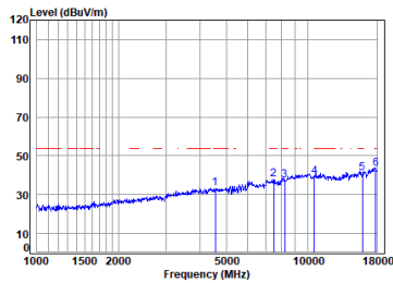
Antenna 2 11a_TX_CH_60_Vertical-Avg
