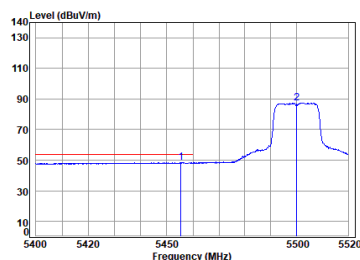
Antenna 1 11a_TX_CH_100_Horizontal-Avg
