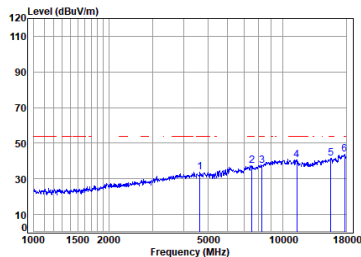
Antenna 1 11a_TX_CH_140_Vertical-Avg
