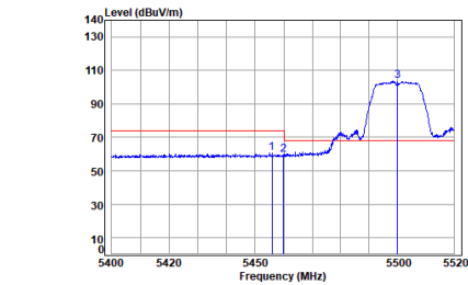
Antenna 2 11a_TX_CH_100_Vertical-Peak
