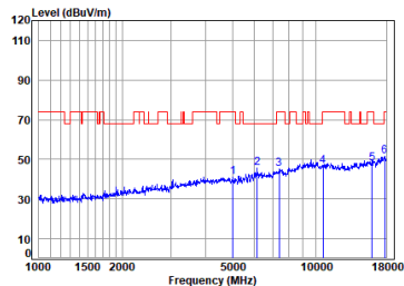
Antenna 2 11a_TX_CH_64_Vertical-Peak
