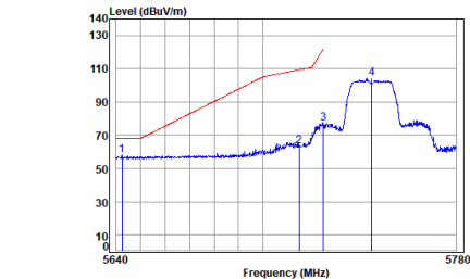
Antenna 2 11ac_VHT(20M)_TX_CH_149_Horizontal-Peak
