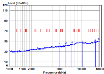
Antenna 2 11a_TX_CH_52_Vertical-Peak
