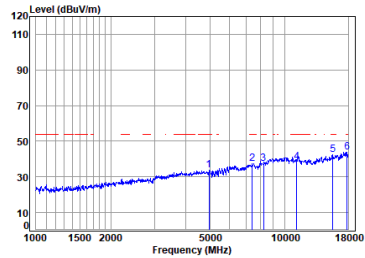
Antenna 1 11a_TX_CH_116_Vertical-Avg
