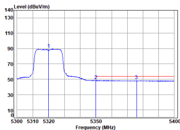
Antenna 2 11a_TX_CH_64_Vertical-Avg
