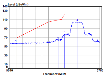
Antenna 2 11a_TX_CH_149_Vertical-Peak
