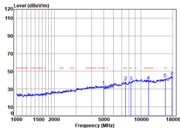
Antenna 2 11a_TX_CH_149_Vertical-Avg
