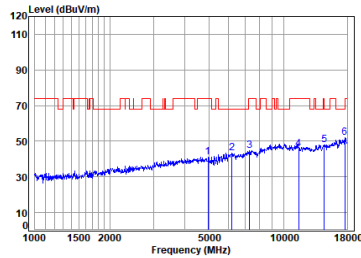
Antenna 1 11a_TX_CH_149_Vertical-Peak
