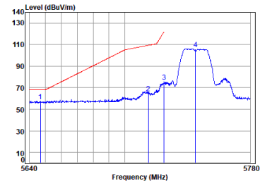
Antenna 1 11a_TX_CH_149_Vertical-Peak
