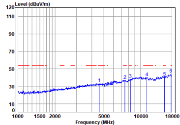
Antenna 1 11a_TX_CH_48_Horizontal-Avg
