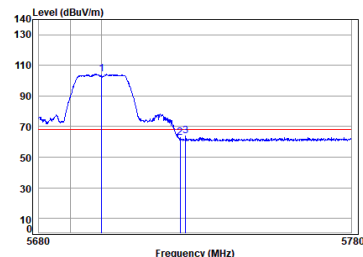
Antenna 2 11a_TX_CH_140_Vertical-Peak
