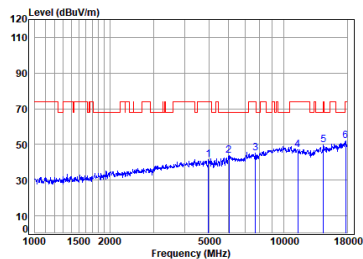
Antenna 1 11a_TX_CH_140_Horizontal-Peak
