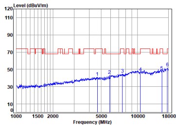
Antenna 2 11a_TX_CH_60_Vertical-Peak
