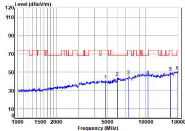
Antenna 1 11a_TX_CH_48_Horizontal-Peak
