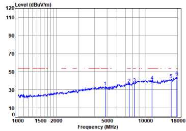
Antenna 1 11a_TX_CH_149_Vertical-Avg
