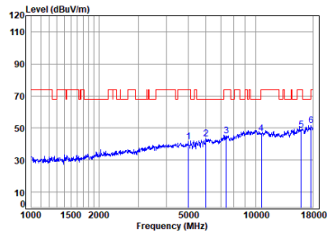
Antenna 2 11a_TX_CH_64_Horizontal-Peak
