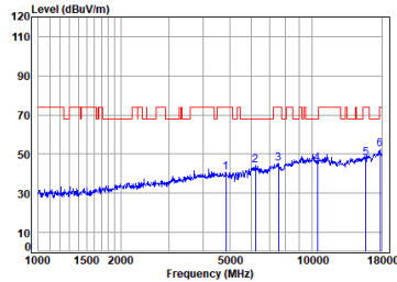
Antenna 2 11a_TX_CH_48_Horizontal-Peak
