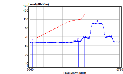
Antenna 1 11ac_VHT(20M)_TX_CH_149_Horizontal-Peak
