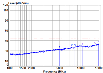
Antenna 1 11a_TX_CH_64_Vertical-Avg
