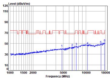
Antenna 2 11a_TX_CH_52_Horizontal-Peak
