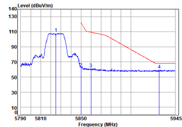
Antenna 1 11a_TX_CH_165_Vertical-Peak
