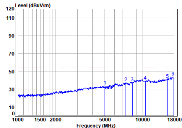
Antenna 2 11a_TX_CH_64_Vertical-Avg
