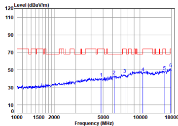
Antenna 1 11a_TX_CH_60_Horizontal-Peak
