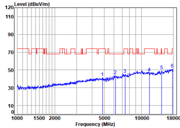
Antenna 2 11a_TX_CH_157_Horizontal-Peak
