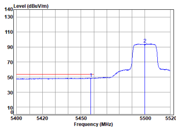
Antenna 2 11ac_VHT(20M)_TX_CH_100_Vertical-Avg
