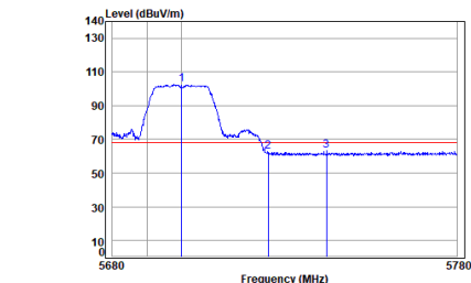
Antenna 2 11a_TX_CH_140_Horizontal-Peak
