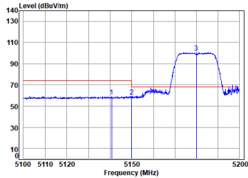
Antenna 2 11ac_VHT(20M)_TX_CH_36_Horizontal-Peak
