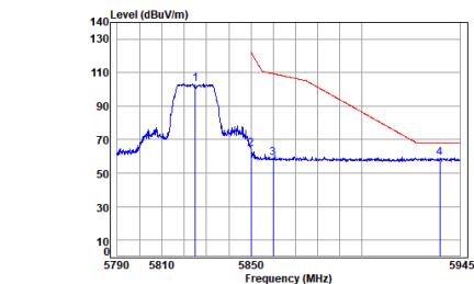
Antenna 1 11ac_VHT(20M)_TX_CH_165_Horizontal-Peak
