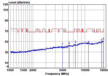
Antenna 1 11a_TX_CH_116_Horizontal-Peak
