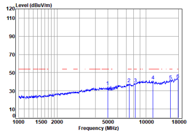
Antenna 1 11a_TX_CH_44_Horizontal-Avg
