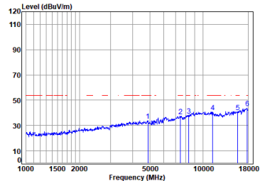
Antenna 1 11a_TX_CH_48_Vertical-Avg
