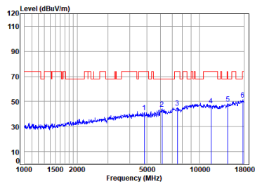
Antenna 2 11a_TX_CH_165_Horizontal-Peak
