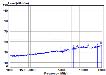
Antenna 2 11a_TX_CH_52_Vertical-Avg
