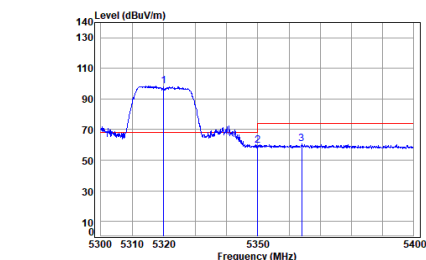
Antenna 2 11ac_VHT(20M)_TX_CH_64_Horizontal-Peak
