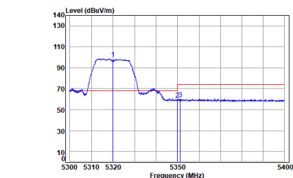
Antenna 2 11a_TX_CH_64_Horizontal-Peak
