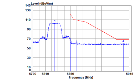
Antenna 2 11ac_VHT(20M)_TX_CH_165_Horizontal-Peak
