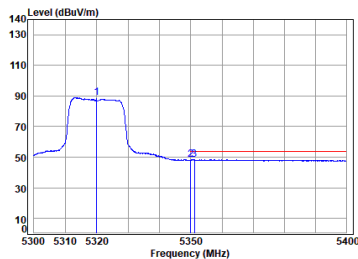
Antenna 1 11a_TX_CH_64_Horizontal-Avg
