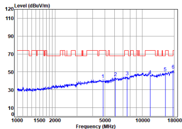
Antenna 1 11a_TX_CH_157_Vertical-Peak
