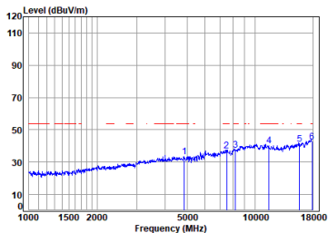
Antenna 1 11a_TX_CH_165_Vertical-Avg
