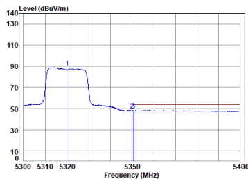
Antenna 1 11ac_VHT(20M)_TX_CH_64_Horizontal-Avg
