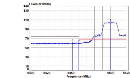
Antenna 1 11a_TX_CH_100_Vertical-Peak
