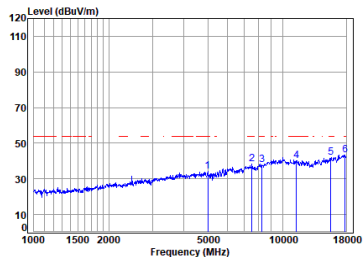
Antenna 2 11a_TX_CH_44_Vertical-Avg
