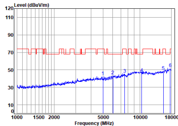
Antenna 2 11a_TX_CH_36_Horizontal-Peak
