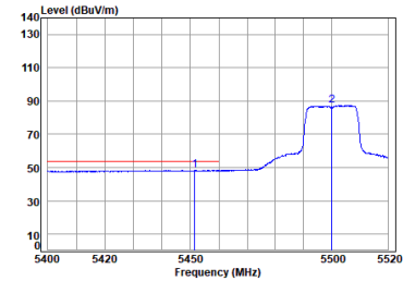
Antenna 1 11ac_VHT(20M)_TX_CH_100_Horizontal-Avg
