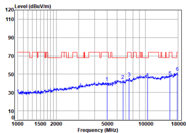
Antenna 2 11a_TX_CH_44_Horizontal-Peak
