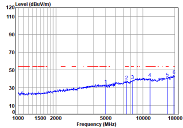
Antenna 1 11a_TX_CH_52_Horizontal-Avg
