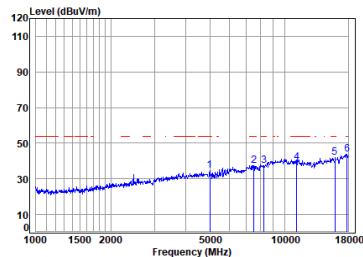
Antenna 2 11a_TX_CH_116_Vertical-Avg
