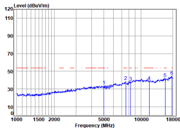
Antenna 2 11a_TX_CH_165_Vertical-Avg
