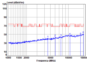
Antenna 1 11a_TX_CH_64_Horizontal-Peak
