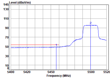
Antenna 1 11ac_VHT(20M)_TX_CH_100_Vertical-Avg
