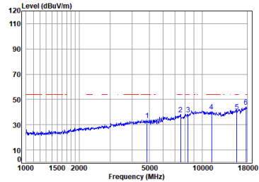
Antenna 2 11a_TX_CH_48_Horizontal-Avg
