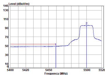
Antenna 1 11a_TX_CH_100_Vertical-Avg
