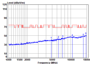
Antenna 1 11a_TX_CH_64_Vertical-Peak
