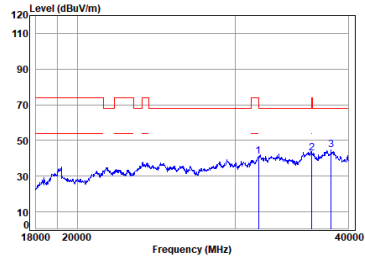
Antenna 1 11a_TX_CH_100_Vertical-Peak
