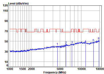
Antenna 2 11a_TX_CH_149_Horizontal-Peak
