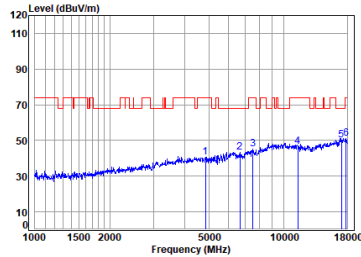
Antenna 2 11a_TX_CH_140_Horizontal-Peak
