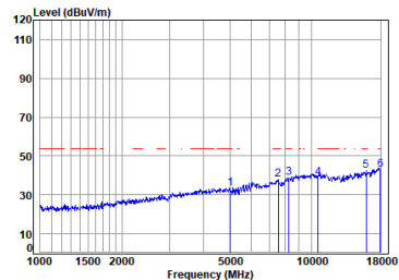
Antenna 1 11a_TX_CH_60_Vertical-Avg
