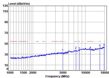
Antenna 2 11a_TX_CH_165_Horizontal-Avg
