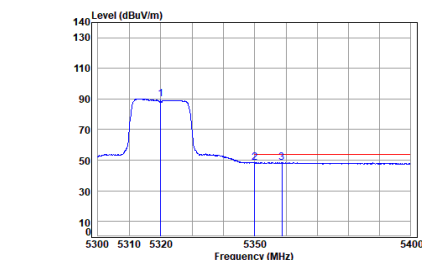
Antenna 2 11ac_VHT(20M)_TX_CH_64_Horizontal-Avg
