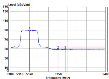
Antenna 2 11a_TX_CH_64_Horizontal-Avg
