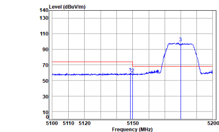
Antenna 2 11a_TX_CH_36_Vertical-Peak
