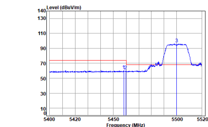
Antenna 1 11a_TX_CH_100_Horizontal-Peak
