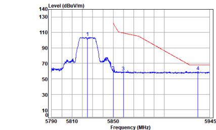
Antenna 1 11a_TX_CH_165_Horizontal-Peak
