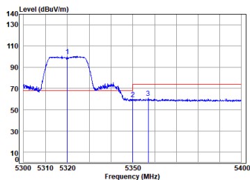
Antenna 1 11ac_VHT(20M)_TX_CH_64_Vertical-Peak
