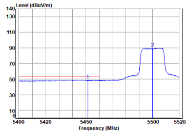
Antenna 2 11a_TX_CH_100_Horizontal-Avg
