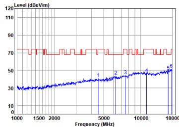
Antenna 2 11a_TX_CH_116_Horizontal-Peak
