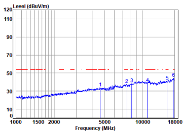
Antenna 2 11a_TX_CH_100_Horizontal-Avg
