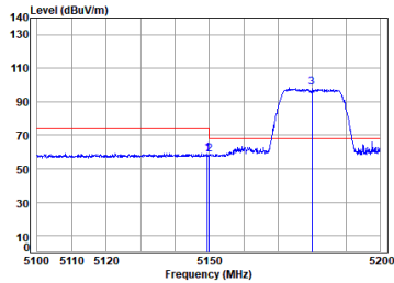
Antenna 2 11ac_VHT(20M)_TX_CH_36_Vertical-Peak
