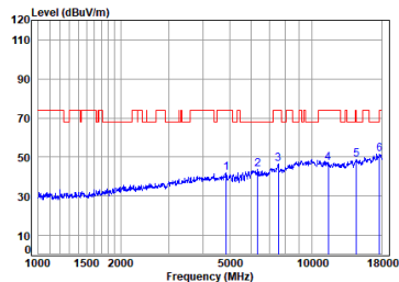
Antenna 2 11a_TX_CH_149_Vertical-Peak
