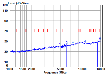
Antenna 2 11a_TX_CH_100_Vertical-Peak
