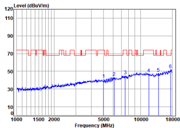
Antenna 1 11a_TX_CH_165_Vertical-Peak
