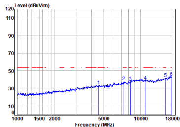
Antenna 1 11a_TX_CH_100_Vertical-Avg
