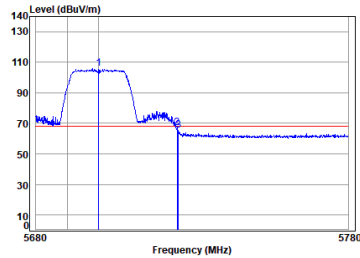
Antenna 1 11ac_VHT(20M)_TX_CH_140_Vertical-Peak
