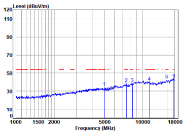
Antenna 1 11a_TX_CH_165_Horizontal-Avg
