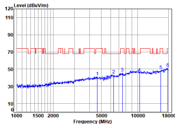
Antenna 1 11a_TX_CH_44_Vertical-Peak
