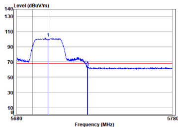
Antenna 2 11ac_VHT(20M)_TX_CH_140_Vertical-Peak
