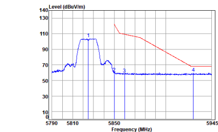
Antenna 2 11a_TX_CH_165_Horizontal-Peak
