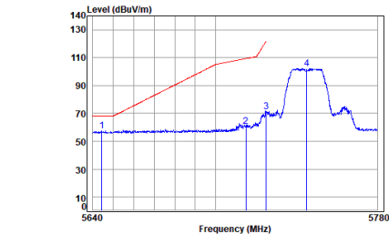
Antenna 1 11a_TX_CH_149_Horizontal-Peak
