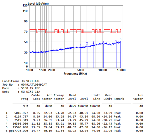
Antenna 1 11a_TX_CH_36_Vertical-Peak
