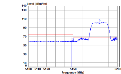
Antenna 1 11ac_VHT(20M)_TX_CH_36_Vertical-Peak
