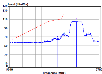
Antenna 1 11ac_VHT(20M)_TX_CH_149_Vertical-Peak
