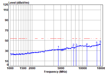
Antenna 2 11a_TX_CH_157_Vertical-Avg
