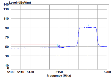
Antenna 2 11ac_VHT(20M)_TX_CH_36_Horizontal-Avg
