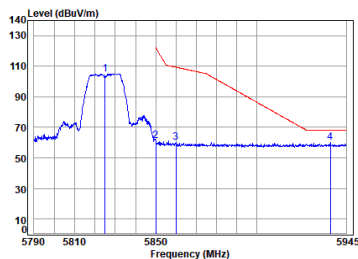
Antenna 2 11a_TX_CH_165_Vertical-Peak
