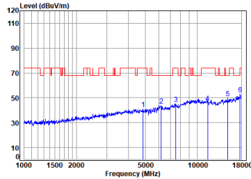
Antenna 1 11a_TX_CH_149_Horizontal-Peak
