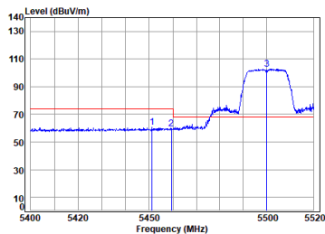
Antenna 2 11ac_VHT(20M)_TX_CH_100_Vertical-Peak
