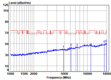
Antenna 1 11a_TX_CH_116_Vertical-Peak
