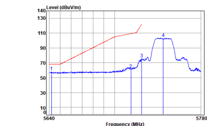
Antenna 2 11a_TX_CH_149_Horizontal-Peak
