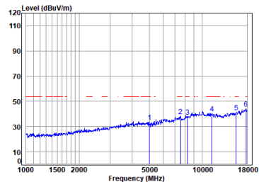
Antenna 1 11a_TX_CH_44_Vertical-Avg
