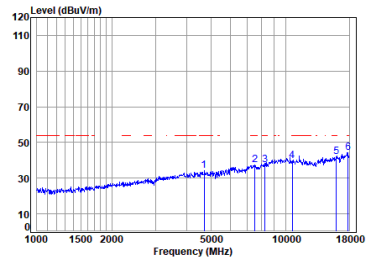
Antenna 2 11a_TX_CH_64_Horizontal-Avg
