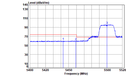
Antenna 1 11ac_VHT(20M)_TX_CH_100_Horizontal-Peak
