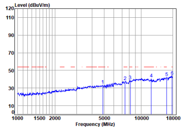
Antenna 1 11a_TX_CH_157_Horizontal-Avg
