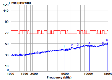
Antenna 2 11a_TX_CH_48_Vertical-Peak
