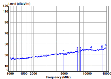
Antenna 2 11a_TX_CH_52_Horizontal-Avg
