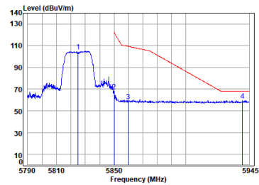
Antenna 2 11ac_VHT(20M)_TX_CH_165_Vertical-Peak
