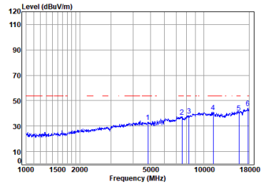
Antenna 1 11a_TX_CH_52_Vertical-Avg
