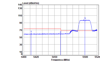
Antenna 2 11ac_VHT(20M)_TX_CH_100_Horizontal-Peak
