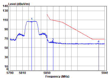
Antenna 1 11ac_VHT(20M)_TX_CH_165_Vertical-Peak
