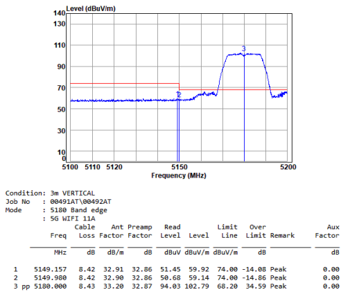
Antenna 1 11a_TX_CH_36_Vertical-Peak
