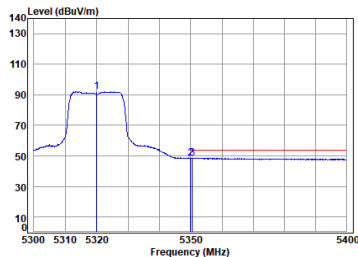
Antenna 1 11a_TX_CH_64_Vertical-Avg
