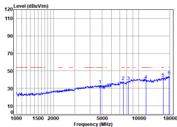
Antenna 2 11a_TX_CH_149_Horizontal-Avg
