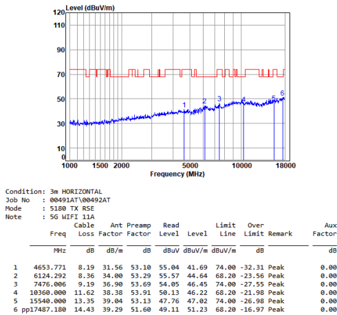
Antenna 1 11a_TX_CH_36_Horizontal-Peak
