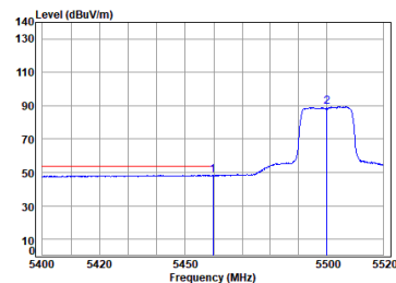
Antenna 2 11ac_VHT(20M)_TX_CH_100_Horizontal-Avg
