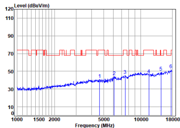
Antenna 2 11a_TX_CH_165_Vertical-Peak
