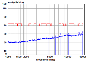
Antenna 1 11a_TX_CH_44_Horizontal-Peak
