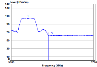
Antenna 1 11a_TX_CH_140_Vertical-Peak
