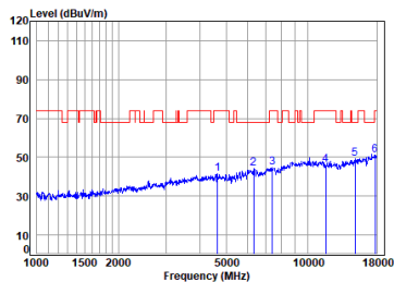
Antenna 1 11a_TX_CH_165_Horizontal-Peak
