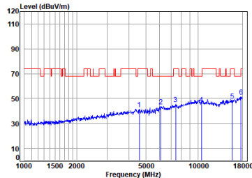
Antenna 1 11a_TX_CH_48_Vertical-Peak
