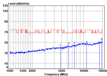
Antenna 2 11a_TX_CH_100_Horizontal-Peak
