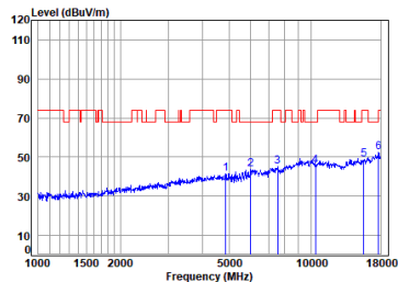
Antenna 2 11a_TX_CH_44_Vertical-Peak
