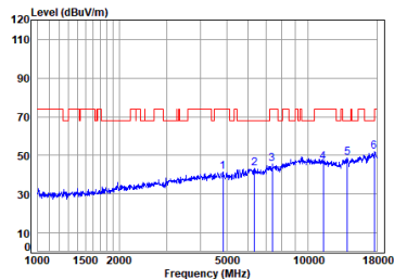
Antenna 1 11a_TX_CH_140_Vertical-Peak
