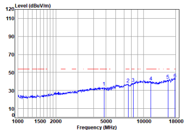
Antenna 1 11a_TX_CH_157_Vertical-Avg
