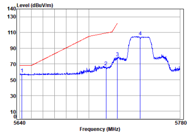
Antenna 2 11ac_VHT(20M)_TX_CH_149_Vertical-Peak
