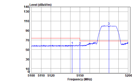
Antenna 2 11a_TX_CH_36_Horizontal-Peak
