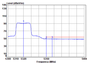
Antenna 1 11ac_VHT(20M)_TX_CH_64_Vertical-Avg
