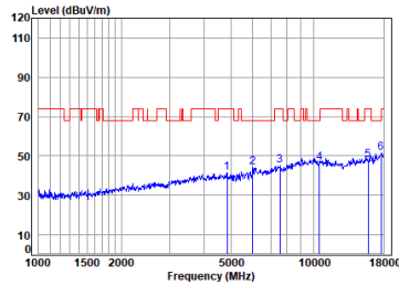
Antenna 1 11a_TX_CH_52_Vertical-Peak
