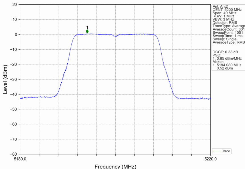
802.11ac(VHT20)_MCH_5200MHz_Ant2_NTNV
