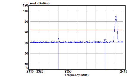
Antenna 1 BLE_1M_TX_CH_00_Horizontal-Peak
