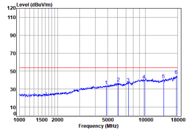
Antenna 2 BLE_2M_TX_CH_19_Vertical-Avg
