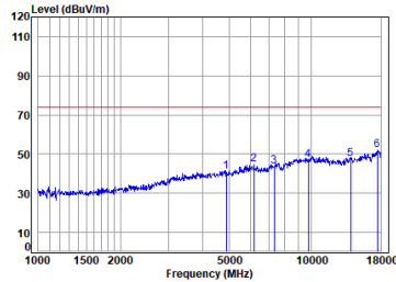
Antenna 1 BLE_2M_TX_CH_19_Horizontal-Peak
