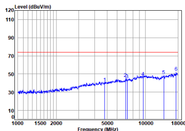
Antenna 2 BLE_2M_TX_CH_00_Vertical-Peak
