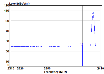
Antenna 1 BLE_1M_TX_CH_00_Vertical-Avg
