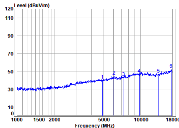
Antenna 2 BLE_1M_TX_CH_19_Vertical-Peak
