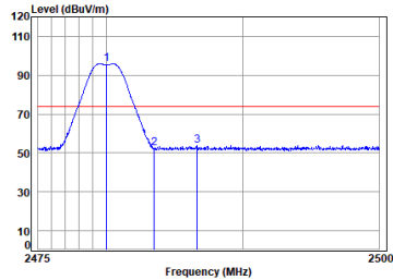
Antenna 2 BLE_2M_TX_CH_39_Horizontal-Peak
