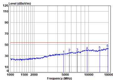
Antenna 2 BLE_1M_TX_CH_00_Vertical-Avg
