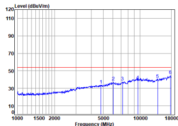
Antenna 2 BLE_2M_TX_CH_00_Horizontal-Avg
