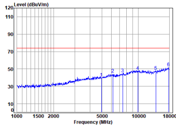
Antenna 2 BLE_2M_TX_CH_39_Vertical-Peak
