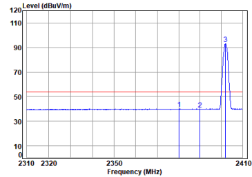
Antenna 2 BLE_1M_TX_CH_00_Horizontal-Avg
