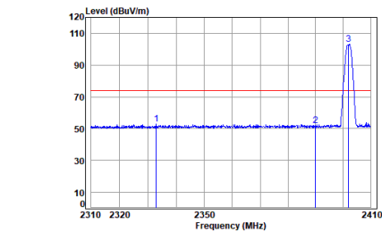
Antenna 1 BLE_1M_TX_CH_00_Vertical-Peak
