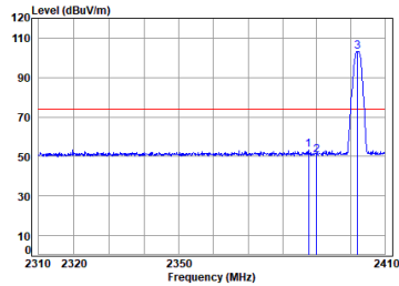
Antenna 2 BLE_1M_TX_CH_00_Vertical-Peak
