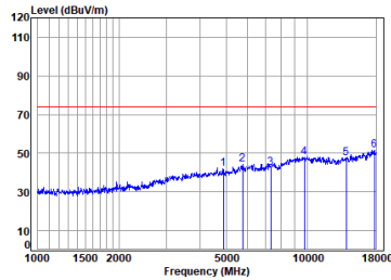
Antenna 2 BLE_2M_TX_CH_19_Vertical-Peak
