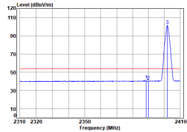
Antenna 2 BLE_2M_TX_CH_00_Vertical-Avg
