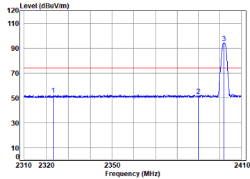
Antenna 2 BLE_1M_TX_CH_00_Horizontal-Peak
