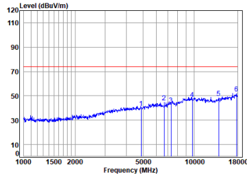
Antenna 2 BLE_1M_TX_CH_19_Horizontal-Peak
