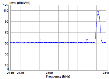
Antenna 2 BLE_2M_TX_CH_00_Vertical-Peak
