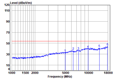
Antenna 2 BLE_1M_TX_CH_39_Vertical-Avg
