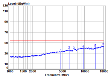
Antenna 2 BLE_1M_TX_CH_00_Horizontal-Avg
