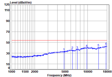
Antenna 2 BLE_1M_TX_CH_19_Horizontal-Avg
