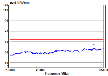
Antenna 2 BLE_1M_TX_CH_19_Horizontal-Peak
