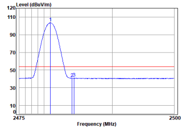
Antenna 2 BLE_1M_TX_CH_39_Vertical-Avg
