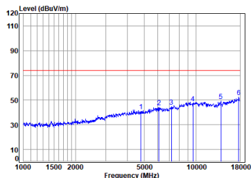
Antenna 2 BLE_1M_TX_CH_00_Horizontal-Peak
