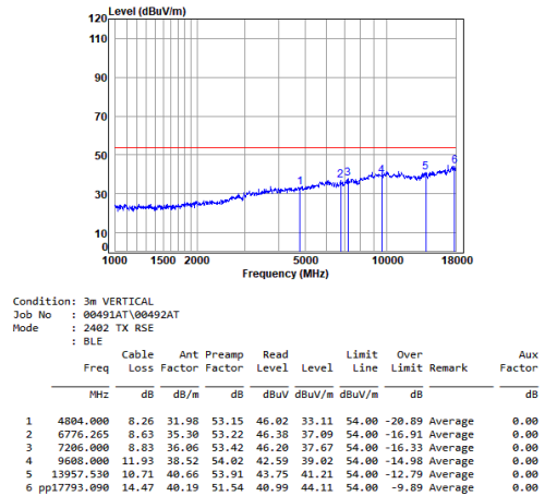
Antenna 1 BLE_1M_TX_CH_00_Vertical-Avg
