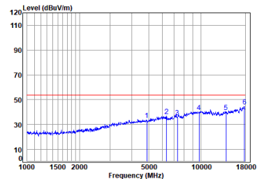
Antenna 2 BLE_1M_TX_CH_19_Vertical-Avg
