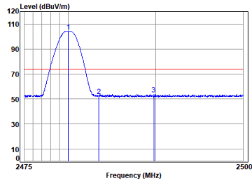
Antenna 2 BLE_1M_TX_CH_39_Vertical-Peak
