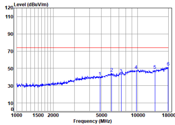
Antenna 1 BLE_2M_TX_CH_19_Vertical-Peak
