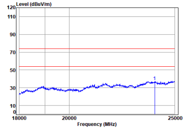
Antenna 1 BLE_1M_TX_CH_19_Vertical-Peak
