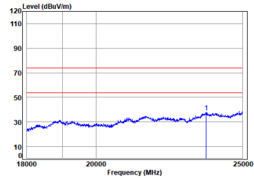
Antenna 2 BLE_1M_TX_CH_19_Vertical-Peak
