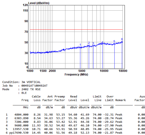
Antenna 1 BLE_1M_TX_CH_00_Vertical-Peak
