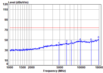
Antenna 2 BLE_2M_TX_CH_19_Horizontal-Peak
