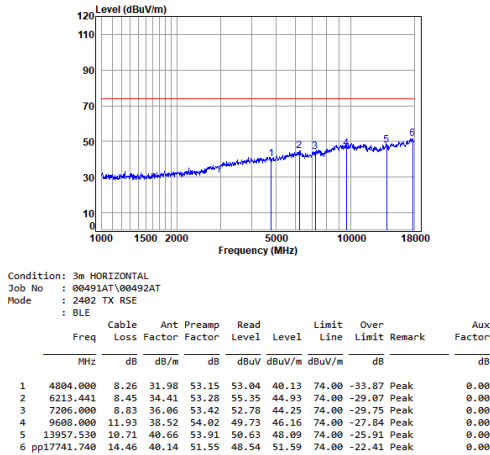
Antenna 1 BLE_1M_TX_CH_00_Horizontal-Peak
