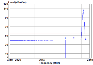
Antenna 2 BLE_1M_TX_CH_00_Vertical-Avg
