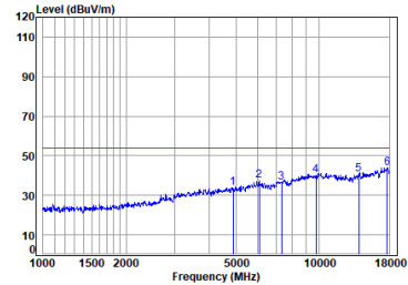
Antenna 2 BLE_2M_TX_CH_19_Horizontal-Avg
