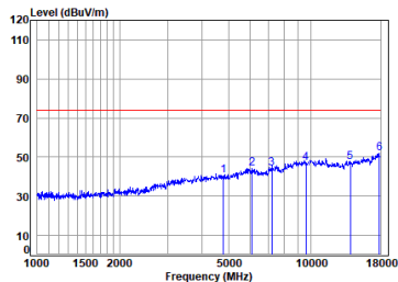
Antenna 2 BLE_1M_TX_CH_00_Vertical-Peak
