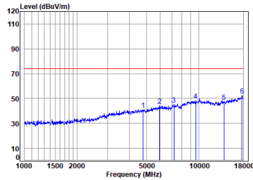
Antenna 1 BLE_2M_TX_CH_00_Vertical-Peak
