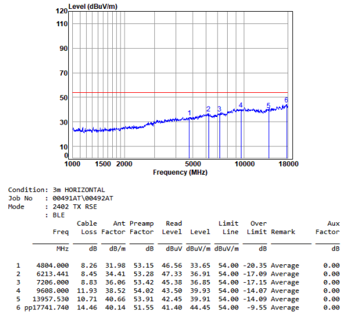
Antenna 1 BLE_1M_TX_CH_00_Horizontal-Avg
