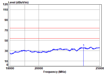
Antenna 1 BLE_1M_TX_CH_19_Horizontal-Peak
