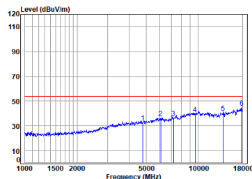
Antenna 2 BLE_2M_TX_CH_00_Vertical-Avg
