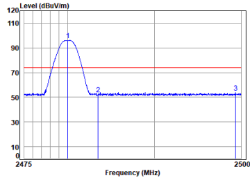
Antenna 2 BLE_1M_TX_CH_39_Horizontal-Peak
