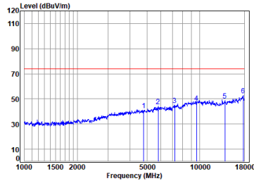
Antenna 1 BLE_2M_TX_CH_00_Horizontal-Peak
