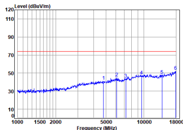
Antenna 2 BLE_2M_TX_CH_00_Horizontal-Peak
