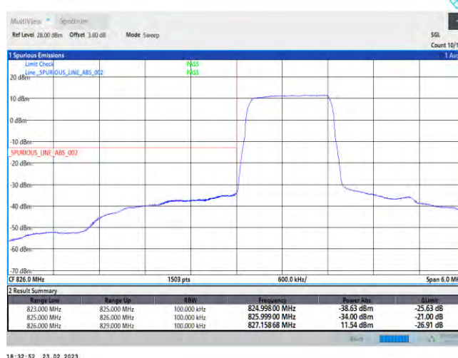
Band5-1.4MHz-QPSK-20427-6RB#0
