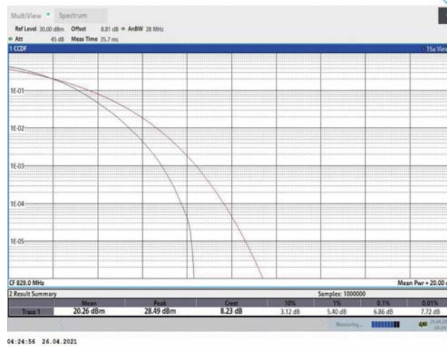
Band5-10MHz-16QAM-20450-50RB#0
