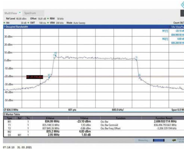
Band5-3MHz-16QAM-20525-15RB#0-2.697
