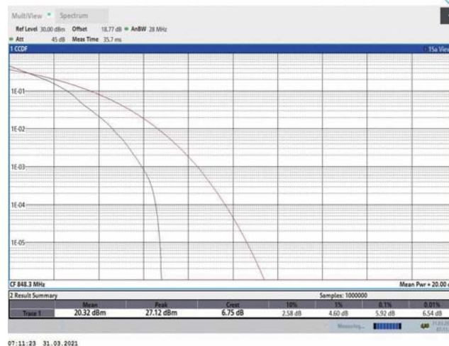
Band5-1.4MHz-QPSK-20643-1RB#0
