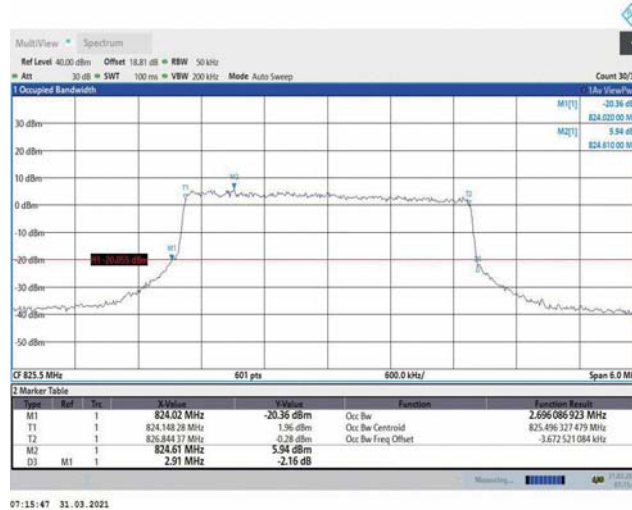
Band5-3MHz-16QAM-20415-15RB#0-2.696
