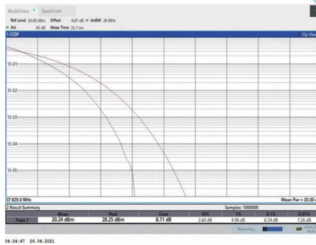
Band5-10MHz-QPSK-20450-50RB#0
