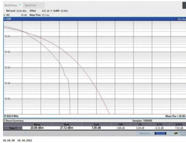
Band5-10MHz-16QAM-20450-1RB#0
