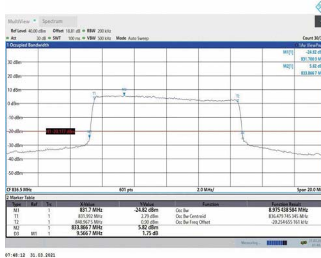
Band5-10MHz-QPSK-20525-50RB#0-8.975
