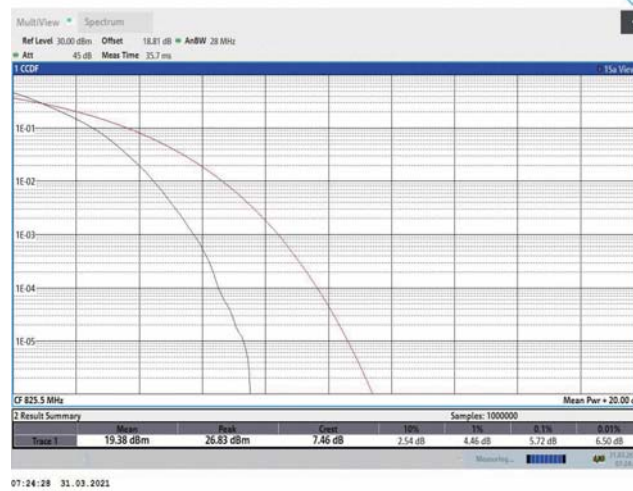
Band5-3MHz-QPSK-20415-15RB#0
