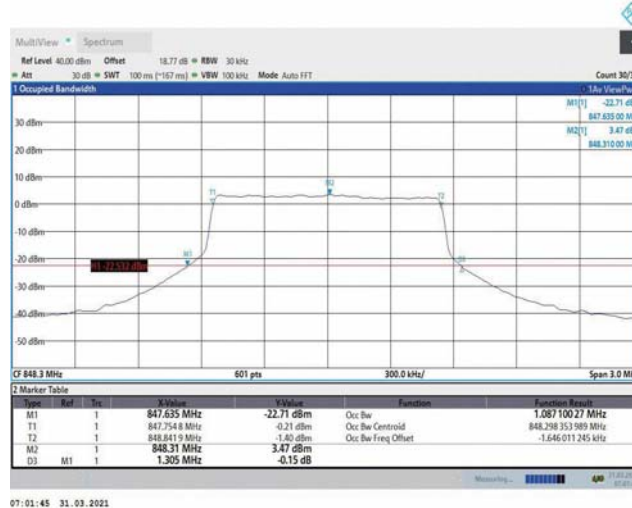
Band5-1.4MHz-16QAM-20643-6RB#0-1.087
