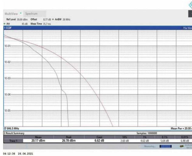
Band5-5MHz-QPSK-20625-1RB#0
