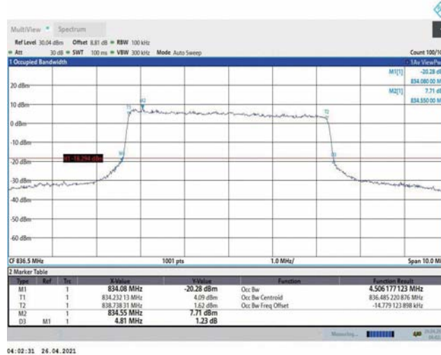
Band5-5MHz-16QAM-20525-25RB#0-4.506
