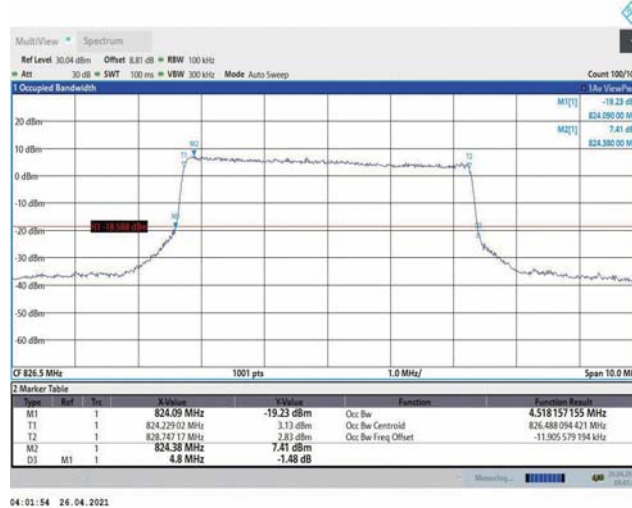
Band5-5MHz-16QAM-20425-25RB#0-4.518
