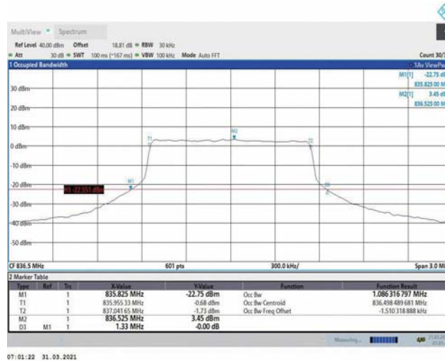
Band5-1.4MHz-16QAM-20525-6RB#0-1.086
