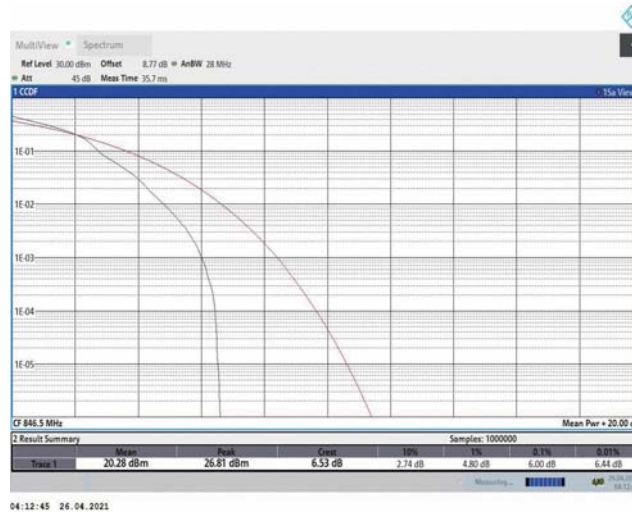
Band5-5MHz-16QAM-20625-1RB#0
