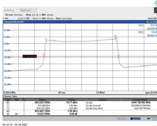
Band5-10MHz-QPSK-20450-50RB#0-9.041
