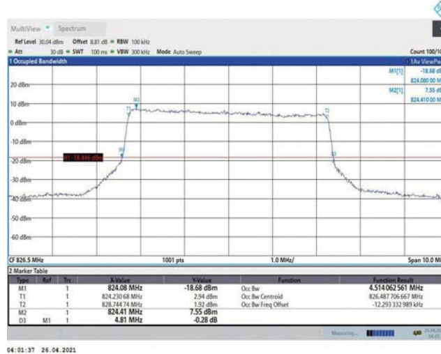
Band5-5MHz-QPSK-20425-25RB#0-4.514
