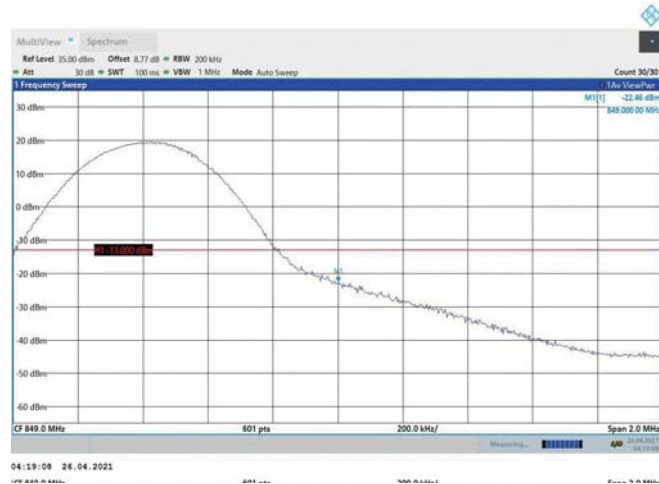
Band5-10MHz-16QAM-20600-1RB#49
