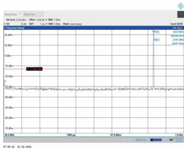
Band5-1.4MHz-QPSK-20525-1RB#0-Range1:30~1000MHz
