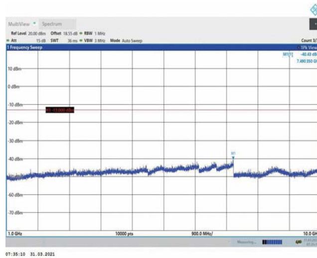
Band5-5MHz-QPSK-20625-1RB#0-Range2:1000~10000MHz
