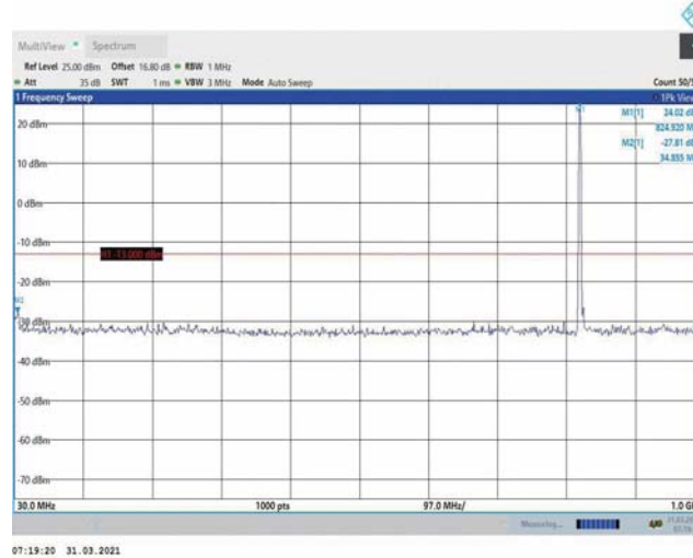
Band5-3MHz-16QAM-20415-1RB#0-Range1:30~1000MHz
