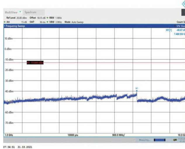
Band5-5MHz-16QAM-20525-1RB#0-Range2:1000~10000MHz
