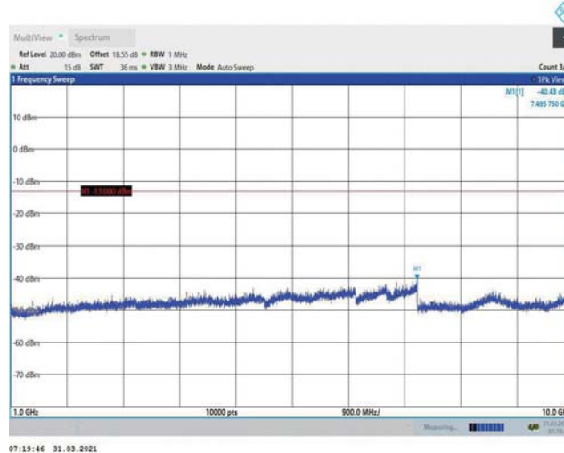
Band5-3MHz-QPSK-20525-1RB#0-Range2:1000~10000MHz
