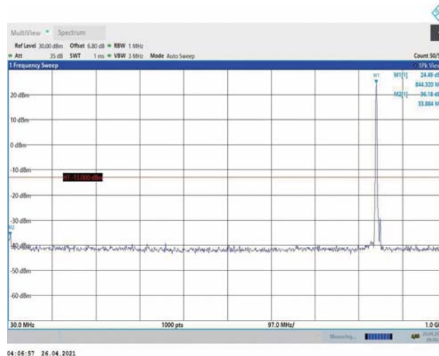
Band5-5MHz-QPSK-20625-1RB#0-Range1:30~1000MHz
