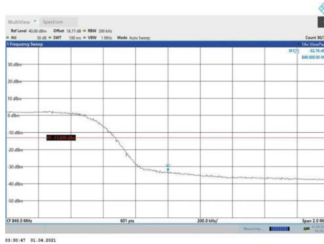
Band5-10MHz-16QAM-20600-50RB#0
