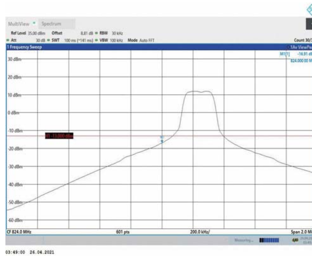
Band5-3MHz-16QAM-20415-1RB#0
