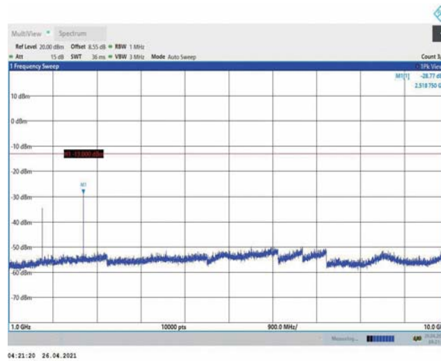
Band5-10MHz-16QAM-20600-1RB#0-Range2:1000~10000MHz
