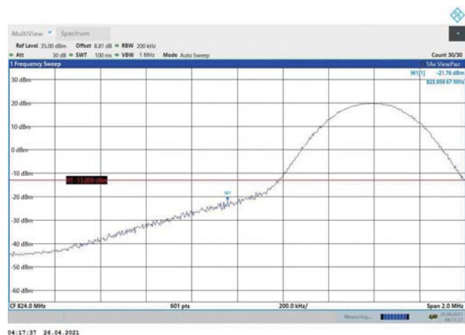
Band5-10MHz-16QAM-20450-1RB#0
