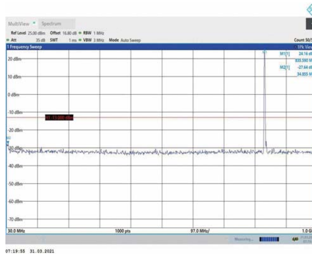
Band5-3MHz-16QAM-20525-1RB#0-Range1:30~1000MHz
