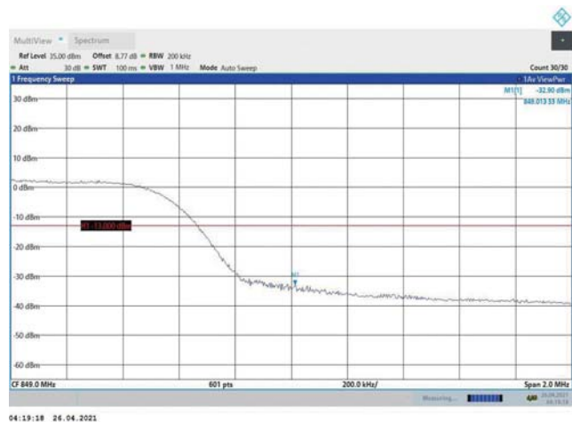
Band5-10MHz-QPSK-20600-50RB#0
