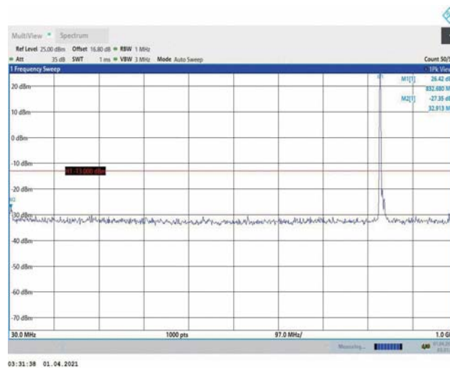
Band5-10MHz-QPSK-20525-1RB#0-Range1:30~1000MHz
