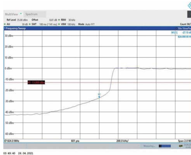
Band5-3MHz-16QAM-20415-15RB#0
