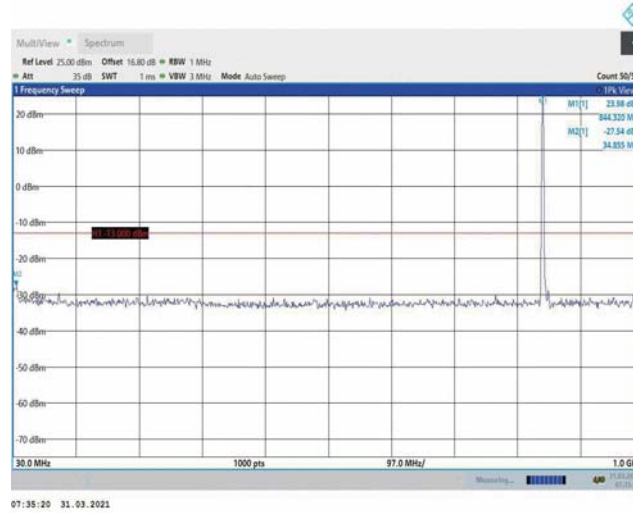
Band5-5MHz-16QAM-20625-1RB#0-Range1:30~1000MHz
