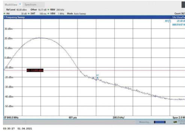
Band5-10MHz-16QAM-20600-1RB#49
