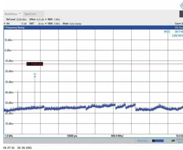
Band5-5MHz-16QAM-20625-1RB#0-Range2:1000~10000MHz
