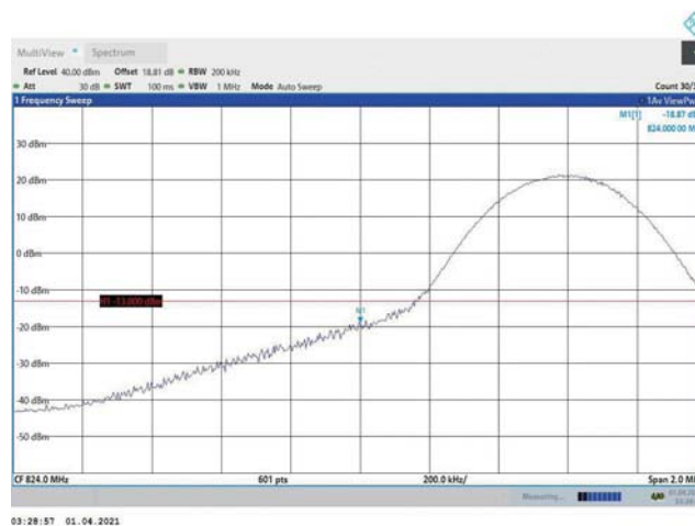
Band5-10MHz-16QAM-20450-1RB#0
