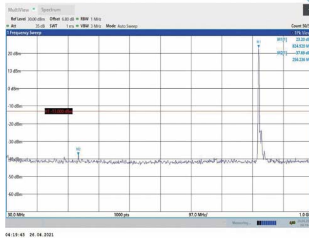
Band5-10MHz-QPSK-20450-1RB#0-Range1:30~1000MHz
