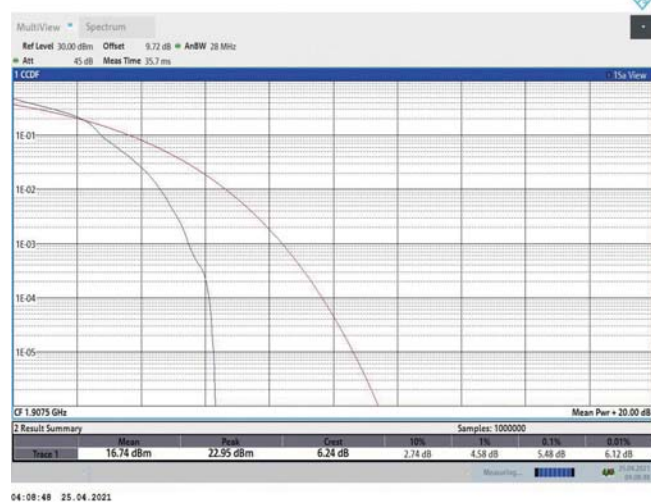
Band2-5MHz-16QAM-19175-1RB#0
