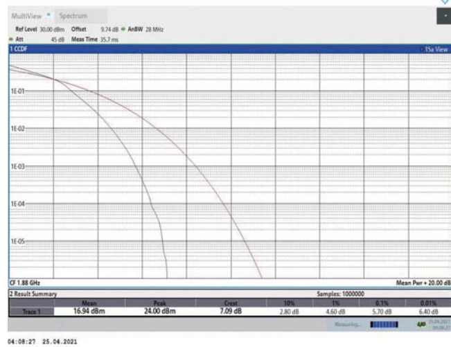
Band2-5MHz-16QAM-18900-25RB#0
