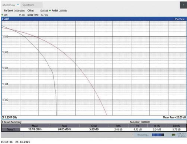
Band2-1.4MHz-QPSK-18607-1RB#0
