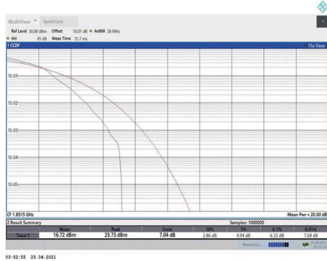
Band2-3MHz-16QAM-18615-1RB#0
