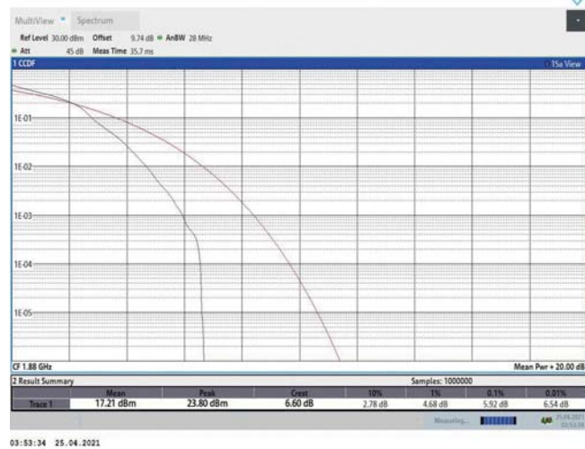
Band2-3MHz-16QAM-18900-1RB#0
