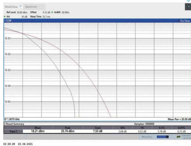
Band2-5MHz-16QAM-19175-25RB#0
