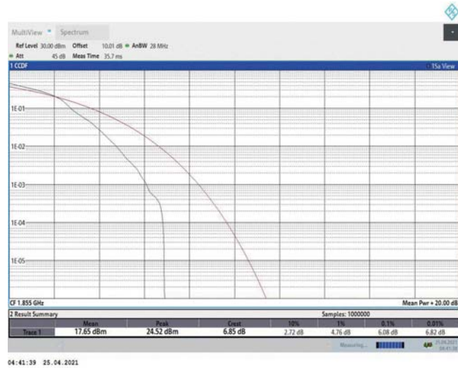
Band2-10MHz-16QAM-18650-1RB#0
