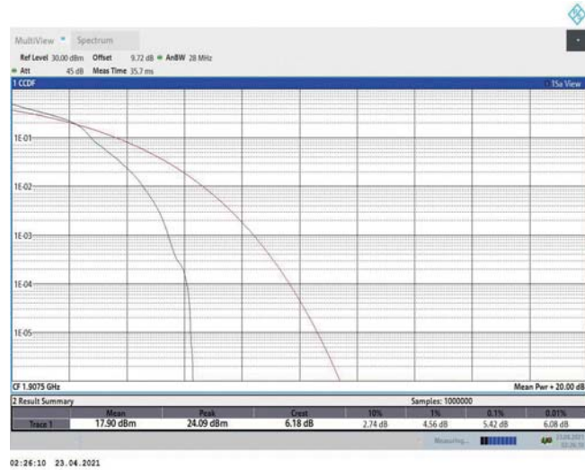
Band2-5MHz-16QAM-19175-1RB#0
