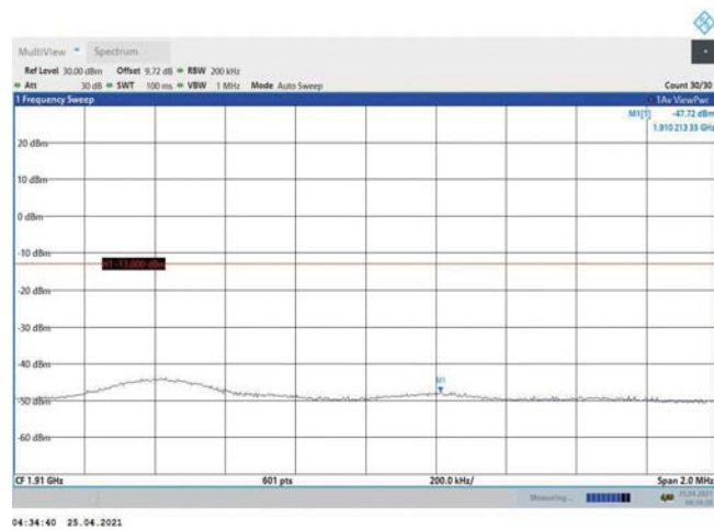
Band2-10MHz-QPSK-19150-1RB#0
