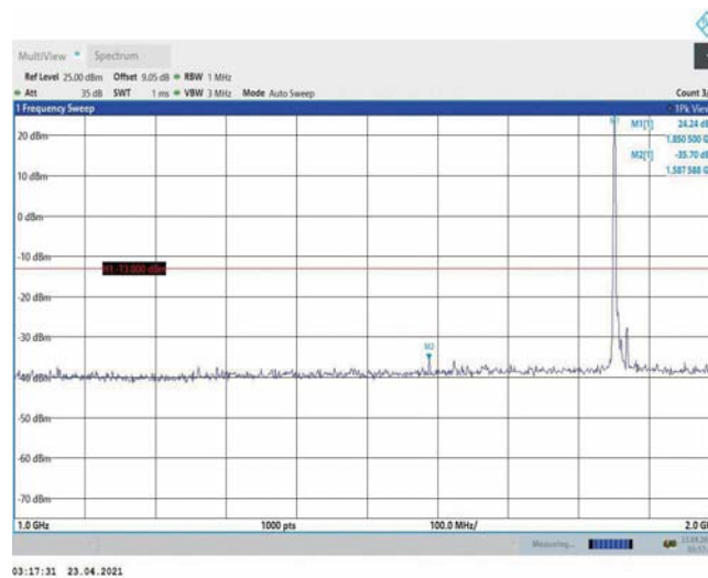
Band2-10MHz-16QAM-18650-1RB#0-Range2:1000~2000MHz
