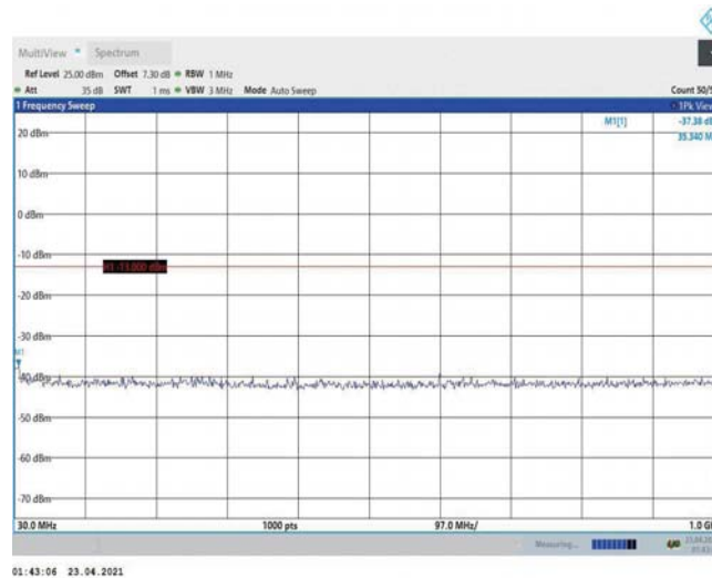
Band2-1.4MHz-16QAM-19193-1RB#0-Range1:30~1000MHz
