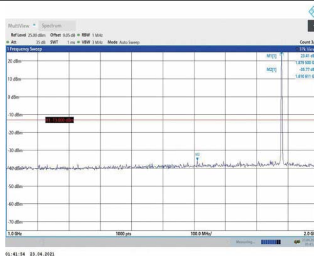
Band2-1.4MHz-16QAM-18900-1RB#0-Range2:1000~2000MHz
