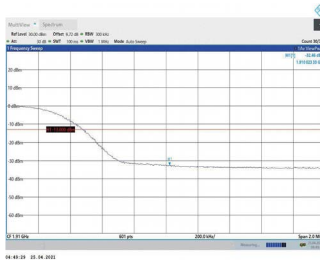
Band2-15MHz-QPSK-19125-75RB#0
