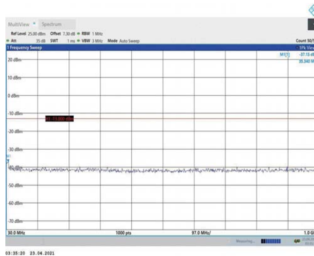
Band2-15MHz-QPSK-18675-1RB#0-Range1:30~1000MHz
