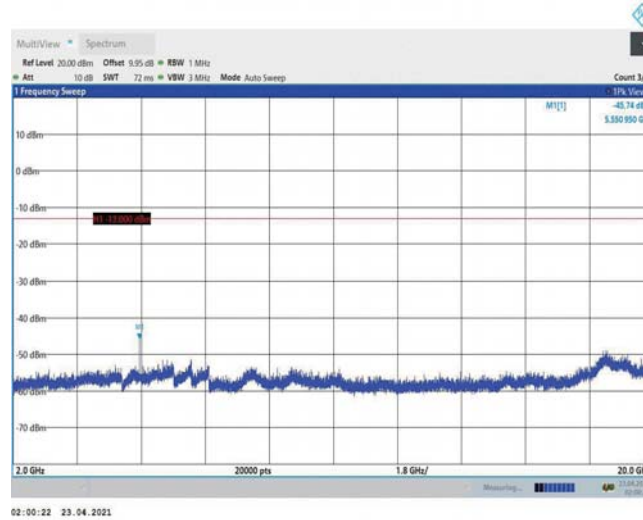
Band2-3MHz-16QAM-18615-1RB#0-Range3:2000~20000MHz
