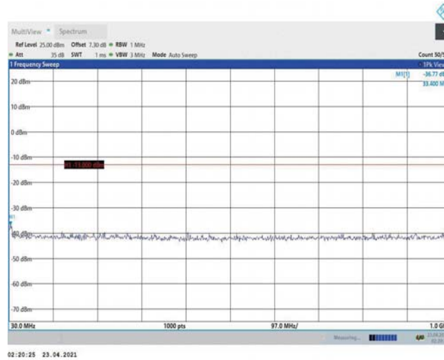
Band2-5MHz-16QAM-19175-1RB#0-Range1:30~1000MHz
