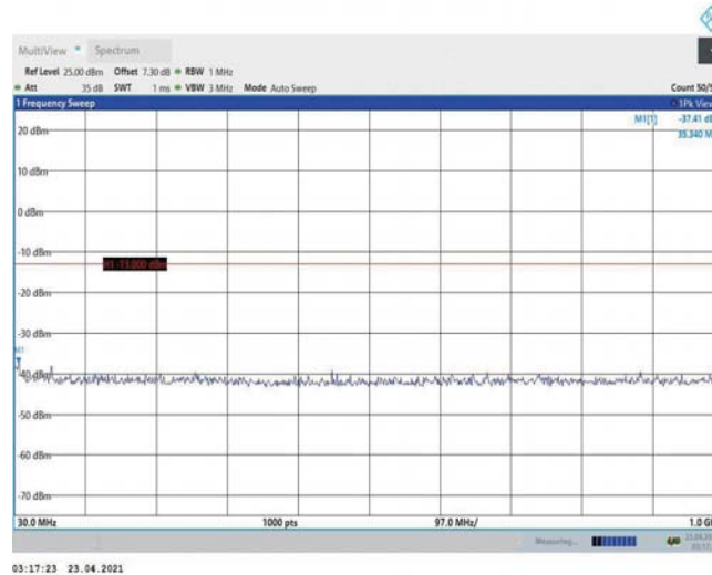
Band2-10MHz-16QAM-18650-1RB#0-Range1:30~1000MHz
