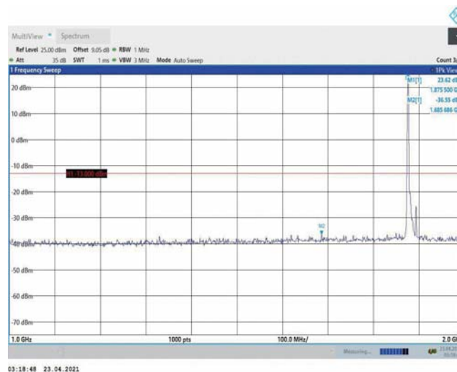
Band2-10MHz-16QAM-18900-1RB#0-Range2:1000~2000MHz
