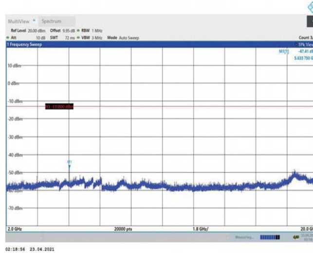
Band2-5MHz-QPSK-18900-1RB#0-Range3:2000~20000MHz
