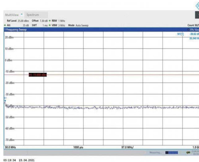
Band2-10MHz-QPSK-19150-1RB#0-Range1:30~1000MHz
