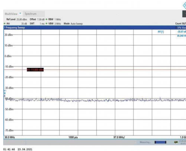
Band2-1.4MHz-16QAM-18900-1RB#0-Range1:30~1000MHz
