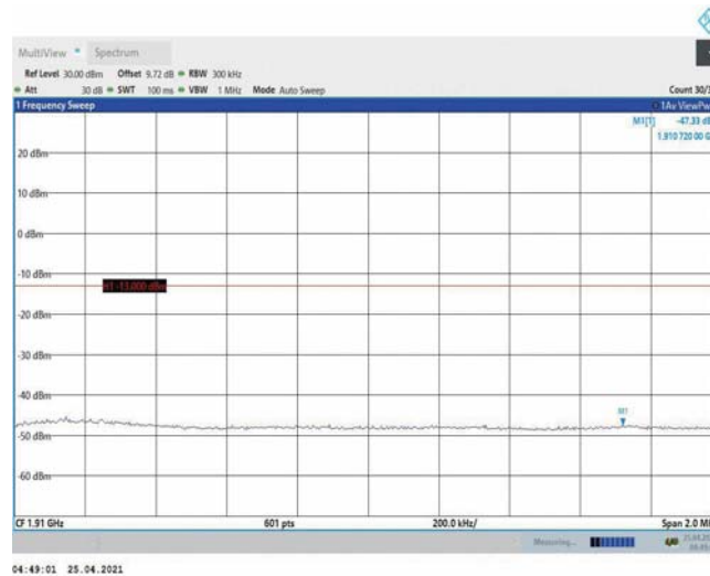
Band2-15MHz-16QAM-19125-1RB#0
