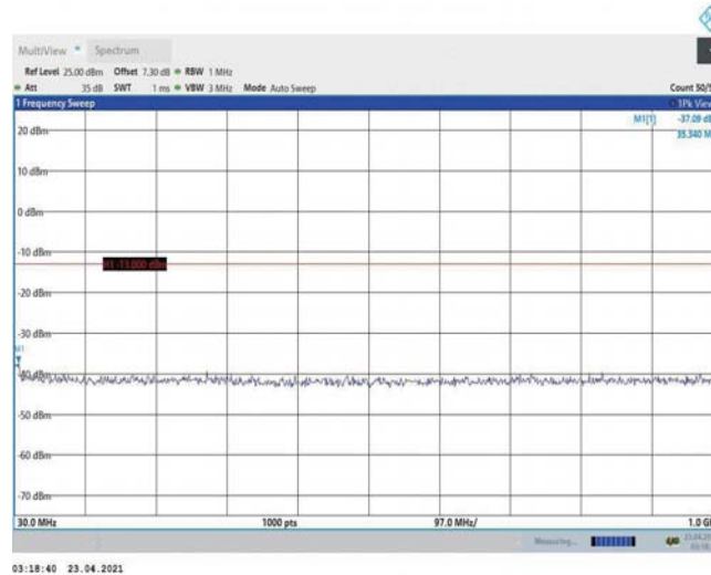
Band2-10MHz-16QAM-18900-1RB#0-Range1:30~1000MHz
