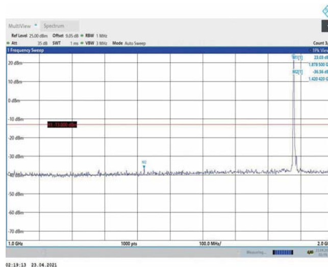
Band2-5MHz-16QAM-18900-1RB#0-Range2:1000~2000MHz
