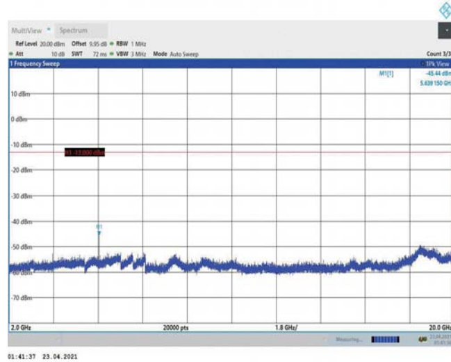
Band2-1.4MHz-QPSK-18900-1RB#0-Range3:2000~20000MHz
