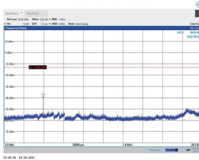
Band2-15MHz-QPSK-18675-1RB#0-Range3:2000~20000MHz
