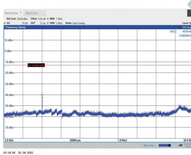
Band2-10MHz-16QAM-18900-1RB#0-Range3:2000~20000MHz
