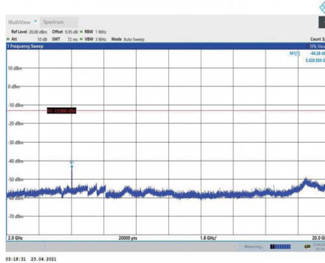
Band2-10MHz-QPSK-18900-1RB#0-Range3:2000~20000MHz
