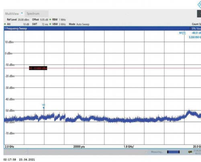
Band2-5MHz-16QAM-18625-1RB#0-Range3:2000~20000MHz
