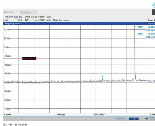
Band2-5MHz-16QAM-18625-1RB#0-Range2:1000~2000MHz
