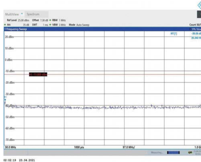
Band2-3MHz-QPSK-19185-1RB#0-Range1:30~1000MHz
