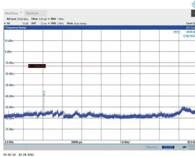
Band2-10MHz-16QAM-19150-1RB#0-Range3:2000~20000MHz
