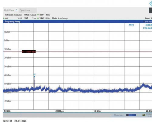
Band2-1.4MHz-QPSK-19193-1RB#0-Range3:2000~20000MHz
