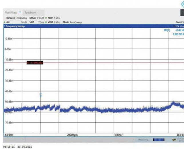
Band2-5MHz-16QAM-18900-1RB#0-Range3:2000~20000MHz
