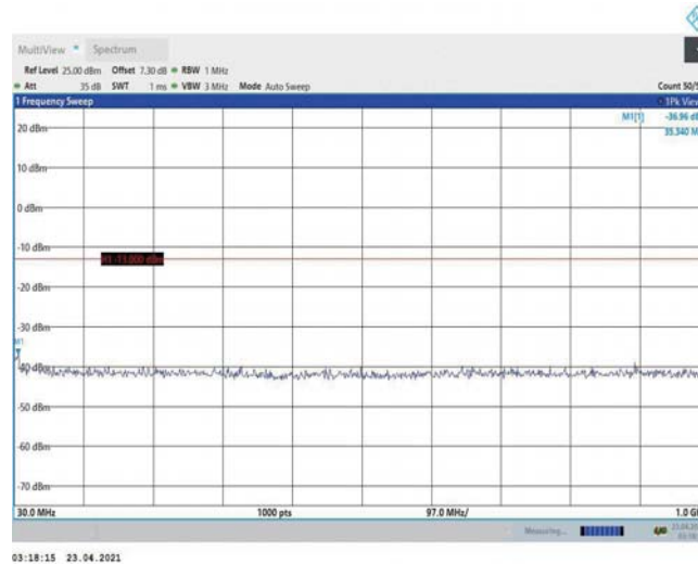
Band2-10MHz-QPSK-18900-1RB#0-Range1:30~1000MHz
