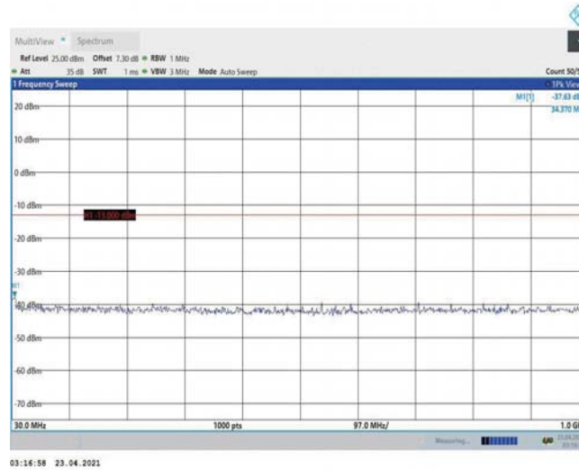
Band2-10MHz-QPSK-18650-1RB#0-Range1:30~1000MHz
