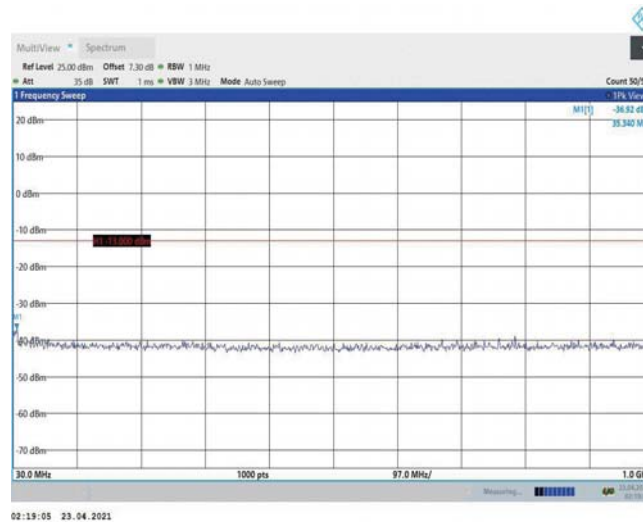
Band2-5MHz-16QAM-18900-1RB#0-Range1:30~1000MHz
