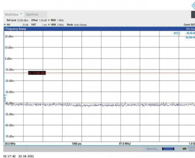
Band2-5MHz-16QAM-18625-1RB#0-Range1:30~1000MHz
