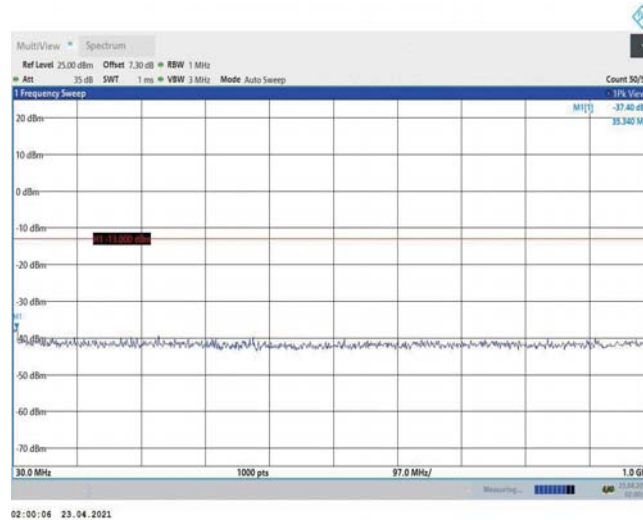
Band2-3MHz-16QAM-18615-1RB#0-Range1:30~1000MHz
