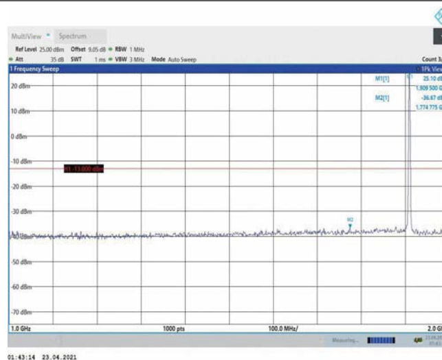
Band2-1.4MHz-16QAM-19193-1RB#0-Range2:1000~2000MHz
