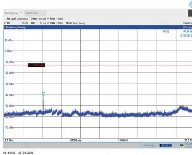
Band2-1.4MHz-16QAM-19193-1RB#0-Range3:2000~20000MHz
