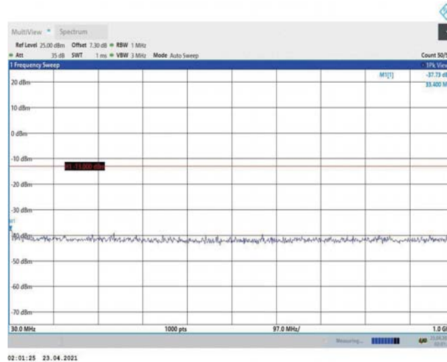
Band2-3MHz-16QAM-18900-1RB#0-Range1:30~1000MHz
