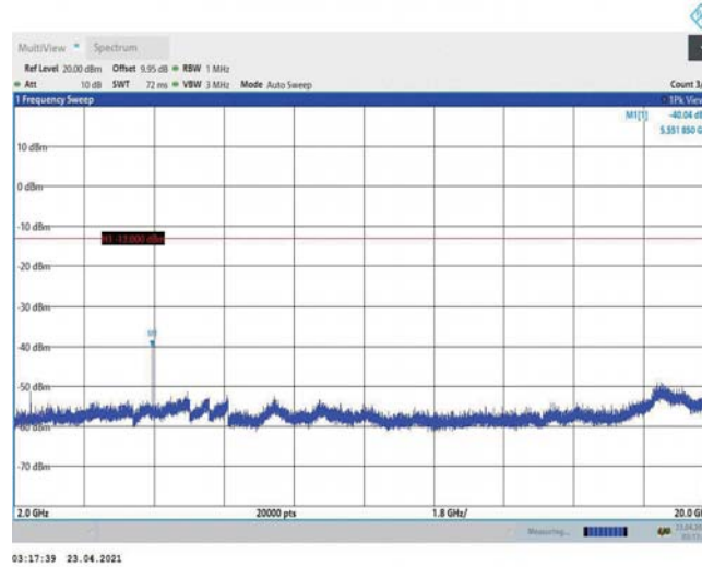
Band2-10MHz-16QAM-18650-1RB#0-Range3:2000~20000MHz
