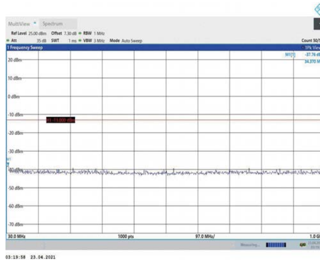
Band2-10MHz-16QAM-19150-1RB#0-Range1:30~1000MHz
