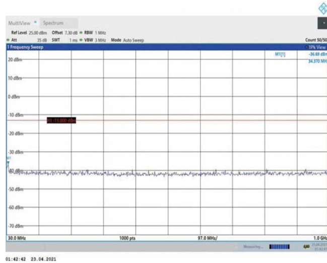
Band2-1.4MHz-QPSK-19193-1RB#0-Range1:30~1000MHz
