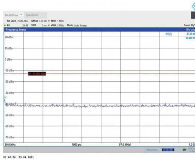
Band2-1.4MHz-16QAM-18607-1RB#0-Range1:30~1000MHz
