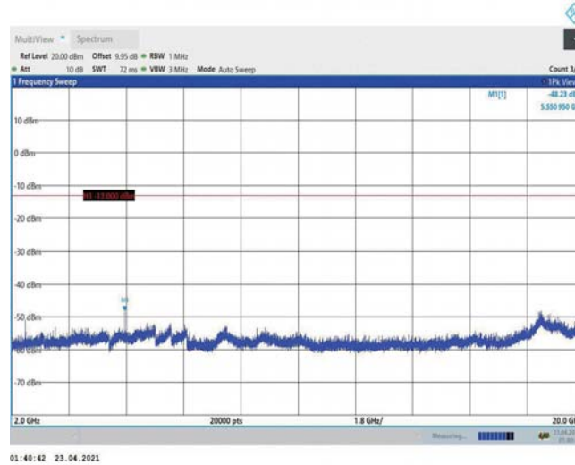
Band2-1.4MHz-16QAM-18607-1RB#0-Range3:2000~20000MHz
