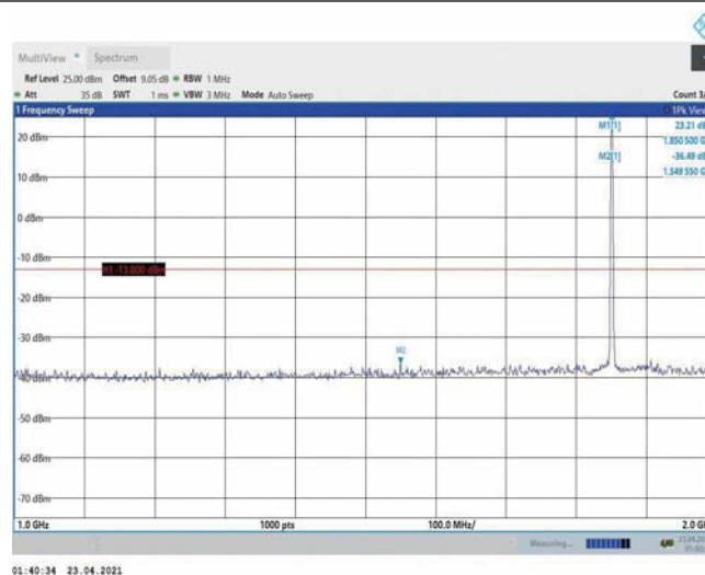
Band2-1.4MHz-16QAM-18607-1RB#0-Range2:1000~2000MHz
