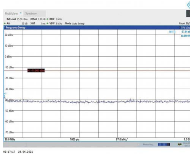
Band2-5MHz-QPSK-18625-1RB#0-Range1:30~1000MHz
