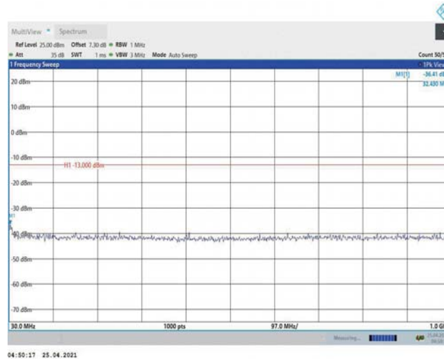
Band2-15MHz-16QAM-18675-1RB#0-Range1:30~1000MHz
