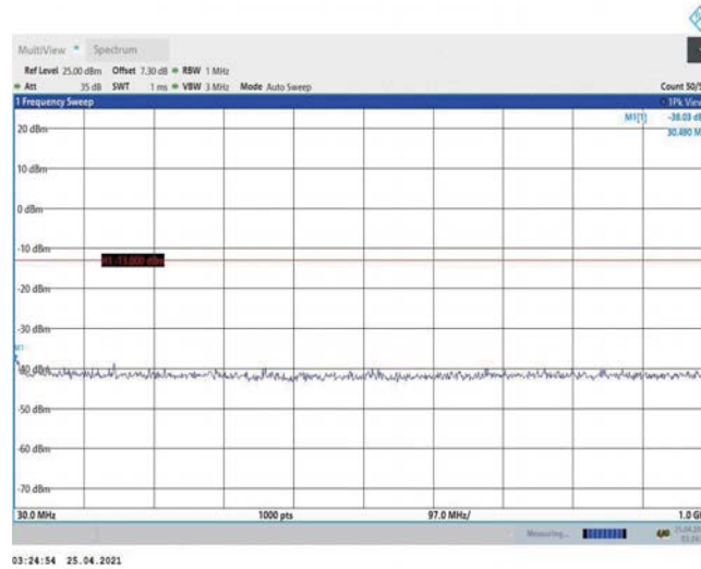
Band2-1.4MHz-QPSK-19193-1RB#0-Range1:30~1000MHz
