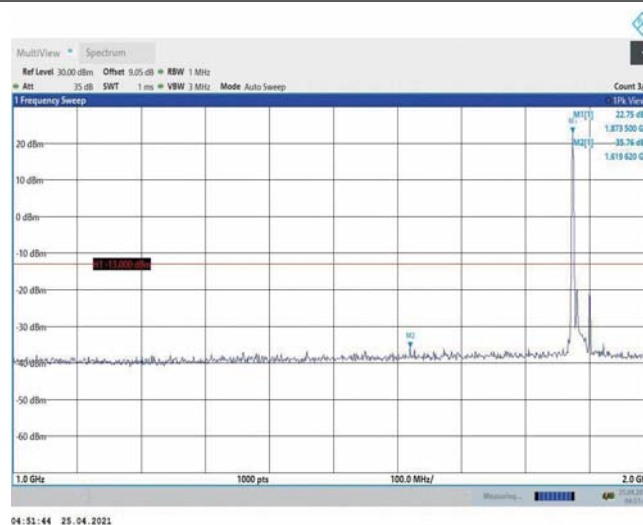
Band2-15MHz-16QAM-18900-1RB#0-Range2:1000~2000MHz
