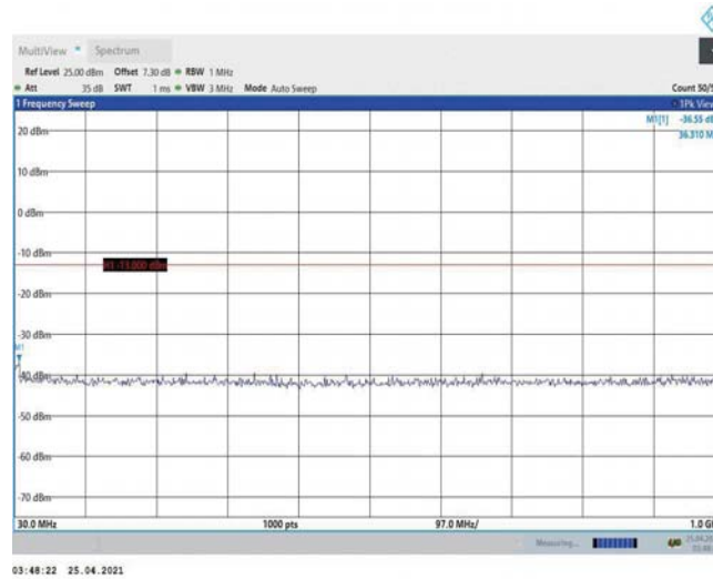
Band2-3MHz-16QAM-18900-1RB#0-Range1:30~1000MHz
