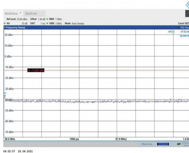
Band2-5MHz-16QAM-18625-1RB#0-Range1:30~1000MHz
