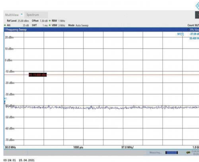
Band2-1.4MHz-QPSK-18900-1RB#0-Range1:30~1000MHz
