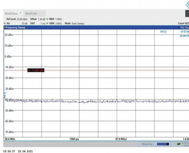
Band2-15MHz-16QAM-18900-1RB#0-Range1:30~1000MHz
