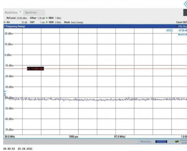
Band2-15MHz-QPSK-18675-1RB#0-Range1:30~1000MHz
