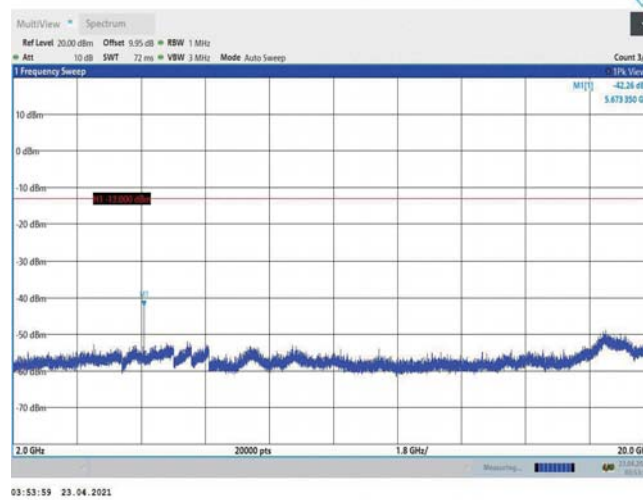
Band2-20MHz-16QAM-19100-1RB#0-Range3:2000~20000MHz
