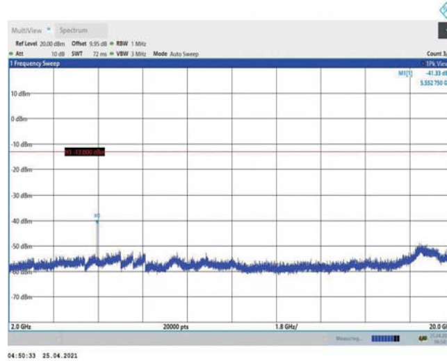
Band2-15MHz-16QAM-18675-1RB#0-Range3:2000~20000MHz
