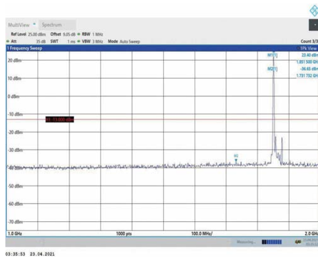
Band2-15MHz-16QAM-18675-1RB#0-Range2:1000~2000MHz
