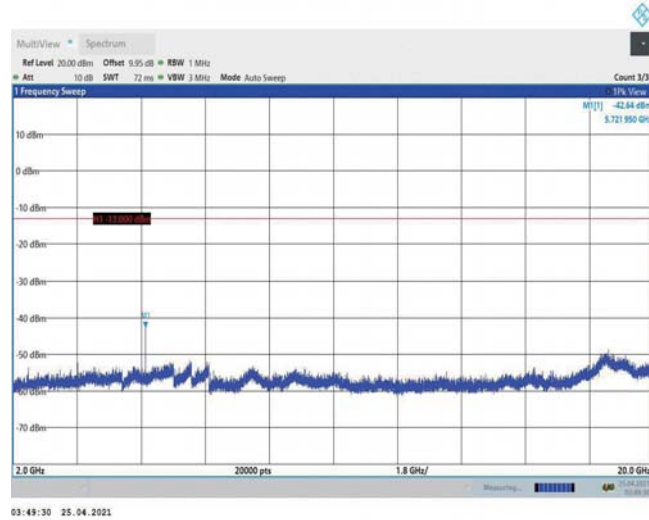
Band2-3MHz-16QAM-19185-1RB#0-Range3:2000~20000MHz
