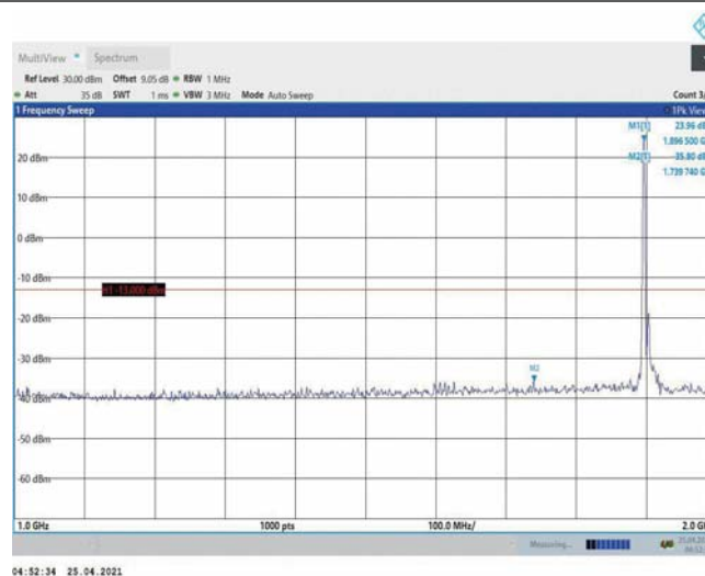
Band2-15MHz-16QAM-19125-1RB#0-Range2:1000~2000MHz
