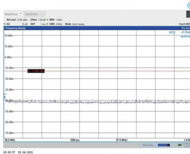
Band2-20MHz-QPSK-19100-1RB#0-Range1:30~1000MHz
