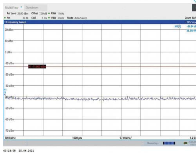
Band2-1.4MHz-QPSK-18607-1RB#0-Range1:30~1000MHz
