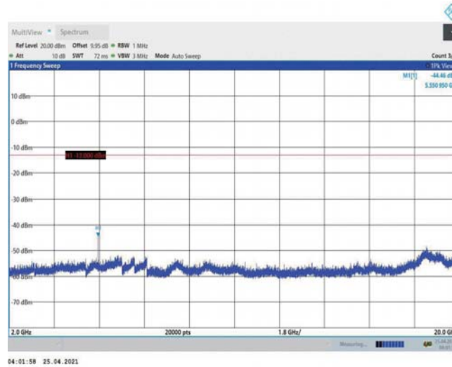
Band2-5MHz-QPSK-18625-1RB#0-Range3:2000~20000MHz
