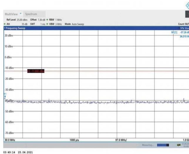
Band2-3MHz-16QAM-19185-1RB#0-Range1:30~1000MHz
