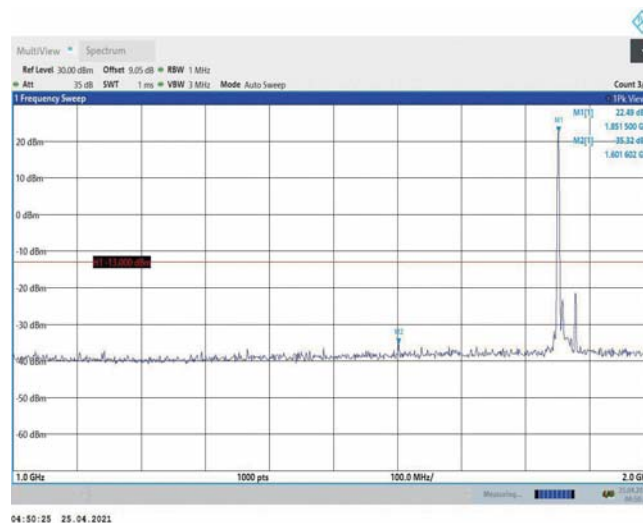
Band2-15MHz-16QAM-18675-1RB#0-Range2:1000~2000MHz
