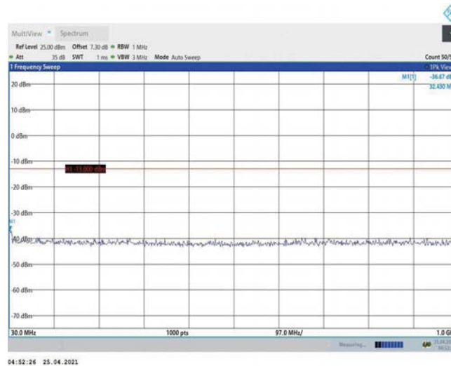
Band2-15MHz-16QAM-19125-1RB#0-Range1:30~1000MHz
