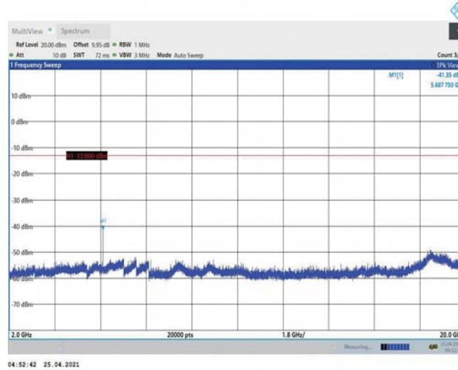
Band2-15MHz-16QAM-19125-1RB#0-Range3:2000~20000MHz
