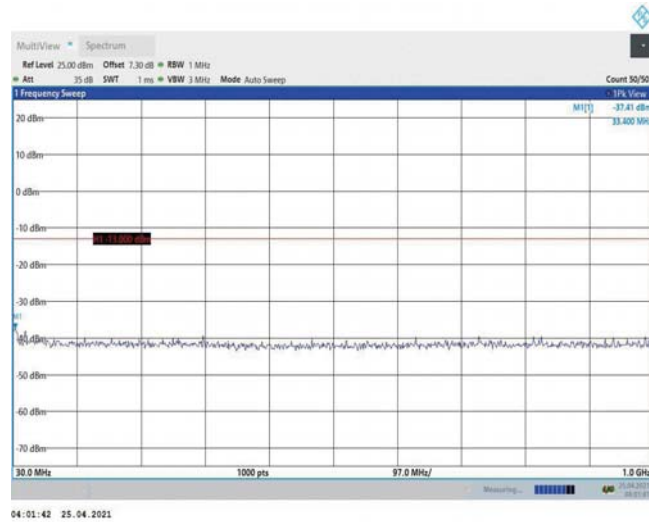
Band2-5MHz-QPSK-18625-1RB#0-Range1:30~1000MHz
