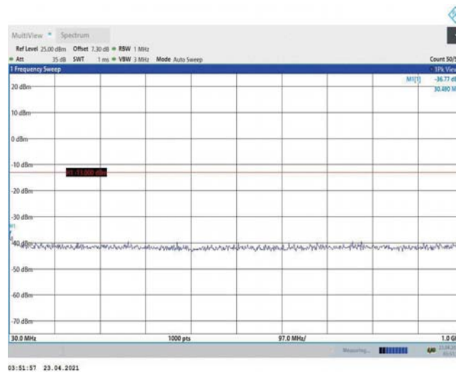
Band2-20MHz-16QAM-18700-1RB#0-Range1:30~1000MHz
