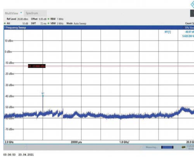
Band2-15MHz-16QAM-18900-1RB#0-Range3:2000~20000MHz
