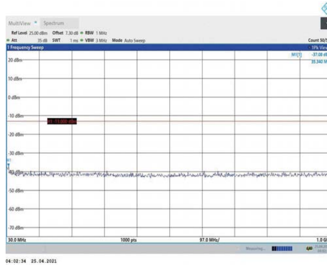
Band2-5MHz-QPSK-18900-1RB#0-Range1:30~1000MHz
