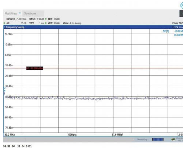
Band2-15MHz-16QAM-18900-1RB#0-Range1:30~1000MHz
