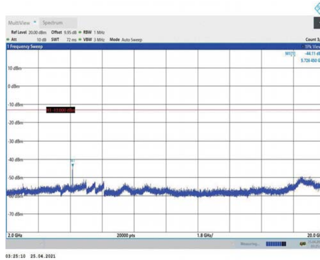
Band2-1.4MHz-QPSK-19193-1RB#0-Range3:2000~20000MHz
