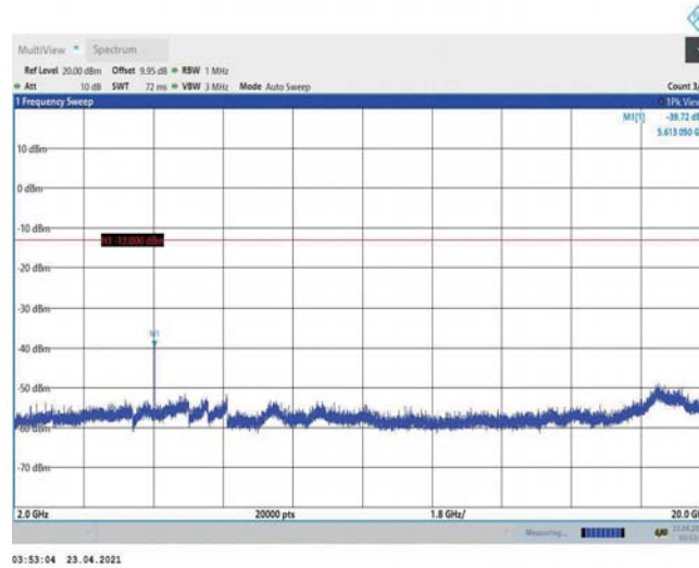
Band2-20MHz-16QAM-18900-1RB#0-Range3:2000~20000MHz
