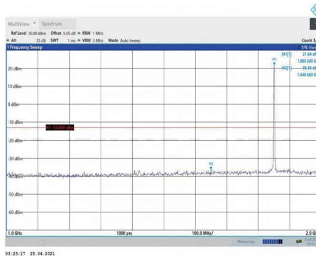
Band2-1.4MHz-QPSK-18607-1RB#0-Range2:1000~2000MHz
