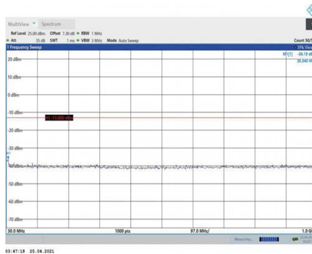
Band2-3MHz-16QAM-18615-1RB#0-Range1:30~1000MHz
