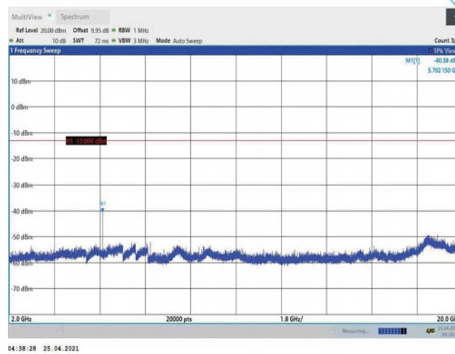
Band2-10MHz-16QAM-19150-1RB#0-Range3:2000~20000MHz
