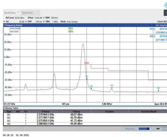
Band7-15MHz-16QAM-21375-1RB#74
