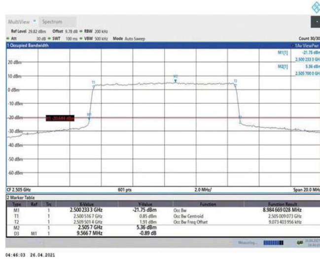
Band7-10MHz-16QAM-20800-50RB#0-8.985
