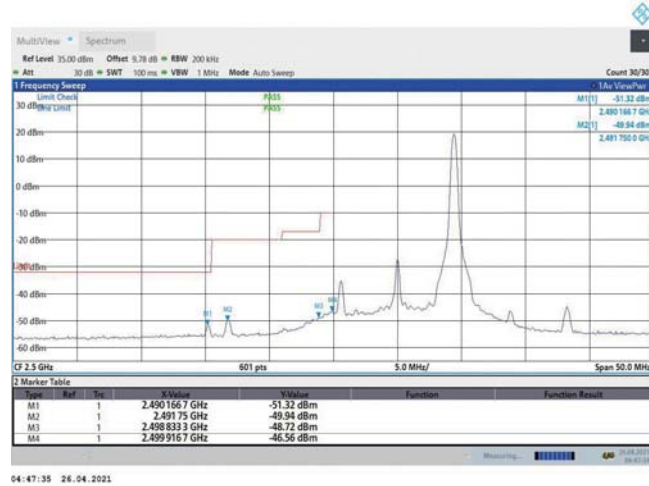
Band7-10MHz-QPSK-20800-1RB#49
