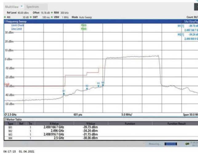
Band7-15MHz-16QAM-20825-75RB#0
