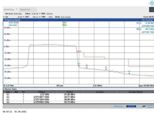
Band7-10MHz-16QAM-21400-50RB#0
