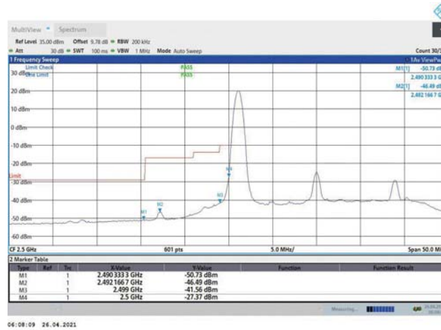
Band7-20MHz-QPSK-20850-1RB#0
