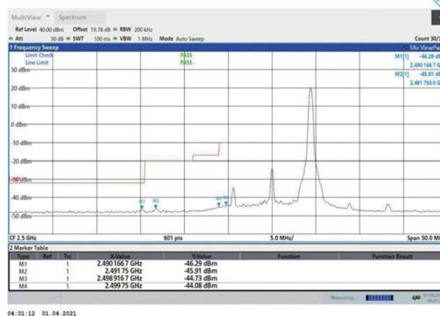
Band7-10MHz-QPSK-20800-1RB#49
