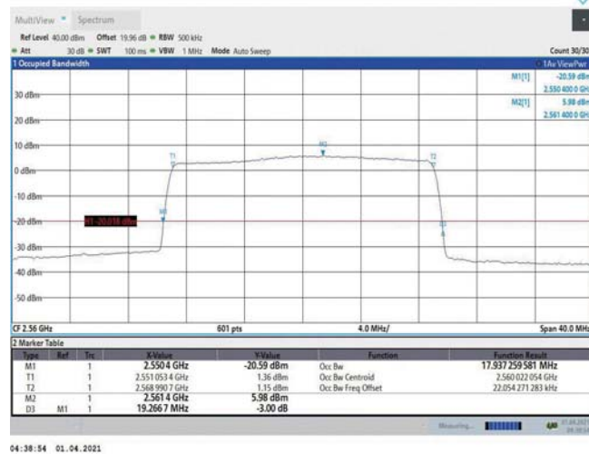
Band7-20MHz-16QAM-21350-100RB#0-17.937
