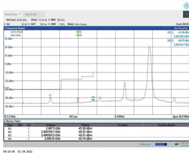
Band7-15MHz-QPSK-20825-1RB#74
