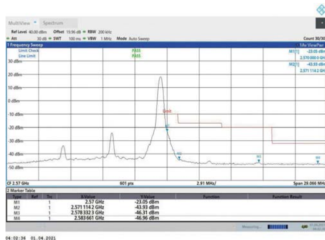
Band7-10MHz-QPSK-21400-1RB#49
