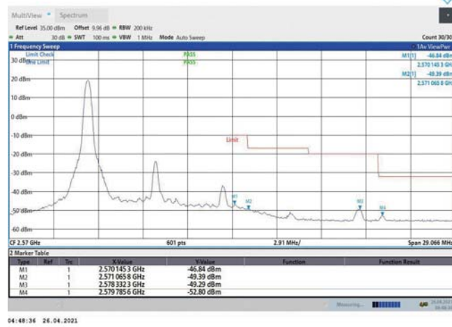
Band7-10MHz-QPSK-21400-1RB#0
