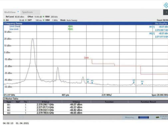
Band7-10MHz-QPSK-21400-1RB#0
