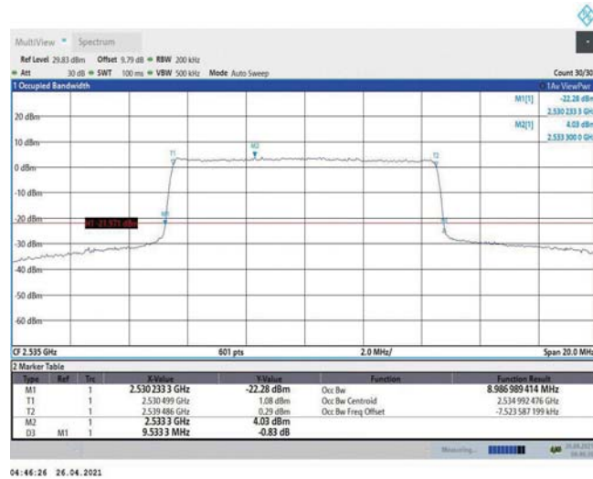
Band7-10MHz-16QAM-21100-50RB#0-8.987
