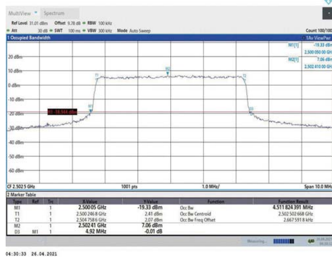
Band7-5MHz-QPSK-20775-25RB#0-4.512
