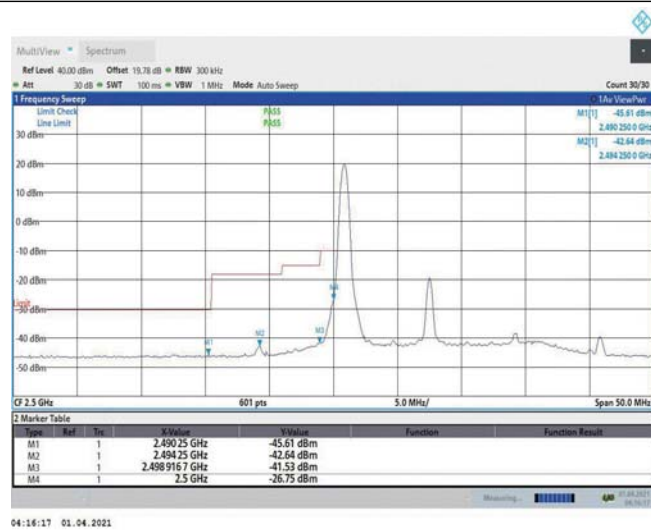
Band7-15MHz-QPSK-20825-1RB#0
