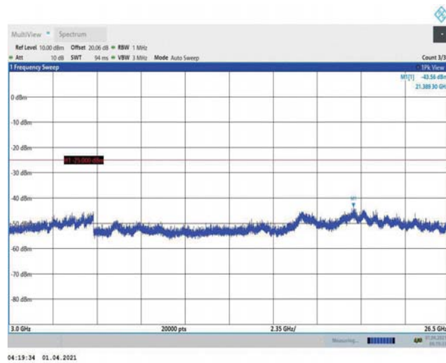
Band7-15MHz-16QAM-20825-1RB#0-Range3:3000~26500MHz
