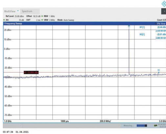
Band7-5MHz-16QAM-21100-1RB#0-Range2:1000~3000MHz
