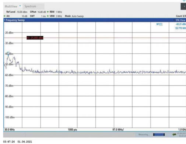
Band7-5MHz-16QAM-21100-1RB#0-Range1:30~1000MHz
