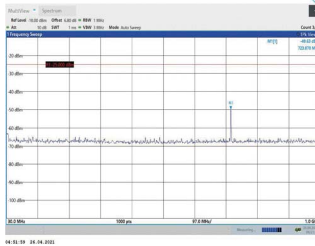
Band7-10MHz-16QAM-21400-1RB#0-Range1:30~1000MHz
