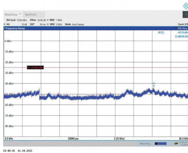
Band7-5MHz-16QAM-21425-1RB#0-Range3:3000~26500MHz
