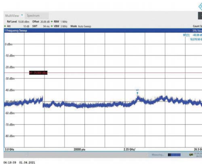
Band7-15MHz-QPSK-20825-1RB#0-Range3:3000~26500MHz
