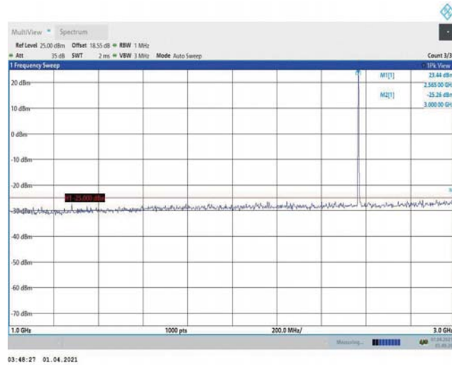
Band7-5MHz-16QAM-21425-1RB#0-Range2:1000~3000MHz
