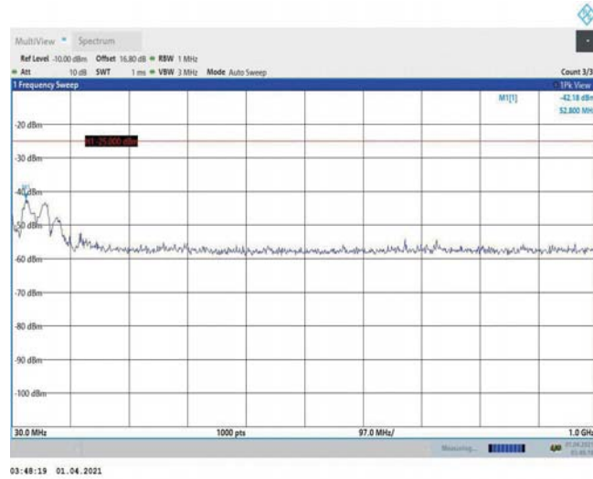
Band7-5MHz-16QAM-21425-1RB#0-Range1:30~1000MHz
