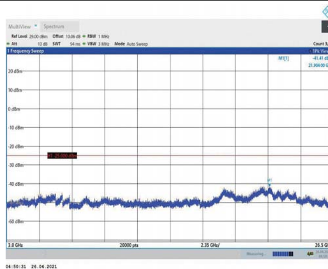
Band7-10MHz-16QAM-20800-1RB#0-Range3:3000~26500MHz
