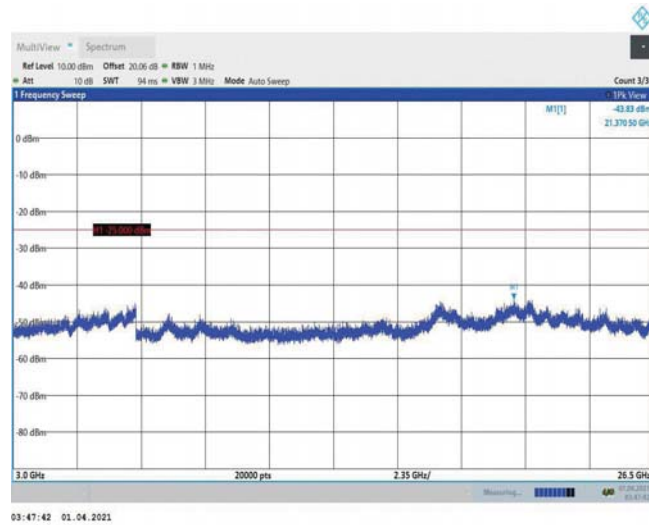
Band7-5MHz-16QAM-21100-1RB#0-Range3:3000~26500MHz
