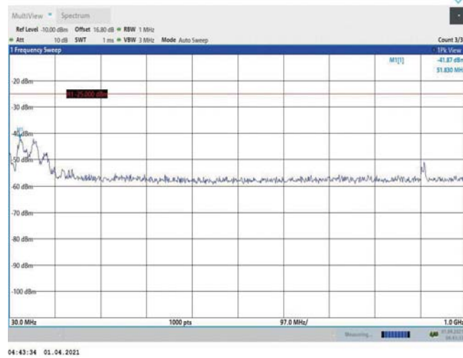
Band7-20MHz-QPSK-21350-1RB#0-Range1:30~1000MHz
