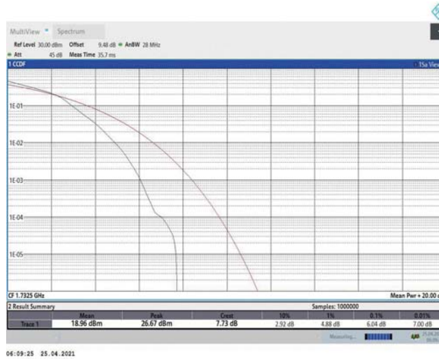
Band4-1.4MHz-16QAM-20175-6RB#0
