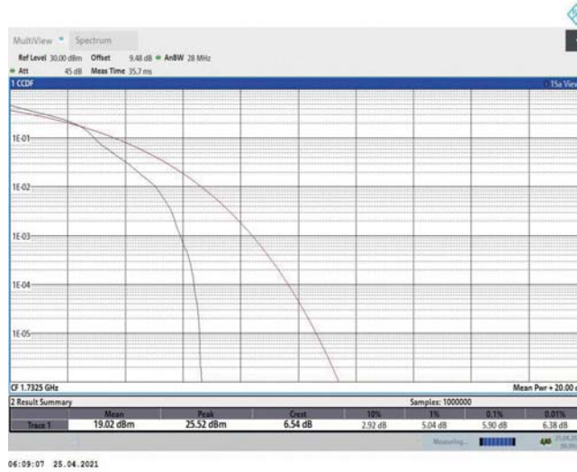
Band4-1.4MHz-16QAM-20175-1RB#0
