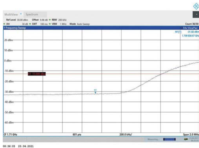
Band4-20MHz-16QAM-20050-100RB#0
