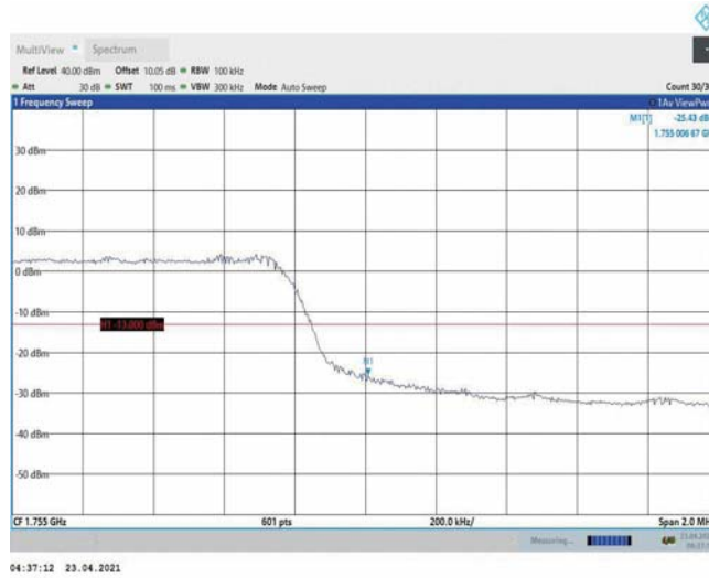
Band4-5MHz-16QAM-20375-25RB#0
