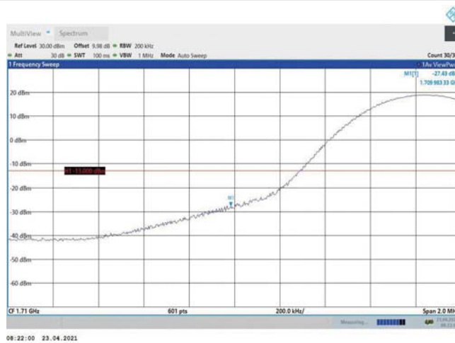
Band4-15MHz-QPSK-20025-1RB#0
