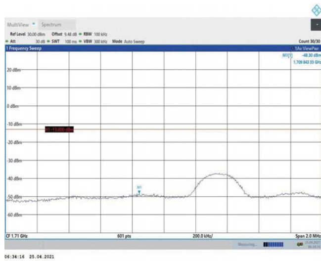
Band4-5MHz-16QAM-19975-1RB#24
