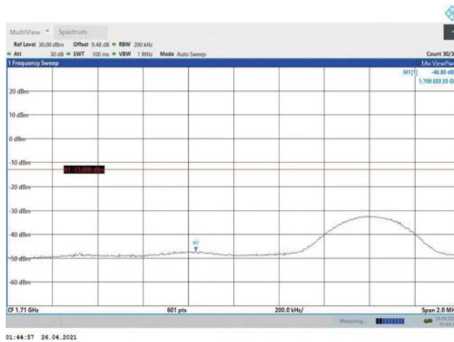
Band4-10MHz-QPSK-20000-1RB#49
