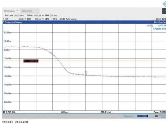
Band4-10MHz-16QAM-20350-50RB#0
