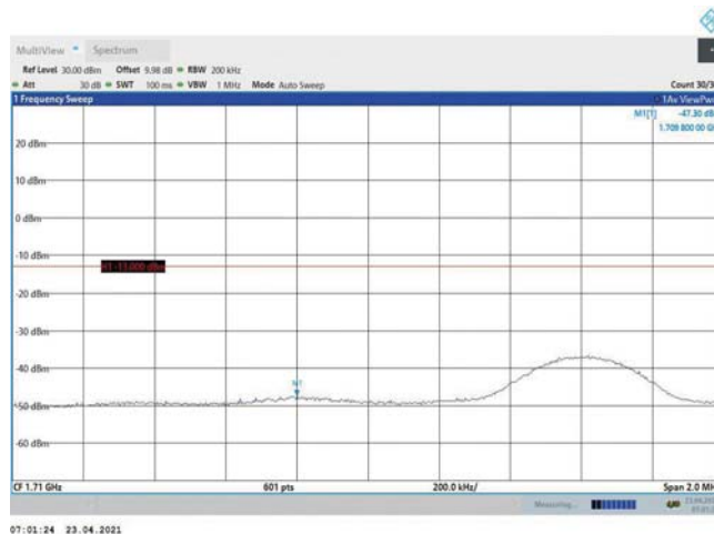
Band4-10MHz-QPSK-20000-1RB#49
