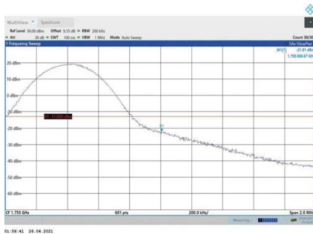
Band4-10MHz-16QAM-20350-1RB#49
