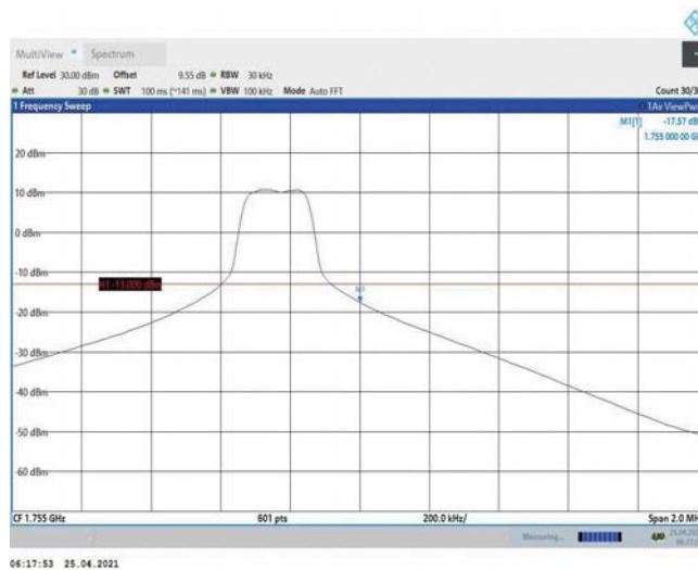
Band4-3MHz-16QAM-20385-1RB#14
