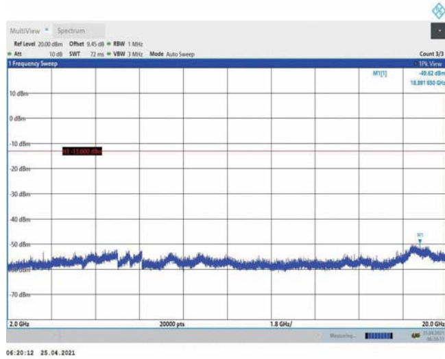
Band4-3MHz-16QAM-20175-1RB#0-Range3:2000~20000MHz
