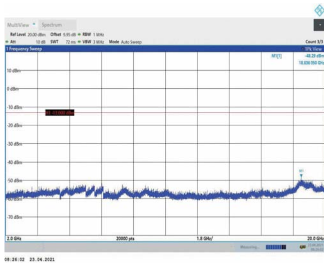
Band4-15MHz-QPSK-20325-1RB#0-Range3:2000~20000MHz
