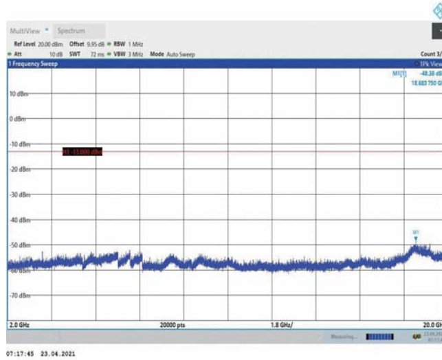
Band4-10MHz-16QAM-20000-1RB#0-Range3:2000~20000MHz
