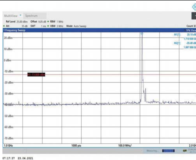
Band4-10MHz-16QAM-20000-1RB#0-Range2:1000~2000MHz
