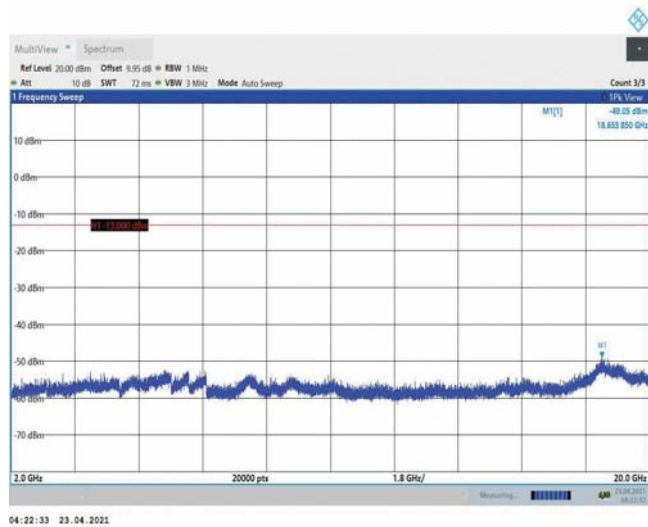
Band4-3MHz-QPSK-20175-1RB#0-Range3:2000~20000MHz
