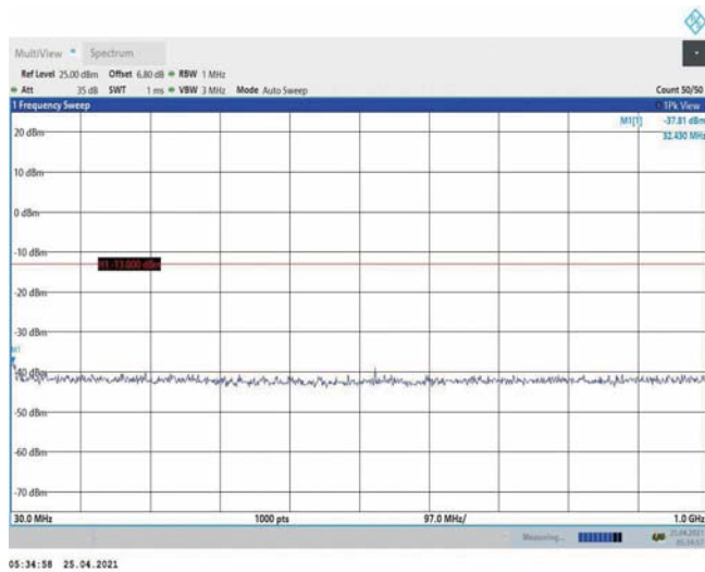
Band4-1.4MHz-QPSK-19957-1RB#0-Range1:30~1000MHz
