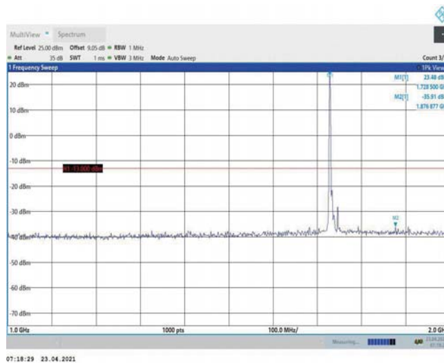
Band4-10MHz-16QAM-20175-1RB#0-Range2:1000~2000MHz
