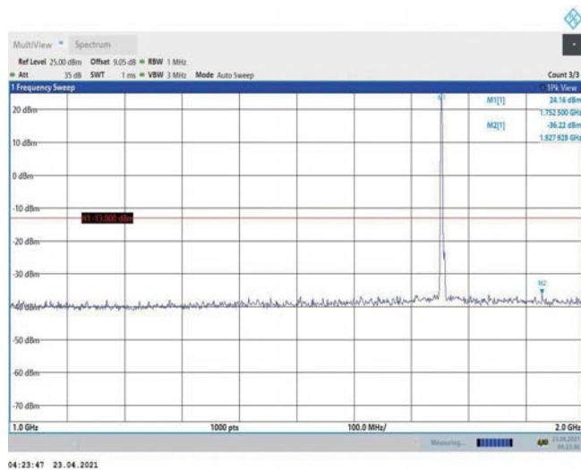
Band4-3MHz-16QAM-20385-1RB#0-Range2:1000~2000MHz
