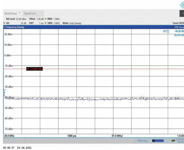
Band4-20MHz-16QAM-20175-1RB#0-Range1:30~1000MHz
