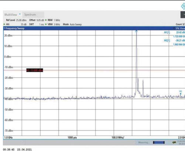
Band4-20MHz-16QAM-20175-1RB#0-Range2:1000~2000MHz
