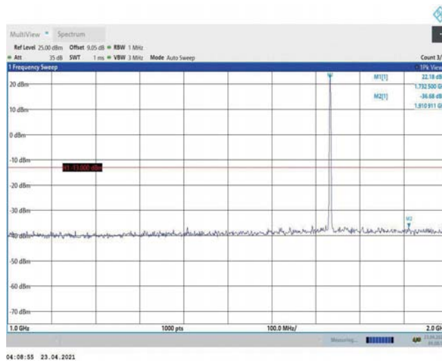
Band4-1.4MHz-16QAM-20175-1RB#0-Range2:1000~2000MHz
