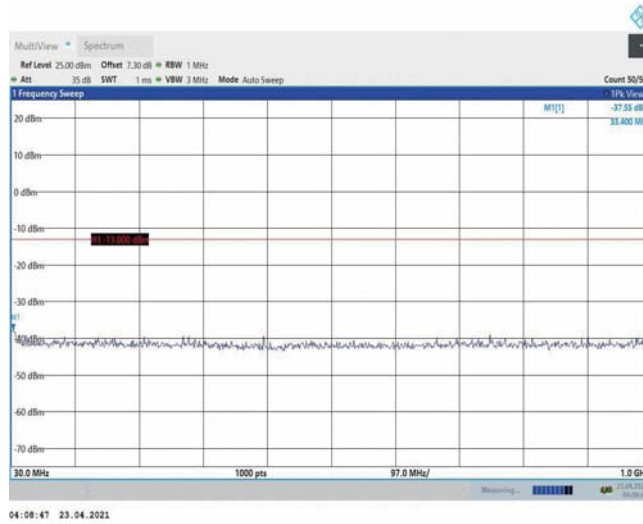
Band4-1.4MHz-16QAM-20175-1RB#0-Range1:30~1000MHz
