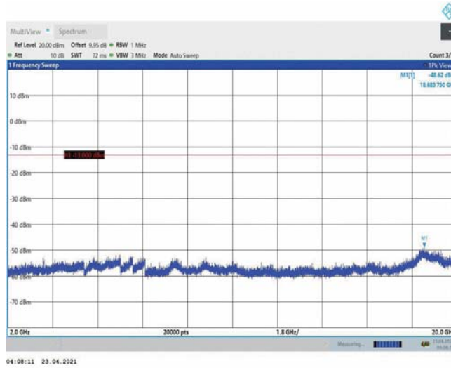
Band4-1.4MHz-16QAM-19957-1RB#0-Range3:2000~20000MHz
