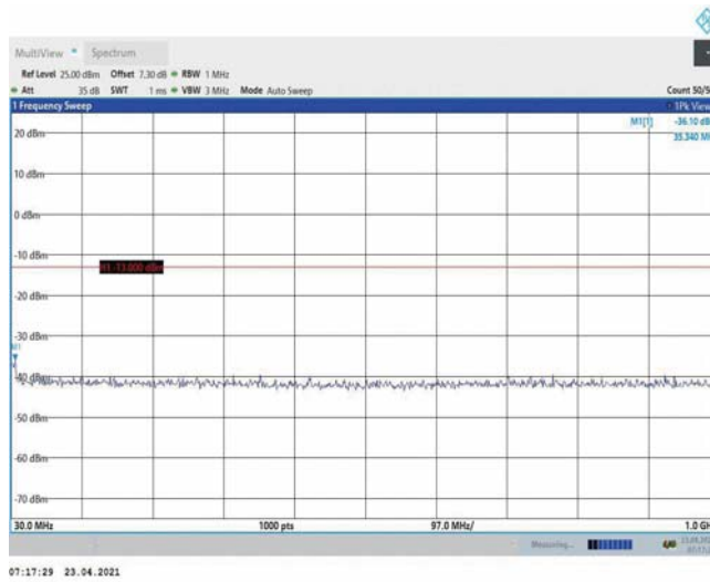
Band4-10MHz-16QAM-20000-1RB#0-Range1:30~1000MHz
