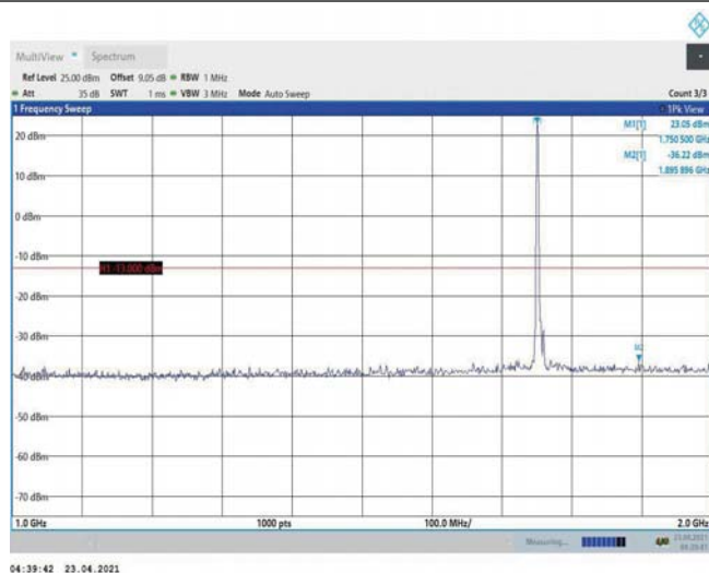
Band4-5MHz-16QAM-20375-1RB#0-Range2:1000~2000MHz
