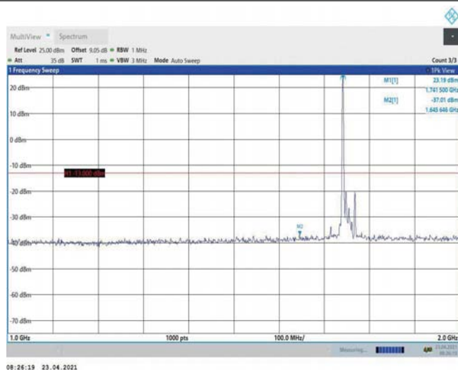
Band4-15MHz-16QAM-20325-1RB#0-Range2:1000~2000MHz
