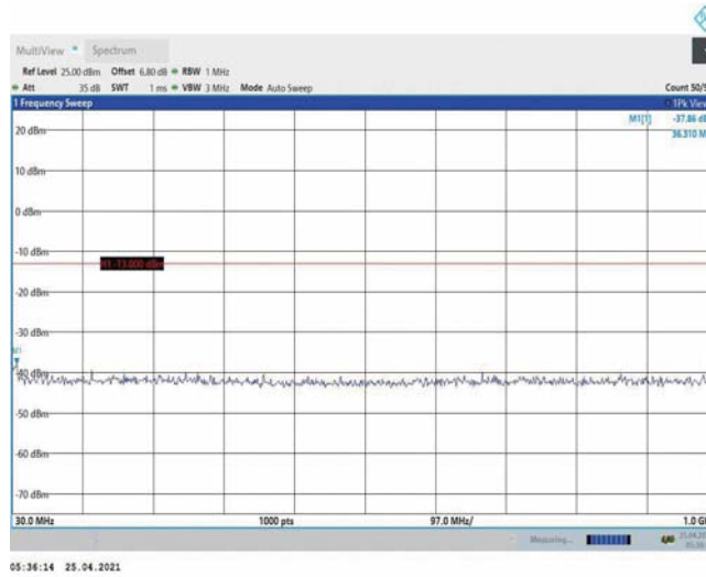
Band4-1.4MHz-16QAM-20175-1RB#0-Range1:30~1000MHz
