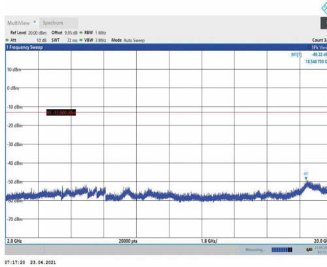
Band4-10MHz-QPSK-20000-1RB#0-Range3:2000~20000MHz
