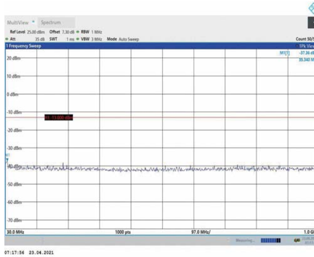
Band4-10MHz-QPSK-20175-1RB#0-Range1:30~1000MHz
