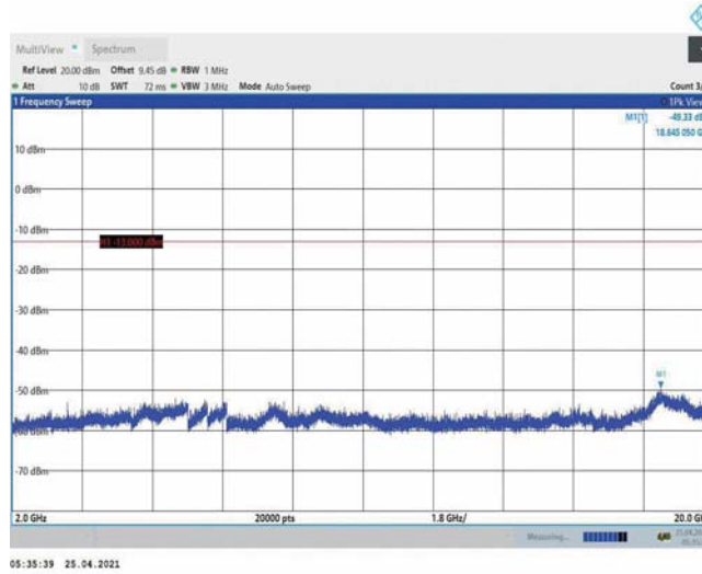
Band4-1.4MHz-16QAM-19957-1RB#0-Range3:2000~20000MHz
