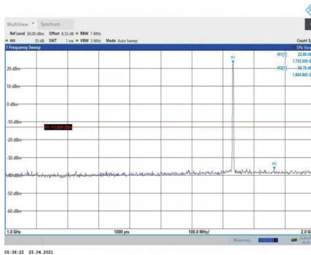
Band4-1.4MHz-16QAM-20175-1RB#0-Range2:1000~2000MHz
