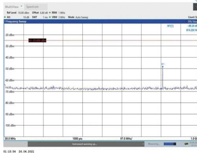
Band38-15MHz-16QAM-38175-1RB#0-Range1:30~1000MHz
