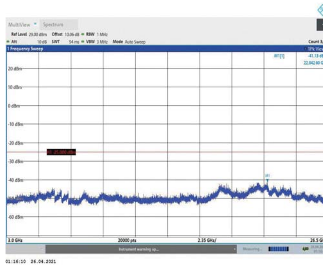
Band38-15MHz-16QAM-38175-1RB#0-Range3:3000~26500MHz
