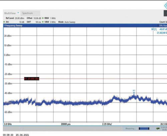
Band38-5MHz-QPSK-38000-1RB#0-Range3:3000~26500MHz
