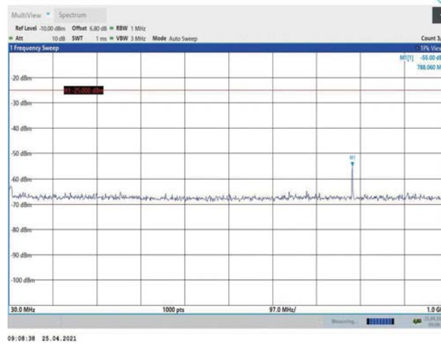
Band38-5MHz-16QAM-38000-1RB#0-Range1:30~1000MHz
