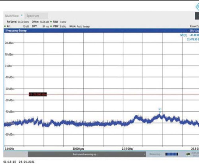
Band38-15MHz-QPSK-37825-1RB#0-Range3:3000~26500MHz
