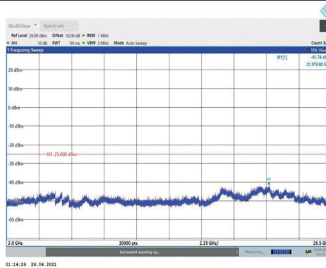
Band38-15MHz-QPSK-38000-1RB#0-Range3:3000~26500MHz
