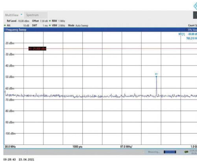
Band38-10MHz-16QAM-38000-1RB#0-Range1:30~1000MHz
