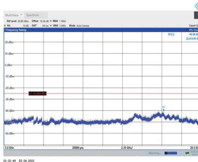
Band38-20MHz-16QAM-37850-1RB#0-Range3:3000~26500MHz
