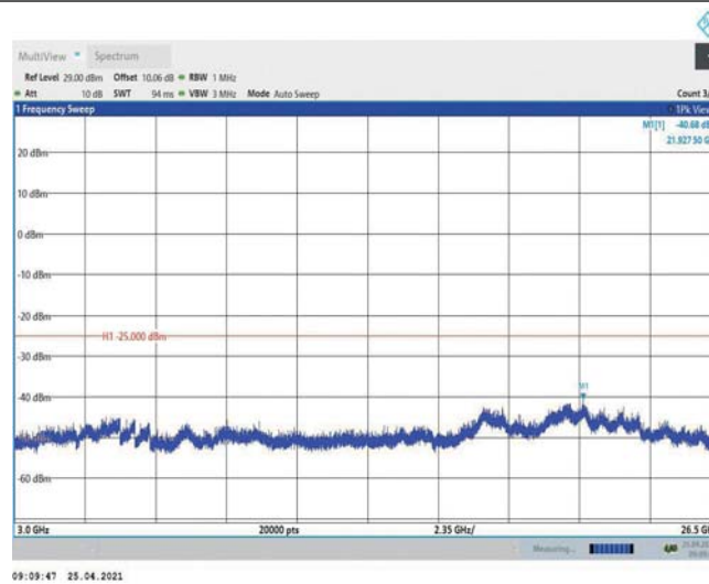
Band38-5MHz-16QAM-38225-1RB#0-Range3:3000~26500MHz
