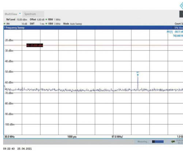
Band38-10MHz-QPSK-37800-1RB#0-Range1:30~1000MHz
