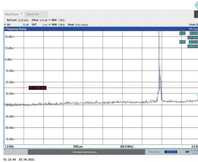
Band38-15MHz-16QAM-37825-1RB#0-Range2:1000~3000MHz
