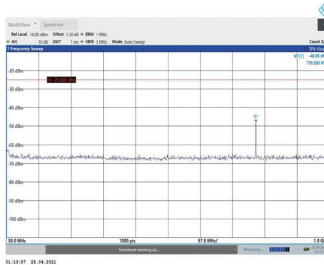
Band38-15MHz-16QAM-38000-1RB#0-Range1:30~1000MHz
