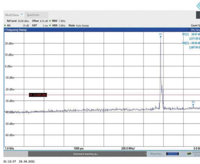
Band38-15MHz-QPSK-37825-1RB#0-Range2:1000~3000MHz
