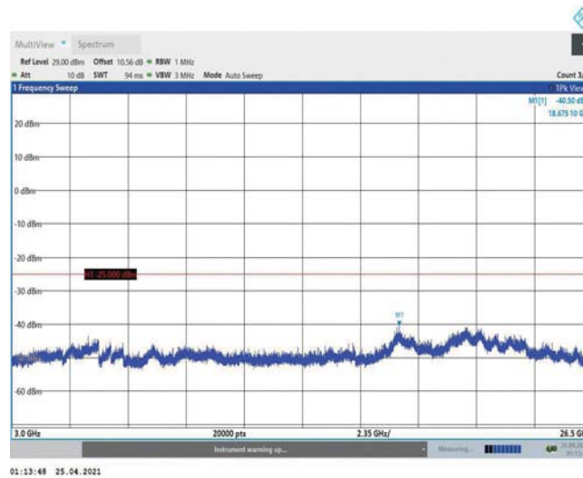
Band38-15MHz-QPSK-38000-1RB#0-Range3:3000~26500MHz
