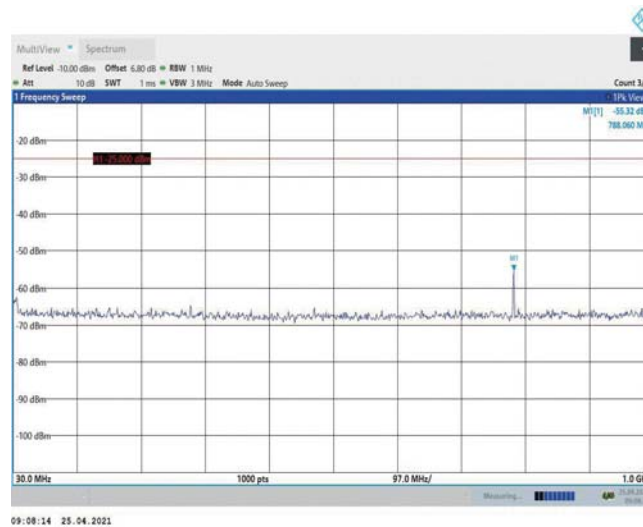
Band38-5MHz-QPSK-38000-1RB#0-Range1:30~1000MHz
