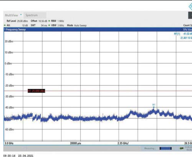
Band38-10MHz-16QAM-38200-1RB#0-Range3:3000~26500MHz
