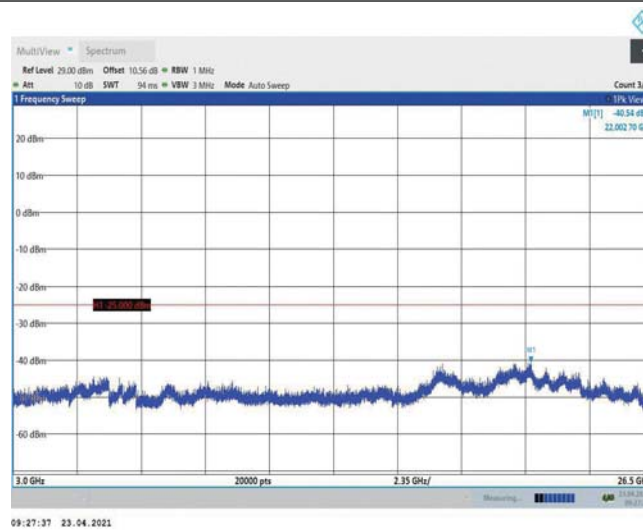
Band38-10MHz-16QAM-37800-1RB#0-Range3:3000~26500MHz
