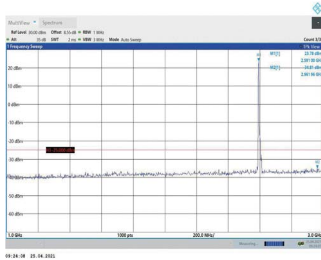
Band38-10MHz-16QAM-38000-1RB#0-Range2:1000~3000MHz
