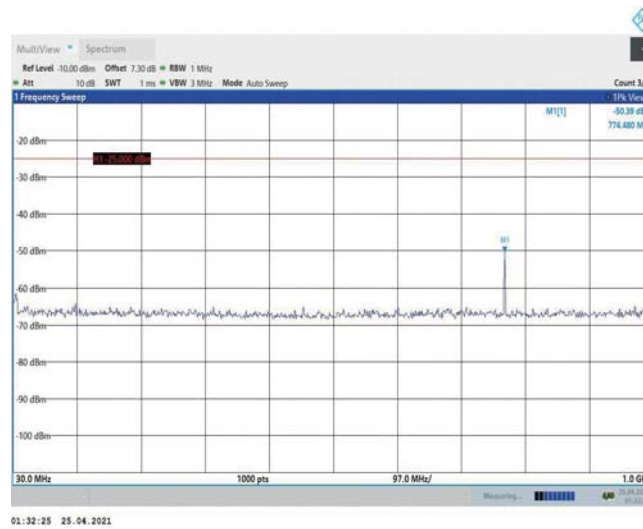
Band38-20MHz-16QAM-38000-1RB#0-Range1:30~1000MHz
