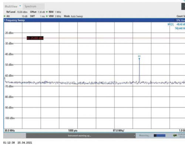
Band38-15MHz-16QAM-37825-1RB#0-Range1:30~1000MHz
