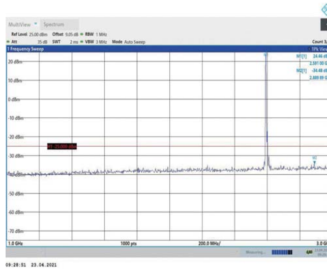
Band38-10MHz-16QAM-38000-1RB#0-Range2:1000~3000MHz
