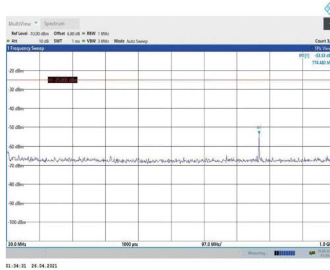
Band38-20MHz-QPSK-38000-1RB#0-Range1:30~1000MHz
