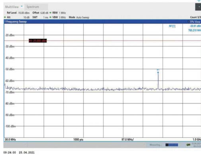
Band38-10MHz-16QAM-38000-1RB#0-Range1:30~1000MHz
