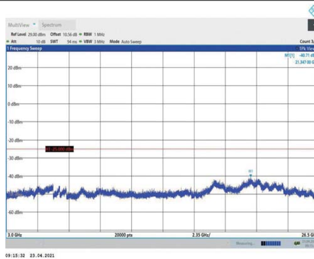
Band38-5MHz-16QAM-38000-1RB#0-Range3:3000~26500MHz
