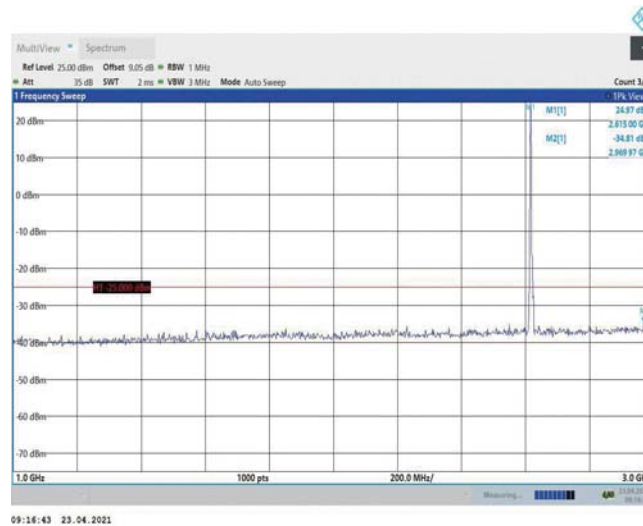
Band38-5MHz-16QAM-38225-1RB#0-Range2:1000~3000MHz
