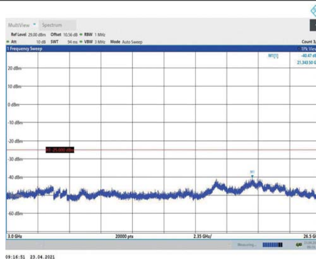
Band38-5MHz-16QAM-38225-1RB#0-Range3:3000~26500MHz
