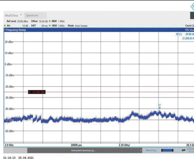
Band38-15MHz-16QAM-38000-1RB#0-Range3:3000~26500MHz
