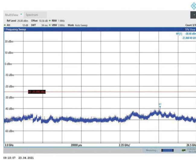
Band38-5MHz-QPSK-38000-1RB#0-Range3:3000~26500MHz
