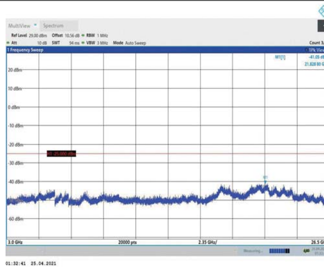
Band38-20MHz-16QAM-38000-1RB#0-Range3:3000~26500MHz
