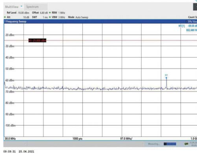
Band38-5MHz-16QAM-38225-1RB#0-Range1:30~1000MHz
