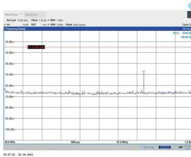
Band38-10MHz-16QAM-37800-1RB#0-Range1:30~1000MHz
