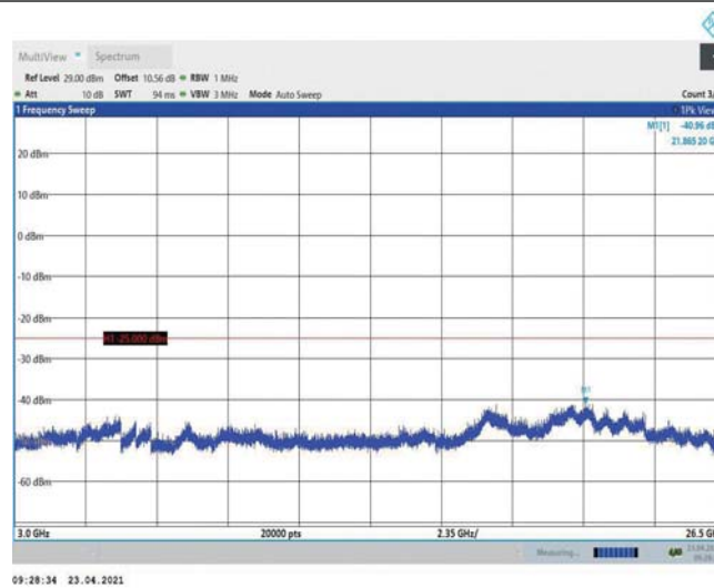
Band38-10MHz-QPSK-38000-1RB#0-Range3:3000~26500MHz
