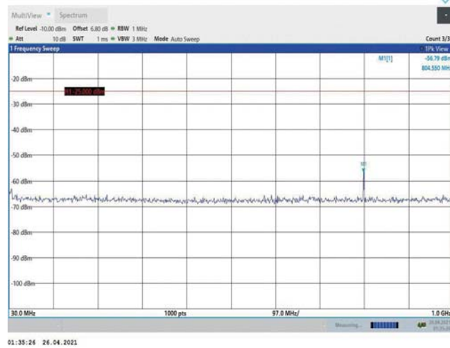
Band38-20MHz-QPSK-38150-1RB#0-Range1:30~1000MHz
