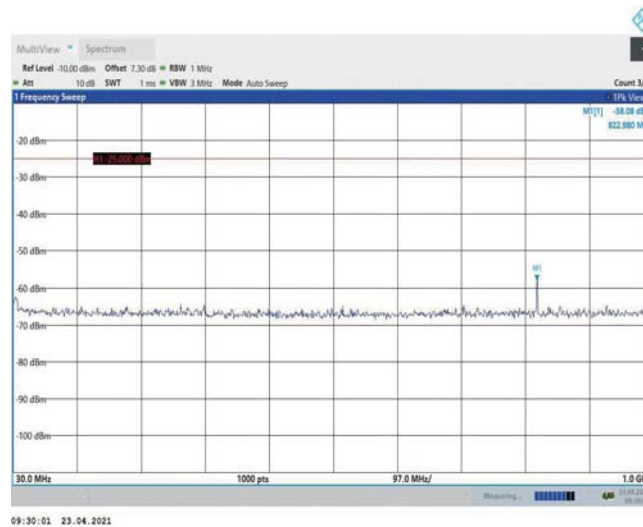
Band38-10MHz-16QAM-38200-1RB#0-Range1:30~1000MHz
