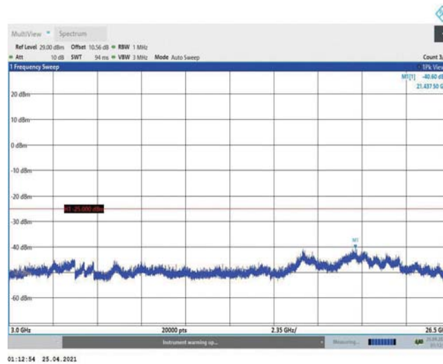
Band38-15MHz-16QAM-37825-1RB#0-Range3:3000~26500MHz
