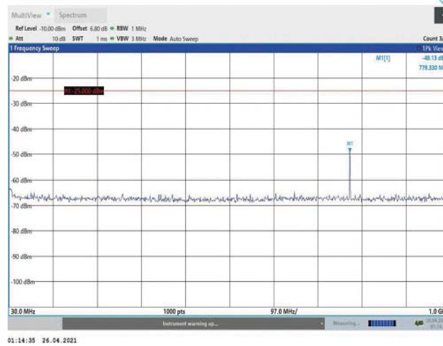
Band38-15MHz-16QAM-38000-1RB#0-Range1:30~1000MHz
