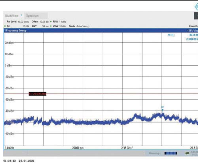
Band38-20MHz-QPSK-38150-1RB#0-Range3:3000~26500MHz
