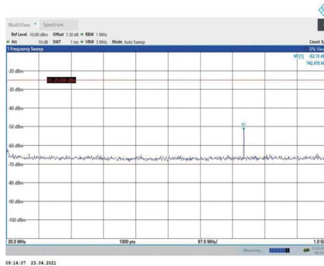
Band38-5MHz-16QAM-37775-1RB#0-Range1:30~1000MHz
