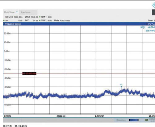
Band38-5MHz-16QAM-37775-1RB#0-Range3:3000~26500MHz
