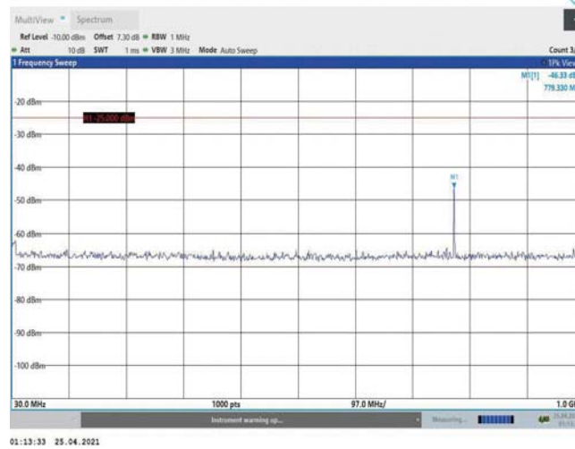
Band38-15MHz-QPSK-38000-1RB#0-Range1:30~1000MHz
