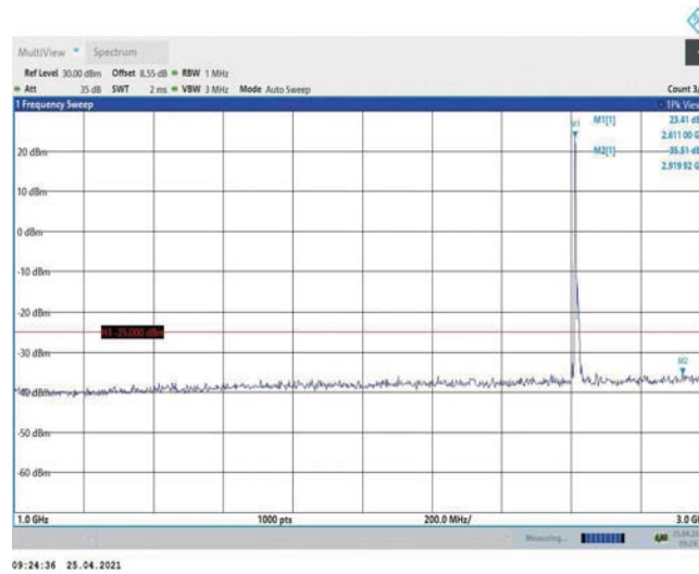
Band38-10MHz-QPSK-38200-1RB#0-Range2:1000~3000MHz
