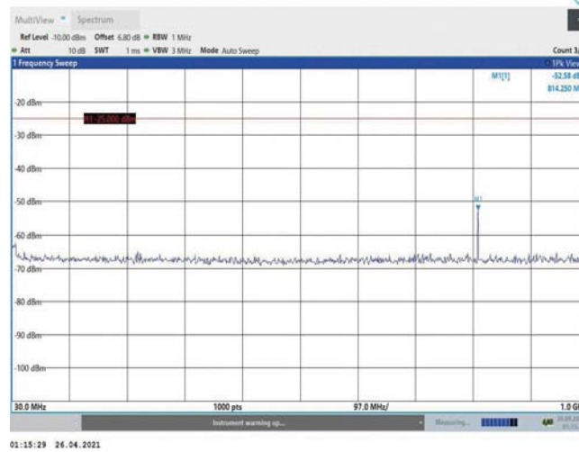
Band38-15MHz-QPSK-38175-1RB#0-Range1:30~1000MHz
