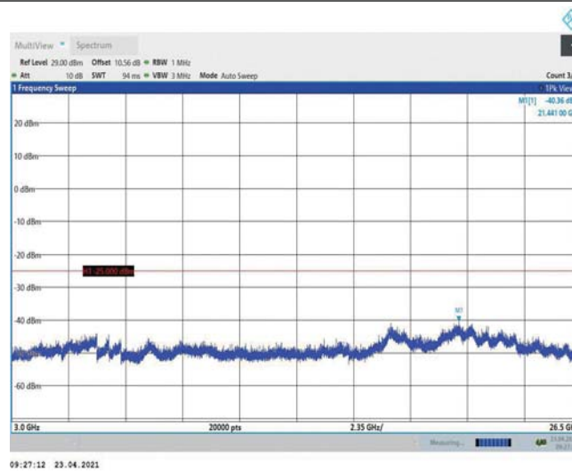
Band38-10MHz-QPSK-37800-1RB#0-Range3:3000~26500MHz
