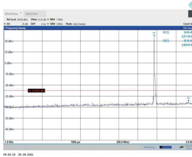
Band38-10MHz-16QAM-37800-1RB#0-Range2:1000~3000MHz
