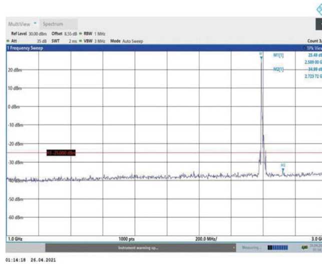
Band38-15MHz-QPSK-38000-1RB#0-Range2:1000~3000MHz
