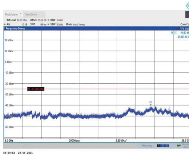
Band38-10MHz-QPSK-38200-1RB#0-Range3:3000~26500MHz
