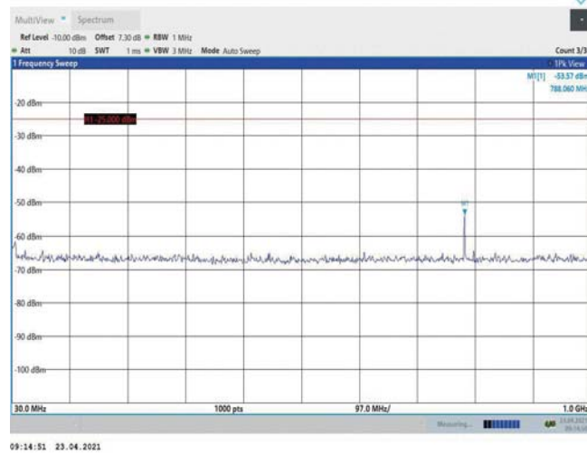
Band38-5MHz-QPSK-38000-1RB#0-Range1:30~1000MHz
