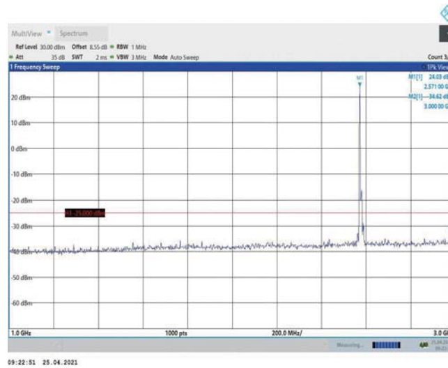
Band38-10MHz-QPSK-37800-1RB#0-Range2:1000~3000MHz
