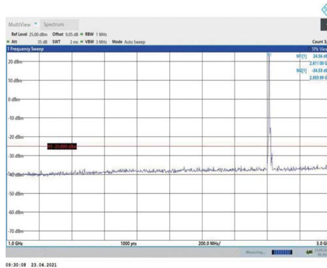
Band38-10MHz-16QAM-38200-1RB#0-Range2: 1000~3000MHz
