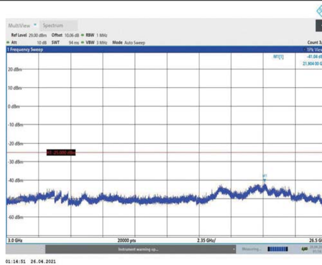
Band38-15MHz-16QAM-38000-1RB#0-Range3:3000~26500MHz
