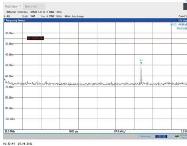
Band38-20MHz-QPSK-37850-1RB#0-Range1:30~1000MHz
