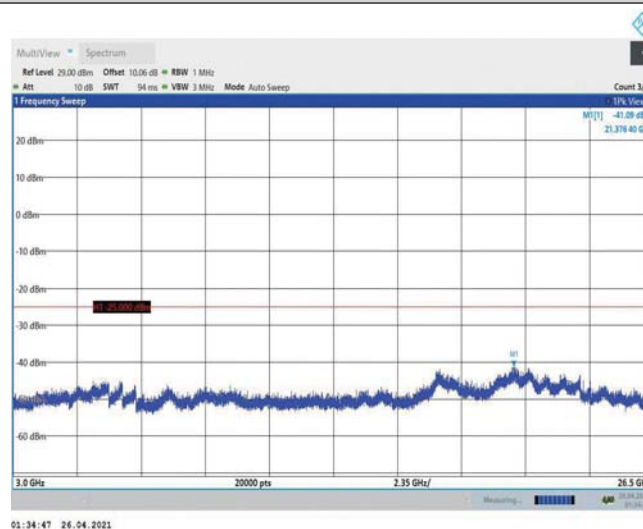
Band38-20MHz-QPSK-38000-1RB#0-Range3:3000~26500MHz
