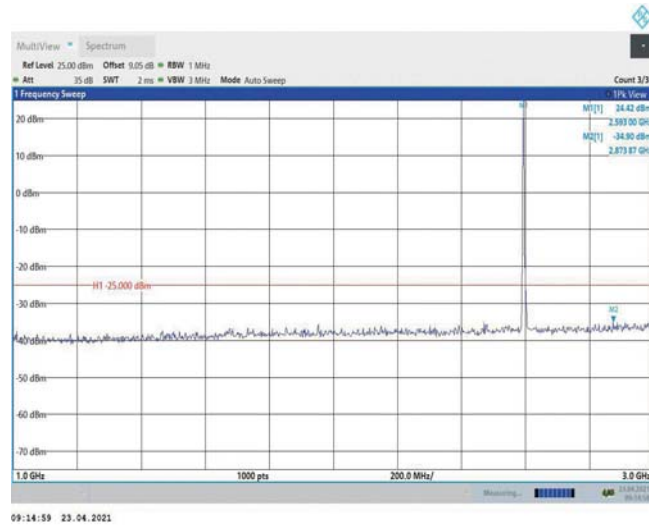
Band38-5MHz-QPSK-38000-1RB#0-Range2:1000~3000MHz
