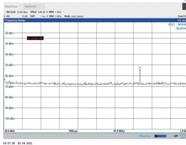
Band38-5MHz-16QAM-37775-1RB#0-Range1:30~1000MHz
