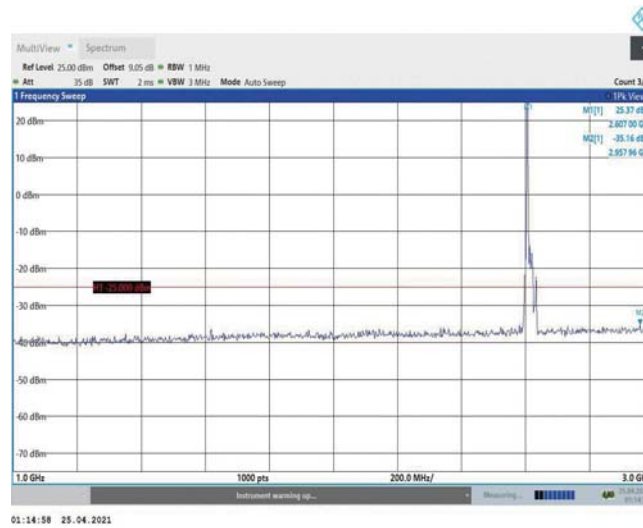
Band38-15MHz-QPSK-38175-1RB#0-Range2:1000~3000MHz
