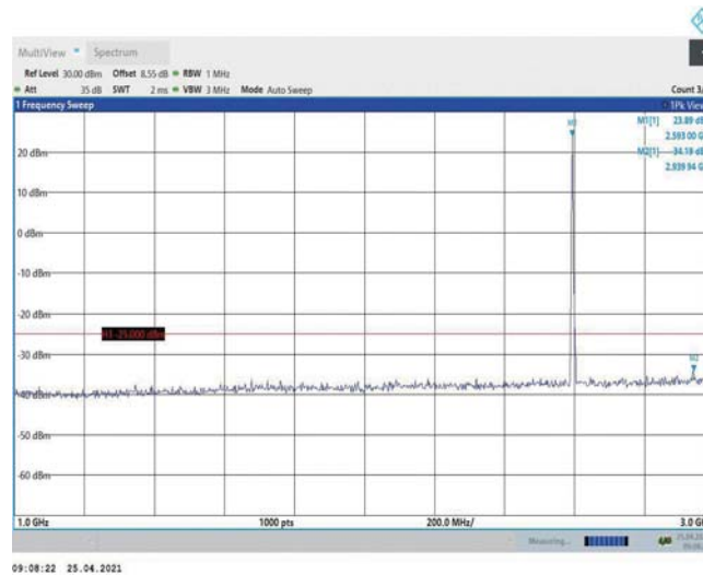
Band38-5MHz-QPSK-38000-1RB#0-Range2:1000~3000MHz
