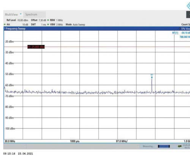
Band38-5MHz-16QAM-38000-1RB#0-Range1:30~1000MHz
