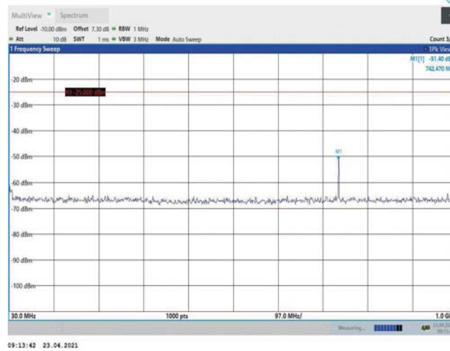
Band38-5MHz-QPSK-37775-1RB#0-Range1:30~1000MHz
