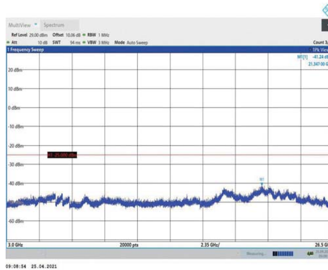
Band38-5MHz-16QAM-38000-1RB#0-Range3:3000~26500MHz
