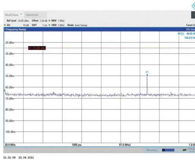
Band38-20MHz-QPSK-37850-1RB#0-Range1:30~1000MHz
