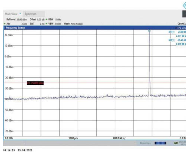
Band38-5MHz-16QAM-37775-1RB#0-Range2:1000~3000MHz
