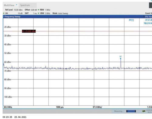
Band38-10MHz-QPSK-38000-1RB#0-Range1:30~1000MHz
