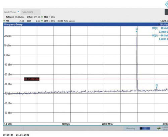
Band38-5MHz-16QAM-38000-1RB#0-Range2:1000~3000MHz
