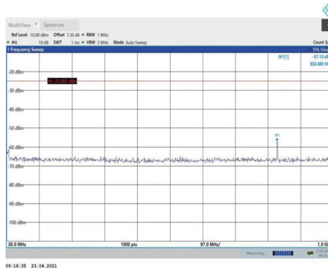
Band38-5MHz-16QAM-38225-1RB#0-Range1:30~1000MHz
