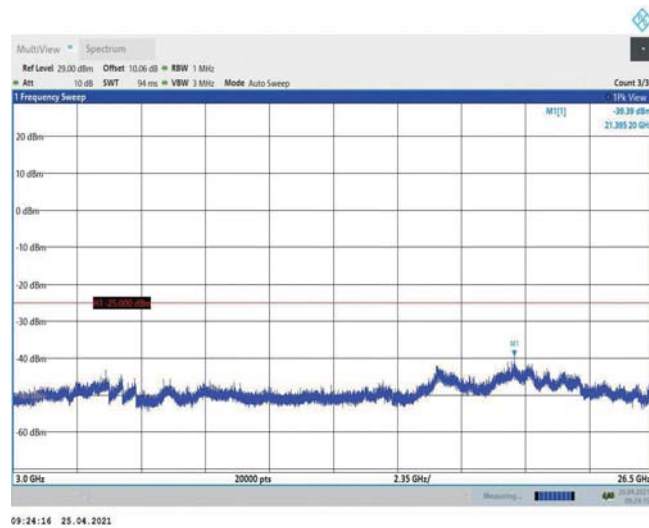
Band38-10MHz-16QAM-38000-1RB#0-Range3:3000~26500MHz
