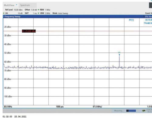
Band38-20MHz-QPSK-38000-1RB#0-Range1:30~1000MHz
