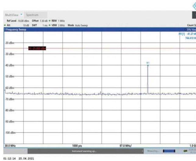
Band38-15MHz-QPSK-37825-1RB#0-Range1:30~1000MHz
