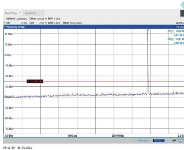
Band38-5MHz-QPSK-37775-1RB#0-Range2:1000~3000MHz
