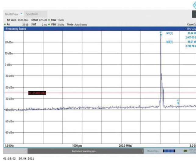
Band38-15MHz-16QAM-38175-1RB#0-Range2:1000~3000MHz
