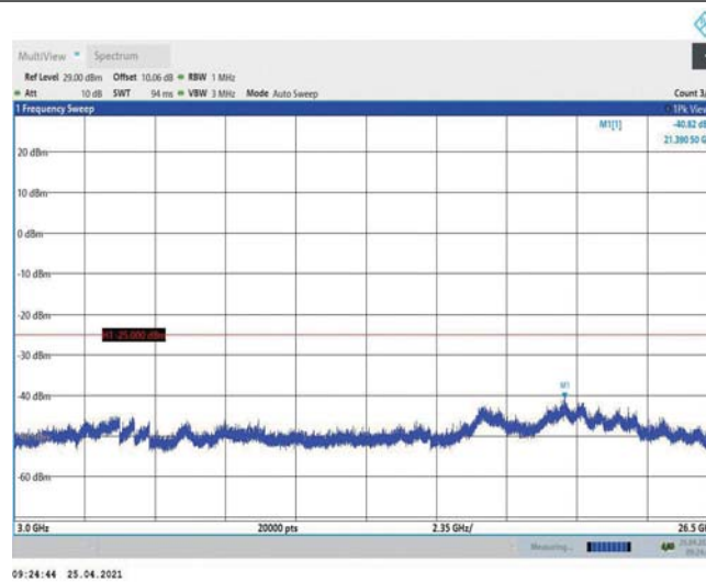
Band38-10MHz-QPSK-38200-1RB#0-Range3:3000~26500MHz
