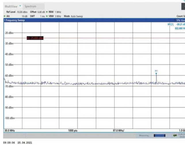
Band38-5MHz-QPSK-38225-1RB#0-Range1:30~1000MHz
