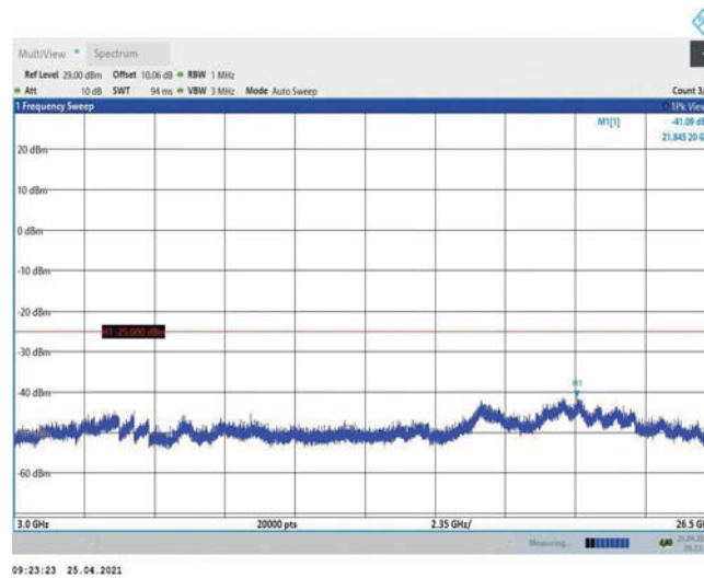
Band38-10MHz-16QAM-37800-1RB#0-Range3:3000~26500MHz
