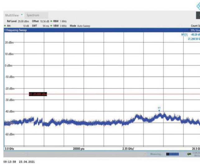
Band38-5MHz-QPSK-37775-1RB#0-Range3:3000~26500MHz
