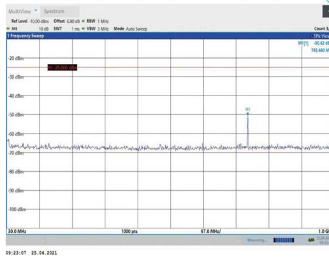
Band38-10MHz-16QAM-37800-1RB#0-Range1:30~1000MHz
