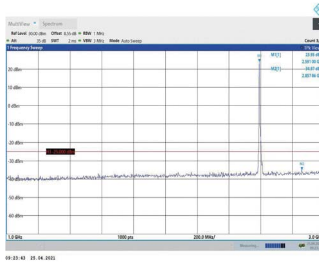
Band38-10MHz-QPSK-38000-1RB#0-Range2:1000~3000MHz
