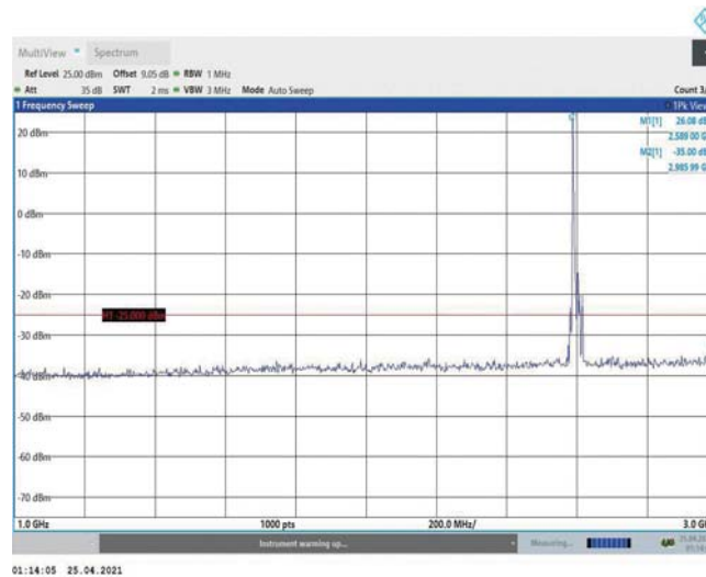
Band38-15MHz-16QAM-38000-1RB#0-Range2:1000~3000MHz
