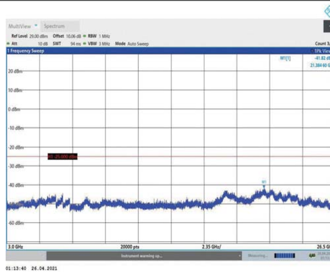
Band38-15MHz-16QAM-37825-1RB#0-Range3:3000~26500MHz
