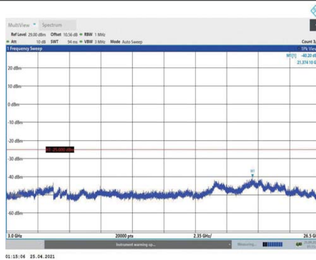
Band38-15MHz-QPSK-38175-1RB#0-Range3:3000~26500MHz
