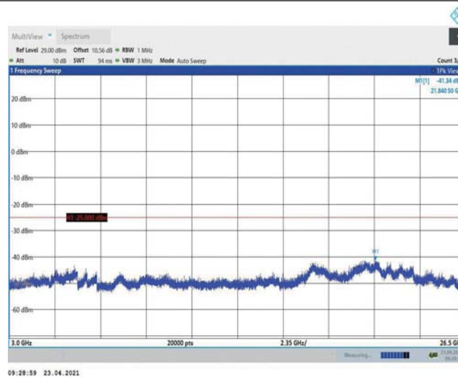
Band38-10MHz-16QAM-38000-1RB#0-Range3:3000~26500MHz
