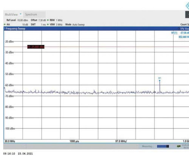
Band38-5MHz-QPSK-38225-1RB#0-Range1:30~1000MHz
