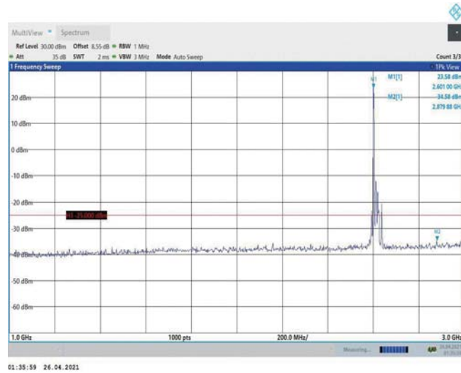
Band38-20MHz-16QAM-38150-1RB#0-Range2:1000~3000MHz
