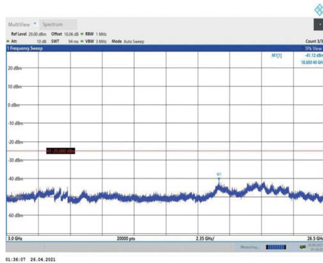
Band38-20MHz-16QAM-38150-1RB#0-Range3:3000~26500MHz
