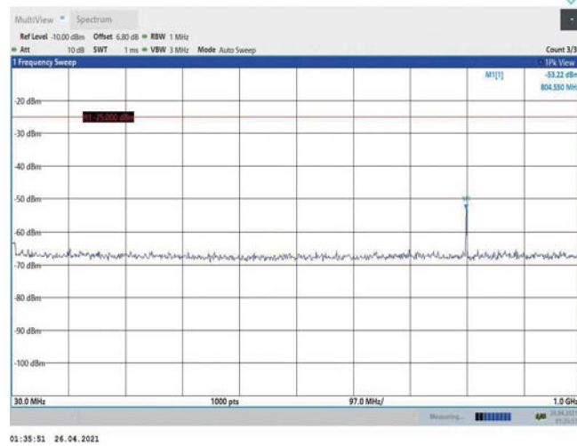
Band38-20MHz-16QAM-38150-1RB#0-Range1:30~1000MHz
